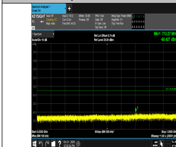
Band7-5MHz-16QAM-21100-1RB#24-30~1000-PASS
