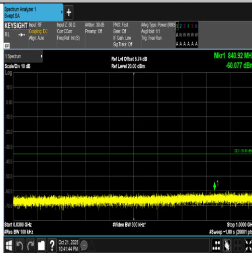
Band7-5MHz-16QAM-21425-1RB#24-30~1000-PASS
