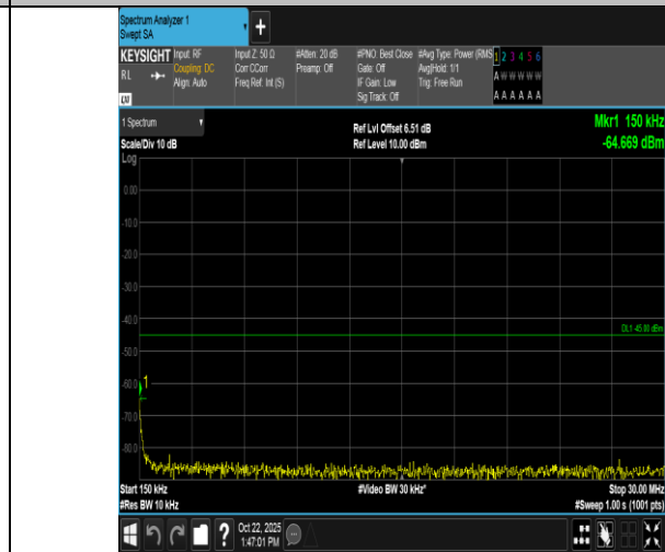
Band7-10MHz-QPSK-20800-50RB#0-0.15~30-PASS
