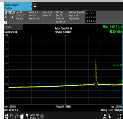
Band7-5MHz-QPSK-21100-25RB#0-1000~3000-PASS
