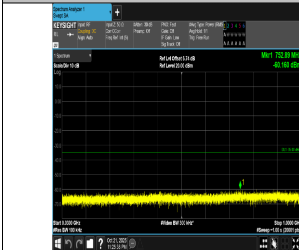
Band7-10MHz-QPSK-20800-1RB#0-30~1000-PASS
