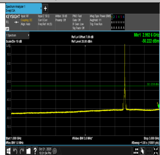
Band7-5MHz-16QAM-21100-1RB#0-1000~3000-PASS
