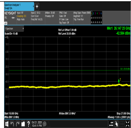
Band7-5MHz-QPSK-21425-1RB#24-18000~27000-PASS
