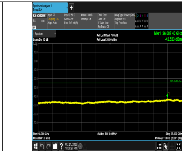
Band7-5MHz-QPSK-21425-1RB#0-18000~27000-PASS
