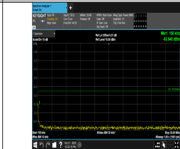
Band7-5MHz-16QAM-21100-1RB#24-0.15~30-PASS
