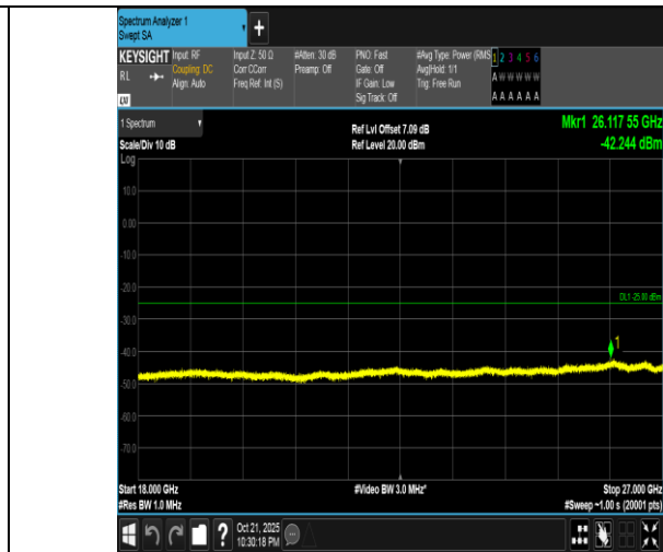
Band7-5MHz-QPSK-21100-1RB#0-18000~27000-PASS
