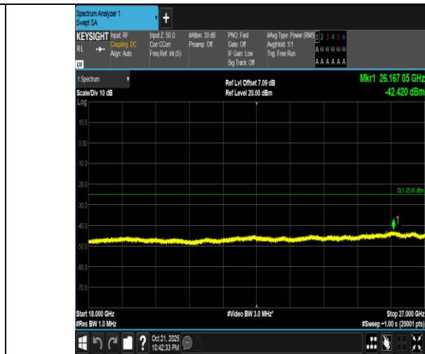
Band7-5MHz-16QAM-21425-1RB#24-18000~27000-PASS
