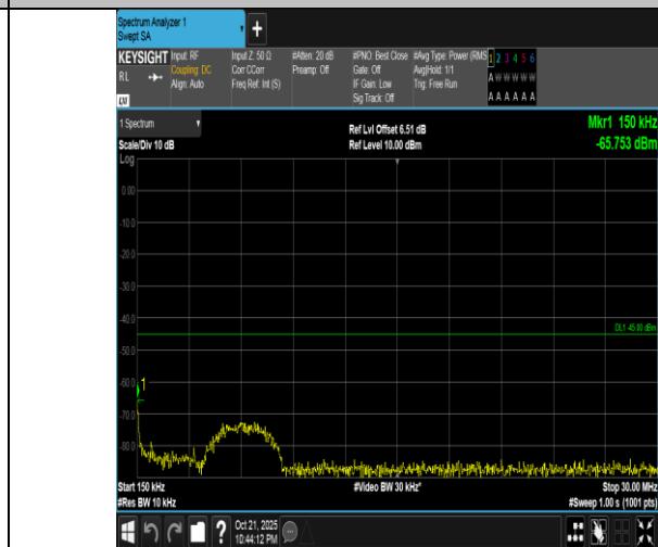
Band7-5MHz-16QAM-21425-25RB#0-0.15~30-PASS
