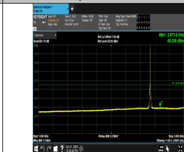
Band7-5MHz-16QAM-21100-1RB#24-1000~3000-PASS
