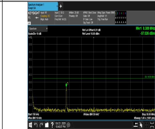
Band7-5MHz-QPSK-21425-1RB#24-0.15~30-PASS
