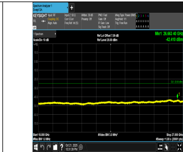
Band7-5MHz-16QAM-21100-1RB#0-18000~27000-PASS
