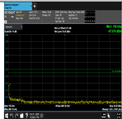
Band7-5MHz-16QAM-21100-25RB#0-0.15~30-PASS
