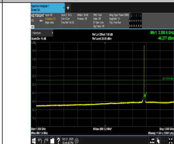
Band7-5MHz-16QAM-21425-25RB#0-1000~3000-PASS
