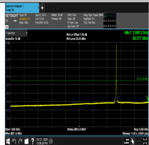
Band7-5MHz-16QAM-21100-25RB#0-1000~3000-PASS
