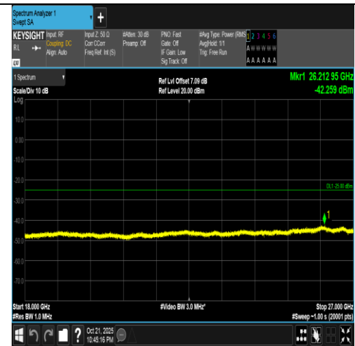
Band7-5MHz-16QAM-21425-25RB#0-18000~27000-PASS
