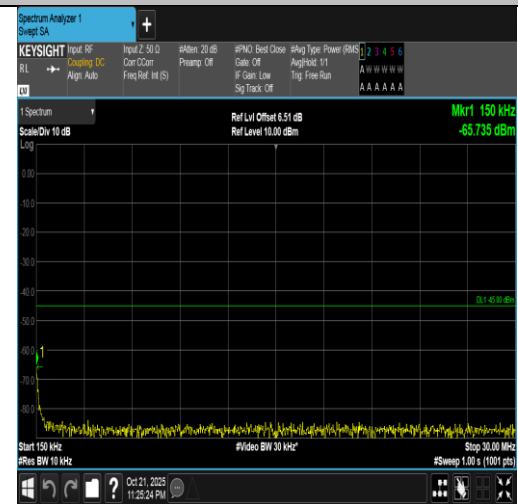
Band7-10MHz-QPSK-20800-1RB#0-0.15~30-PASS
