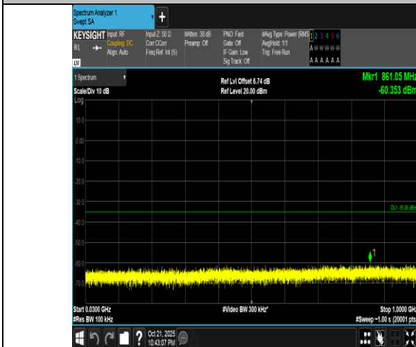
Band7-5MHz-QPSK-21425-25RB#0-30~1000-PASS
