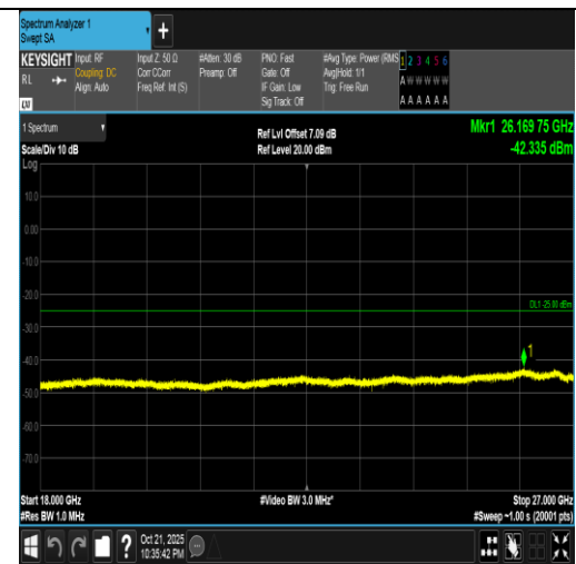
Band7-5MHz-QPSK-21100-25RB#0-18000~27000-PASS
