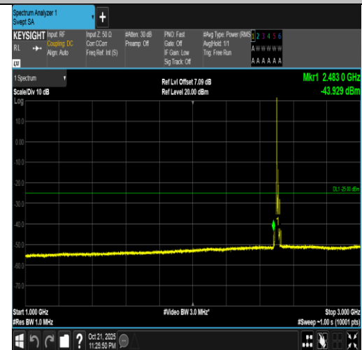
Band7-10MHz-QPSK-20800-1RB#0-1000~3000-PASS
