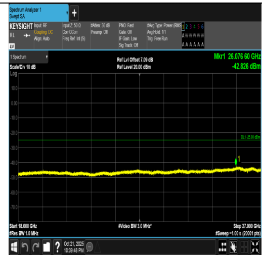
Band7-5MHz-16QAM-21425-1RB#0-18000~27000-PASS
