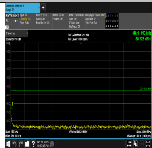
Band7-5MHz-16QAM-21100-1RB#0-0.15~30-PASS
