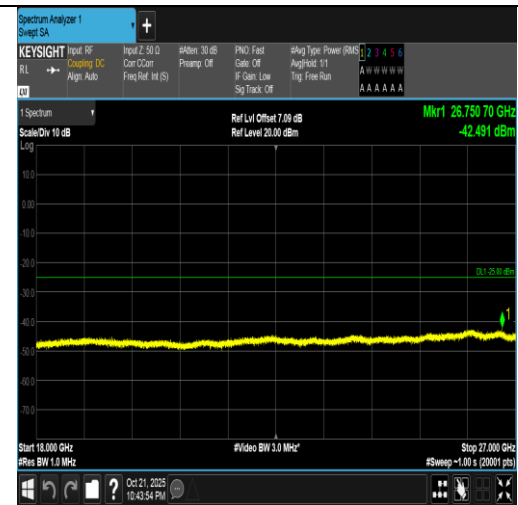
Band7-5MHz-QPSK-21425-25RB#0-18000~27000-PASS
