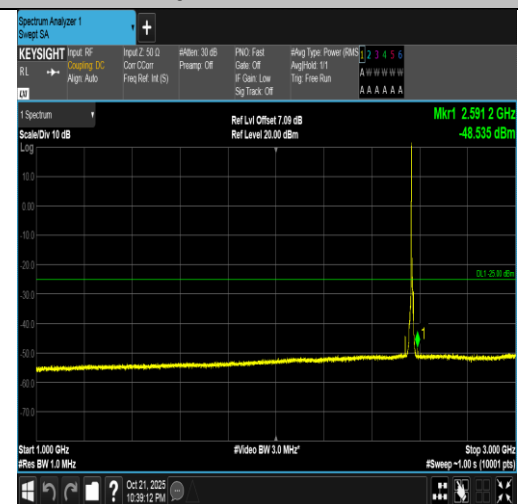
Band7-5MHz-16QAM-21425-1RB#0-1000~3000-PASS
