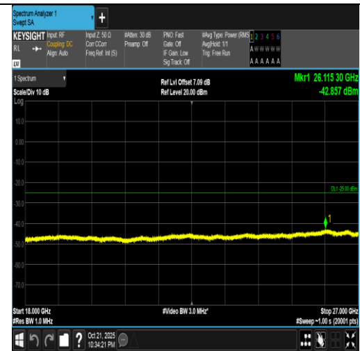
Band7-5MHz-16QAM-21100-1RB#24-18000~27000-PASS
