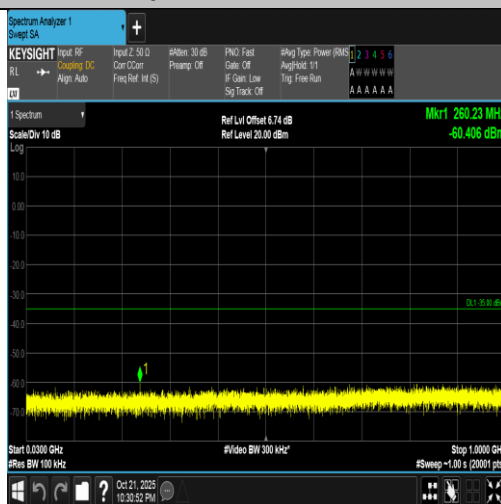
Band7-5MHz-16QAM-21100-1RB#0-30~1000-PASS
