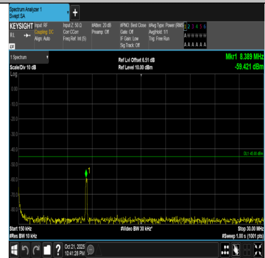
Band7-5MHz-16QAM-21425-1RB#24-0.15~30-PASS
