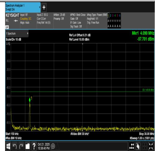
Band7-5MHz-16QAM-21425-1RB#0-0.15~30-PASS
