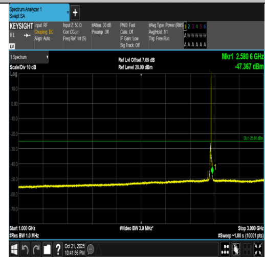
Band7-5MHz-16QAM-21425-1RB#24-1000~3000-PASS
