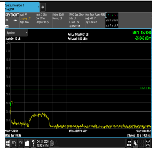
Band7-5MHz-QPSK-21425-25RB#0-0.15~30-PASS
