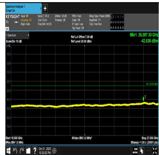
Band7-5MHz-QPSK-21100-1RB#24-18000~27000-PASS
