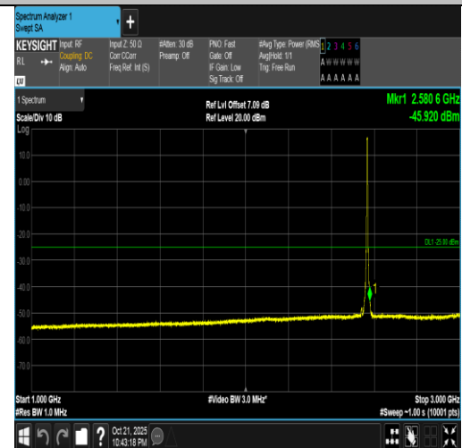
Band7-5MHz-QPSK-21425-25RB#0-1000~3000-PASS
