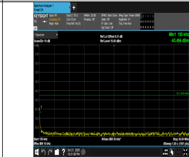
Band7-5MHz-QPSK-21100-1RB#24-0.15~30-PASS
