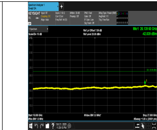
Band7-10MHz-QPSK-20800-1RB#49-18000~27000-PASS
