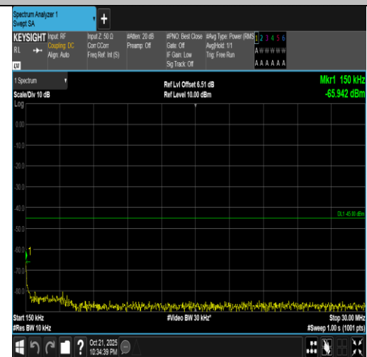
Band7-5MHz-QPSK-21100-25RB#0-0.15~30-PASS
