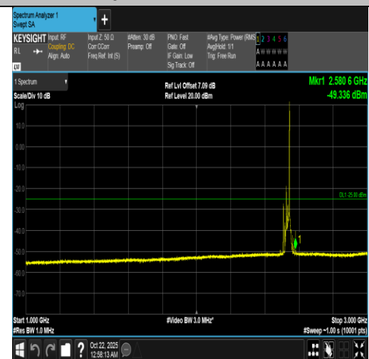
Band7-20MHz-QPSK-21100-1RB#99-1000~3000-PASS
