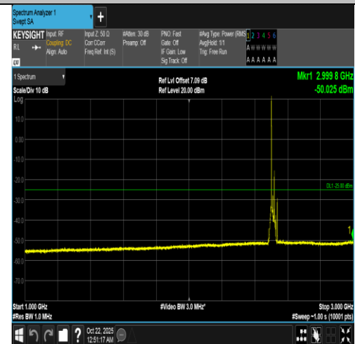
Band7-20MHz-16QAM-20850-1RB#0-1000~3000-PASS
