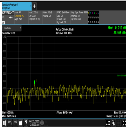
Band7-20MHz-QPSK-20850-1RB#99-0.009~0.15-PASS
