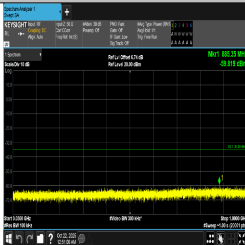
Band7-20MHz-16QAM-20850-1RB#0-30~1000-PASS
