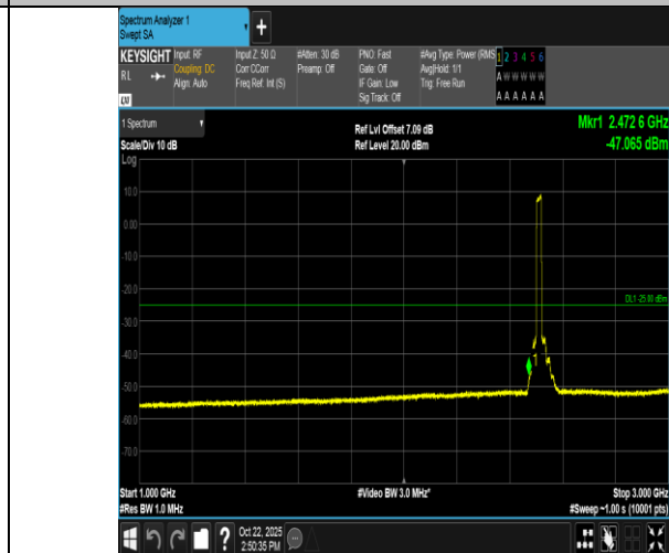
Band7-20MHz-QPSK-20850-100RB#0-1000~3000-PASS
