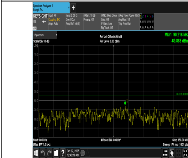
Band7-20MHz-QPSK-20850-1RB#0-0.009~0.15-PASS
