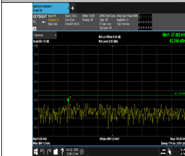
Band7-20MHz-16QAM-21100-1RB#0-0.009~0.15-PASS
