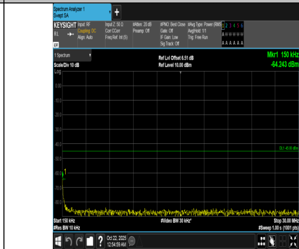
Band7-20MHz-QPSK-21100-1RB#0-0.15~30-PASS
