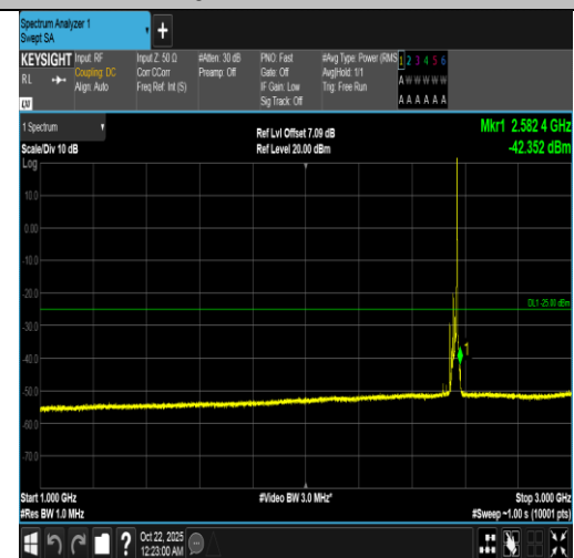
Band7-15MHz-16QAM-21375-1RB#74-1000~3000-PASS
