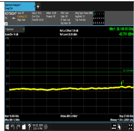
Band7-20MHz-QPSK-20850-100RB#0-18000~27000-PASS
