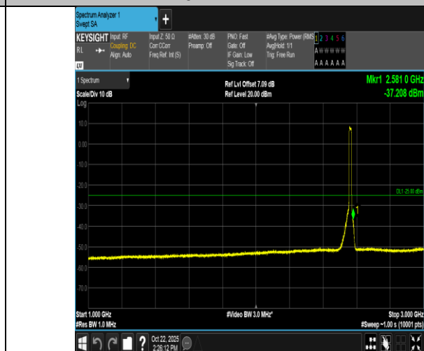
Band7-15MHz-16QAM-21375-75RB#0-1000~3000-PASS
