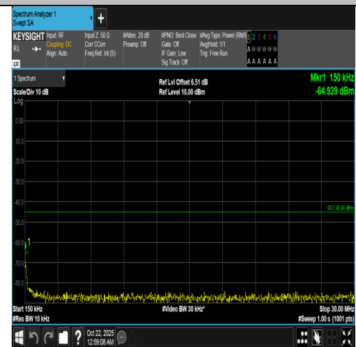
Band7-20MHz-16QAM-21100-1RB#99-0.15~30-PASS
