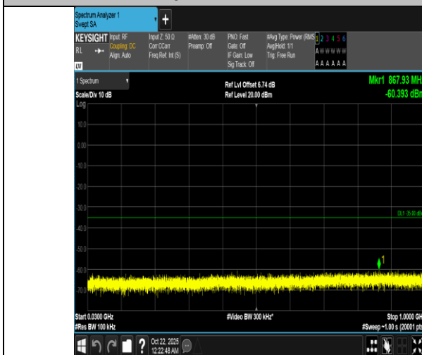
Band7-15MHz-16QAM-21375-1RB#74-30~1000-PASS
