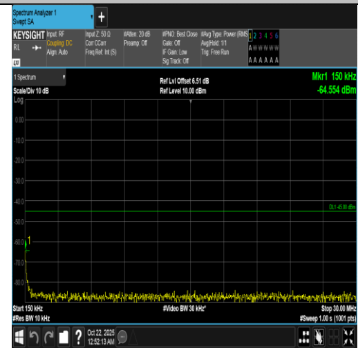
Band7-20MHz-QPSK-20850-1RB#99-0.15~30-PASS
