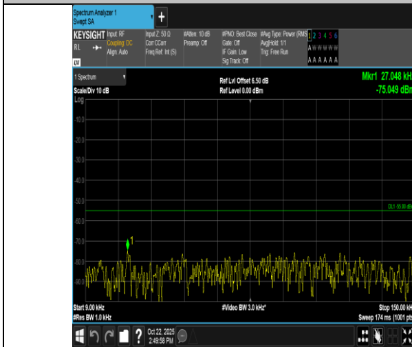
Band7-20MHz-QPSK-20850-100RB#0-0.009~0.15-PASS
