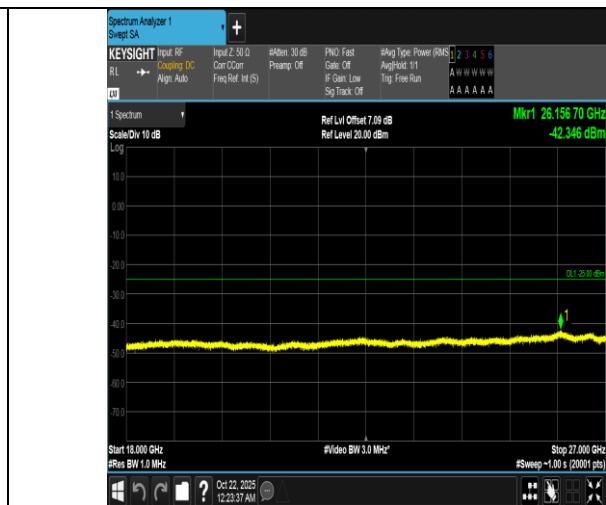
Band7-15MHz-16QAM-21375-1RB#74-18000~27000-PASS
