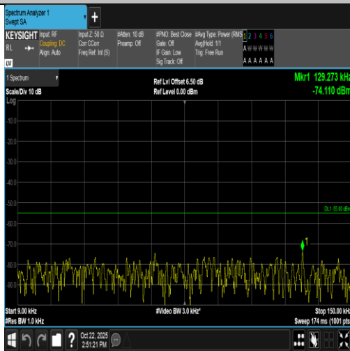
Band7-20MHz-16QAM-20850-100RB#0-0.009~0.15-PASS
