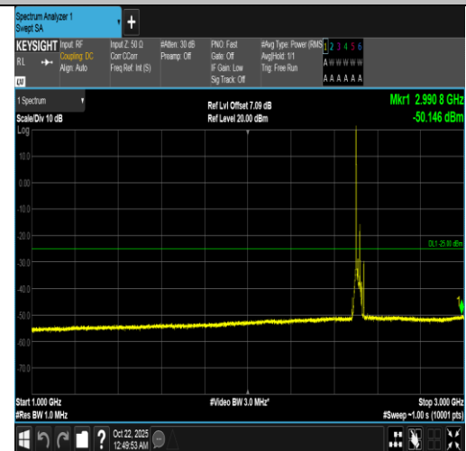
Band7-20MHz-QPSK-20850-1RB#0-1000~3000-PASS
