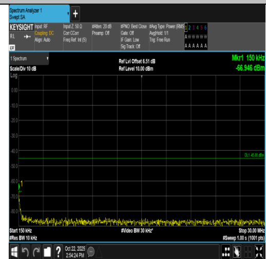
Band7-20MHz-16QAM-21100-100RB#0-0.15~30-PASS
