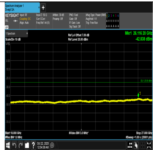
Band7-20MHz-16QAM-20850-1RB#99-18000~27000-PASS
