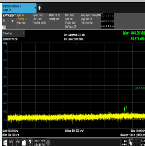
Band7-20MHz-16QAM-21100-100RB#0-30~1000-PASS
