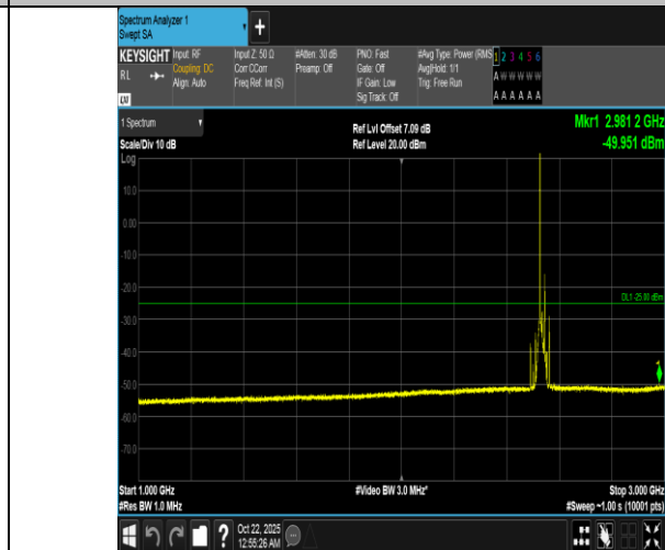
Band7-20MHz-QPSK-21100-1RB#0-1000~3000-PASS
