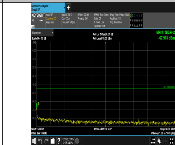
Band7-15MHz-16QAM-21375-75RB#0-0.15~30-PASS
