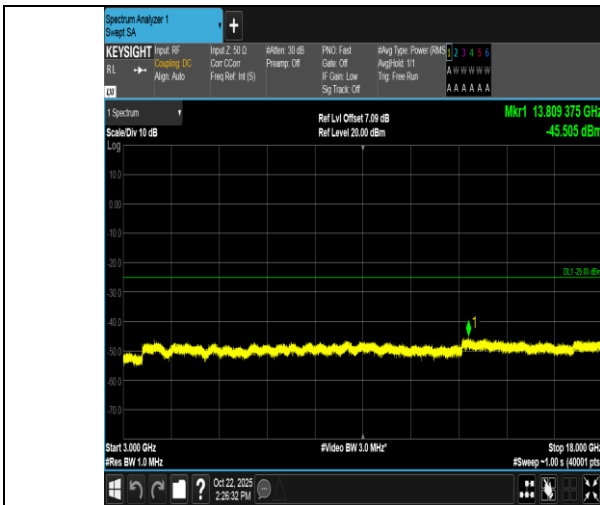
Band7-15MHz-16QAM-21375-75RB#0-3000~18000-PASS
