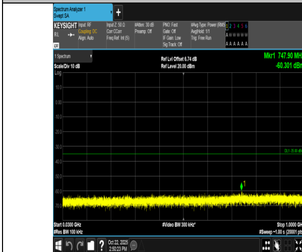
Band7-20MHz-QPSK-20850-100RB#0-30~1000-PASS
