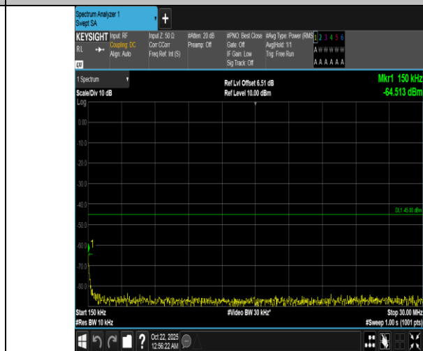
Band7-20MHz-16QAM-21100-1RB#0-0.15~30-PASS
