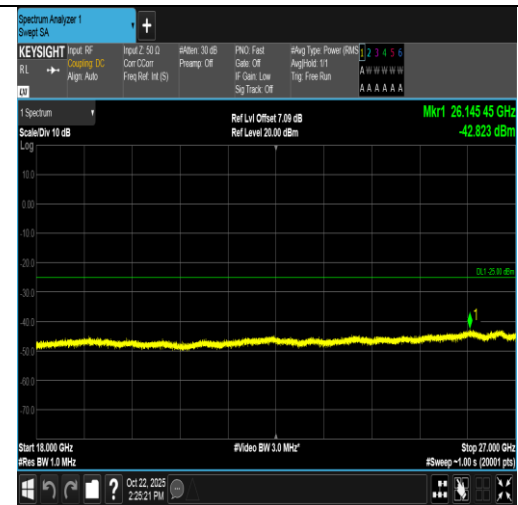
Band7-15MHz-QPSK-21375-75RB#0-18000~27000-PASS
