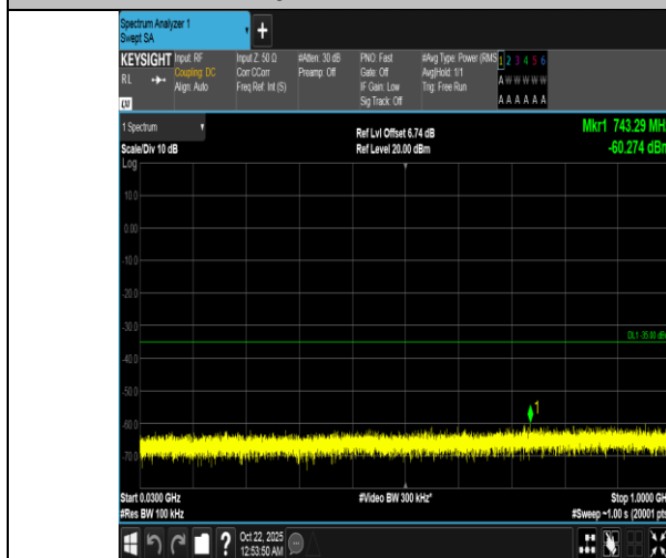
Band7-20MHz-16QAM-20850-1RB#99-30~1000-PASS
