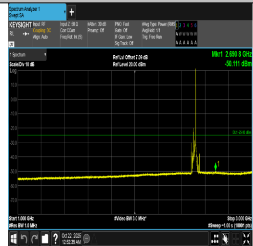
Band7-20MHz-QPSK-20850-1RB#99-1000~3000-PASS
