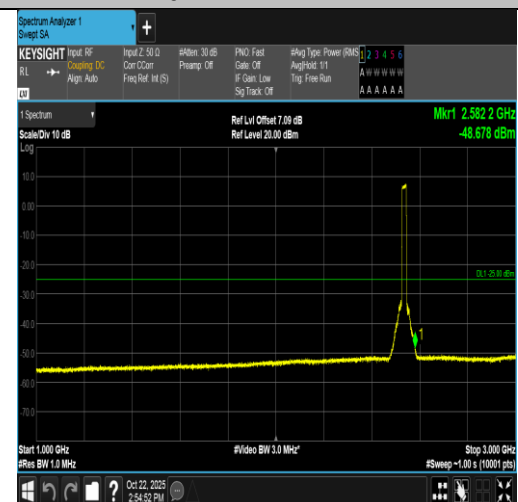
Band7-20MHz-16QAM-21100-100RB#0-1000~3000-PASS
