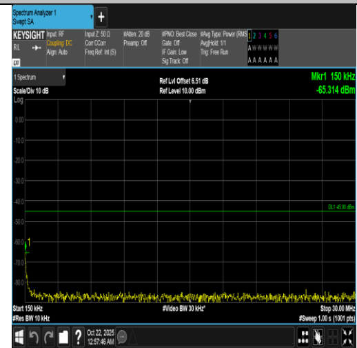
Band7-20MHz-QPSK-21100-1RB#99-0.15~30-PASS
