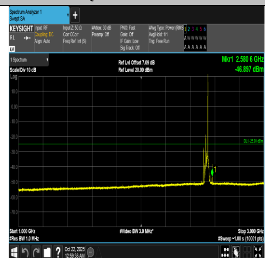
Band7-20MHz-16QAM-21100-1RB#99-1000~3000-PASS
