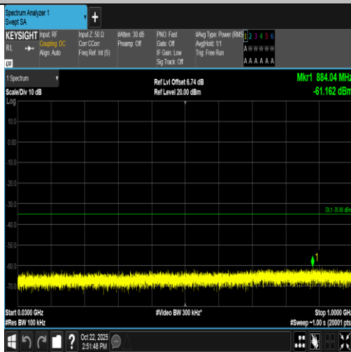
Band7-20MHz-16QAM-20850-100RB#0-30~1000-PASS
