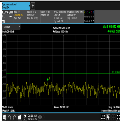
Band7-15MHz-16QAM-21375-1RB#0-0.009~0.15-PASS
