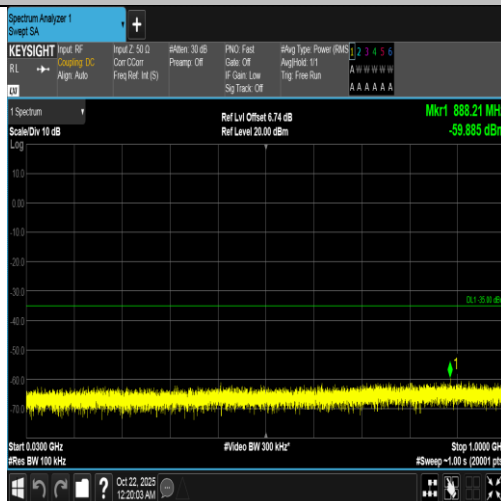
Band7-15MHz-16QAM-21375-1RB#0-30~1000-PASS
