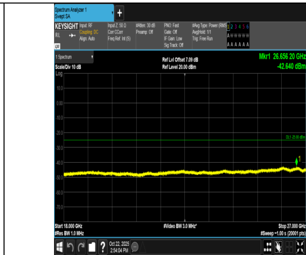
Band7-20MHz-QPSK-21100-100RB#0-18000~27000-PASS
