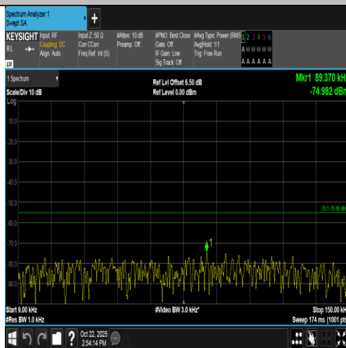
Band7-20MHz-16QAM-21100-100RB#0-0.009~0.15-PASS
