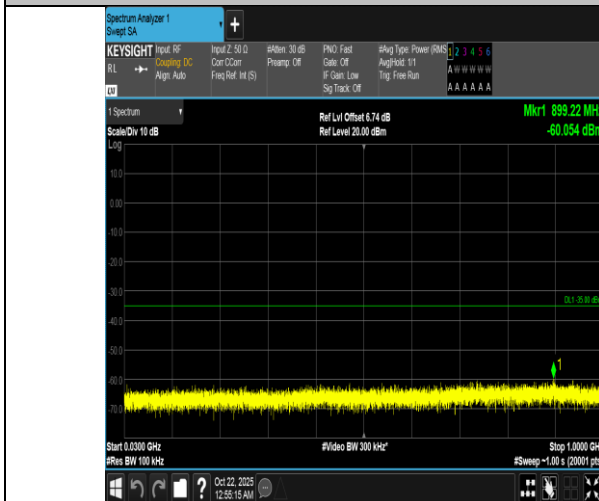
Band7-20MHz-QPSK-21100-1RB#0-30~1000-PASS
