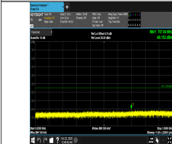
Band7-20MHz-QPSK-20850-1RB#0-30~1000-PASS
