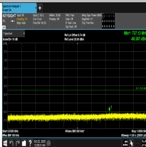
Band7-20MHz-QPSK-21100-1RB#99-30~1000-PASS
