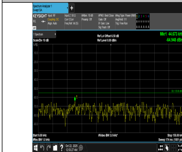
Band7-20MHz-16QAM-20850-1RB#99-0.009~0.15-PASS
