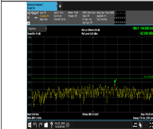
Band7-20MHz-QPSK-21100-1RB#0-0.009~0.15-PASS
