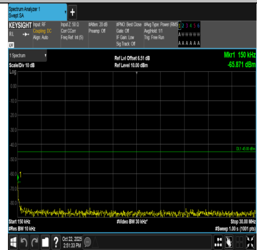
Band7-20MHz-16QAM-20850-100RB#0-0.15~30-PASS
