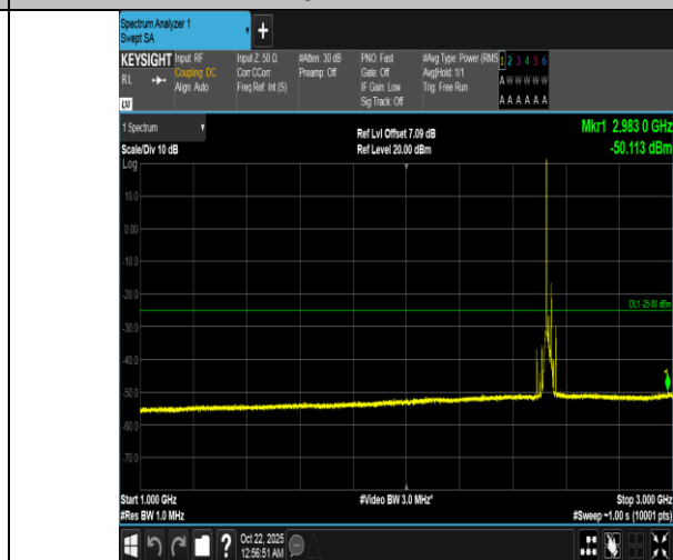
Band7-20MHz-16QAM-21100-1RB#0-1000~3000-PASS
