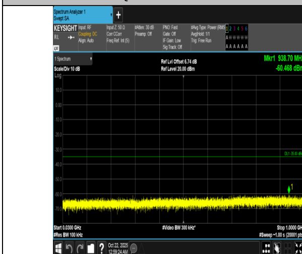
Band7-20MHz-16QAM-21100-1RB#99-30~1000-PASS
