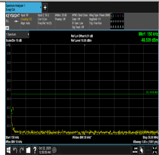
Band7-20MHz-16QAM-20850-1RB#0-0.15~30-PASS
