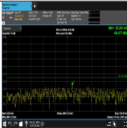
Band7-20MHz-QPSK-21100-1RB#99-0.009~0.15-PASS
