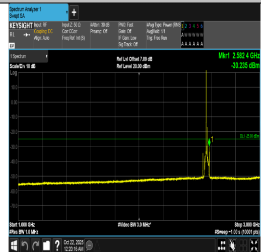
Band7-15MHz-16QAM-21375-1RB#0-1000~3000-PASS
