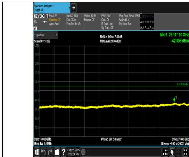
Band7-20MHz-16QAM-20850-100RB#0-18000~27000-PASS
