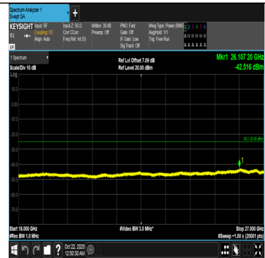
Band7-20MHz-QPSK-20850-1RB#0-18000~27000-PASS
