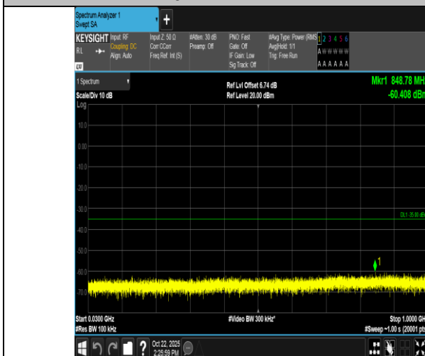
Band7-15MHz-16QAM-21375-75RB#0-30~1000-PASS
