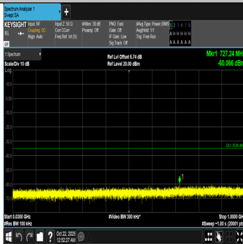
Band7-20MHz-QPSK-20850-1RB#99-30~1000-PASS
