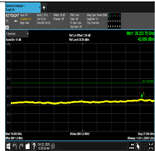
Band7-15MHz-16QAM-21375-1RB#0-18000~27000-PASS
