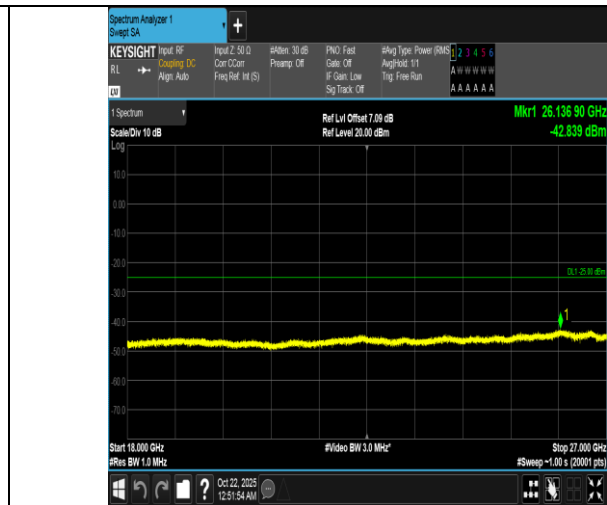
Band7-20MHz-16QAM-20850-1RB#0-18000~27000-PASS
