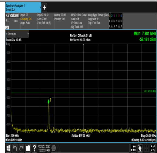
Band7-15MHz-16QAM-21375-1RB#74-0.15~30-PASS
