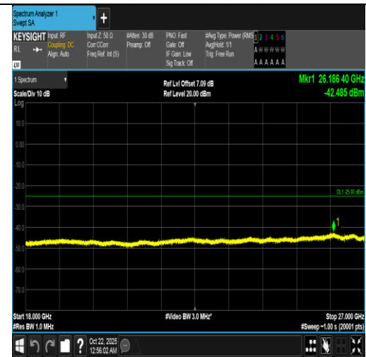
Band7-20MHz-QPSK-21100-1RB#0-18000~27000-PASS
