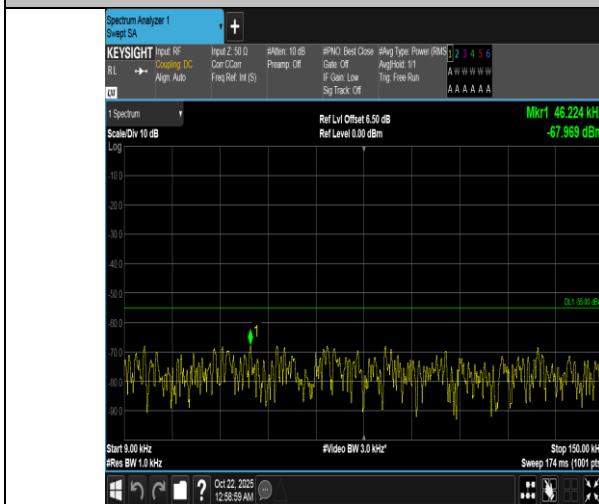
Band7-20MHz-16QAM-21100-1RB#99-0.009~0.15-PASS
