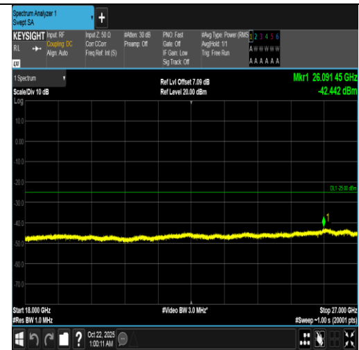
Band7-20MHz-16QAM-21100-1RB#99-18000~27000-PASS
