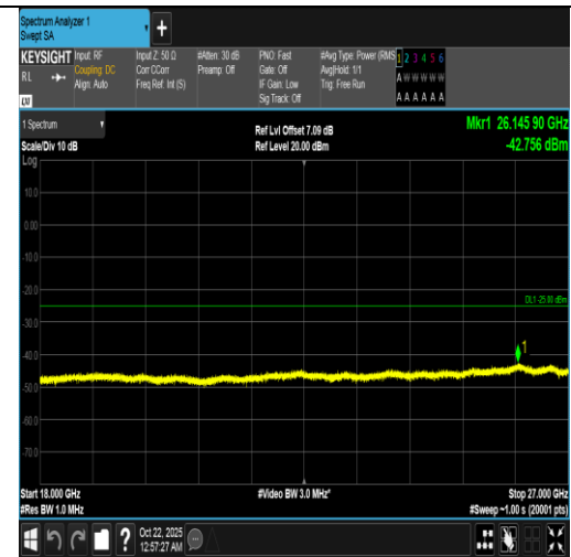
Band7-20MHz-16QAM-21100-1RB#0-18000~27000-PASS
