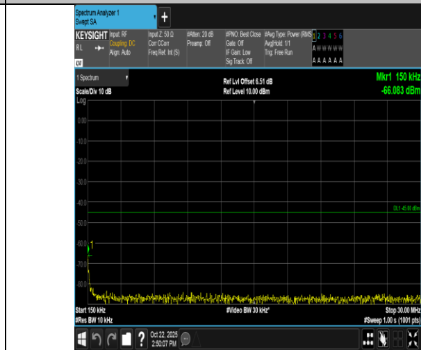
Band7-20MHz-QPSK-20850-100RB#0-0.15~30-PASS
