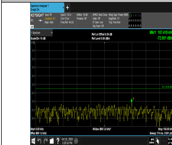
Band7-15MHz-16QAM-21375-75RB#0-0.009~0.15-PASS
