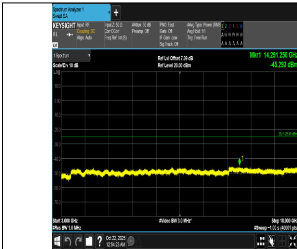
Band7-20MHz-16QAM-20850-1RB#99-3000~18000-PASS
