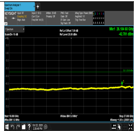
Band7-15MHz-16QAM-21375-75RB#0-18000~27000-PASS
