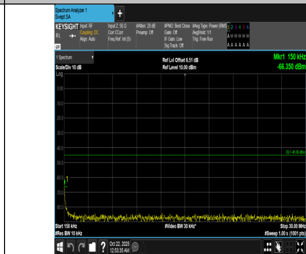
Band7-20MHz-16QAM-20850-1RB#99-0.15~30-PASS
