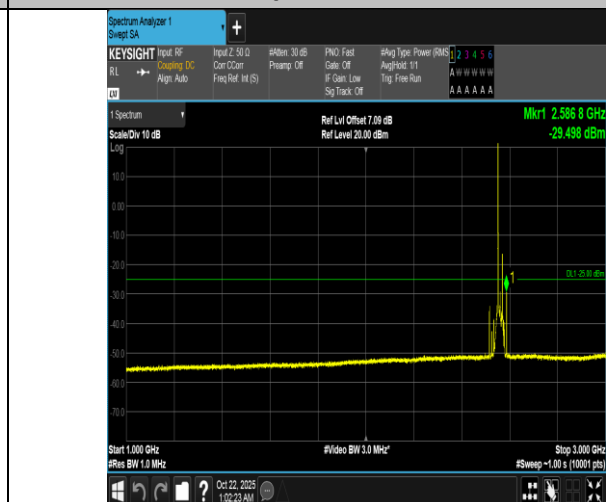
Band7-20MHz-16QAM-21350-1RB#0-1000~3000-PASS
