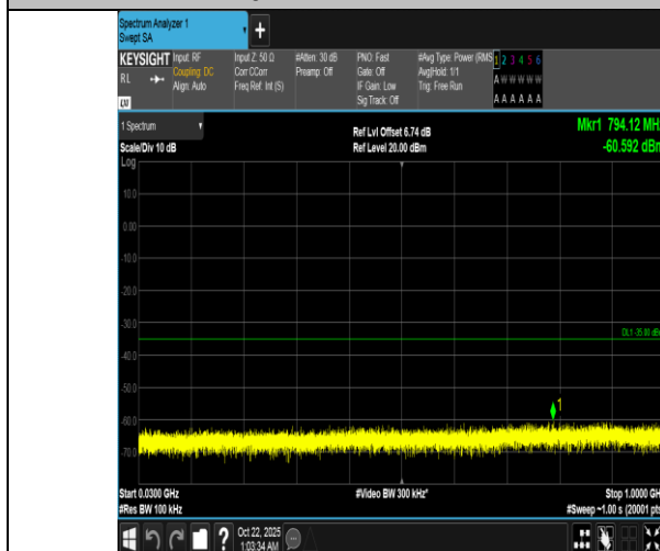
Band7-20MHz-QPSK-21350-1RB#99-30~1000-PASS
