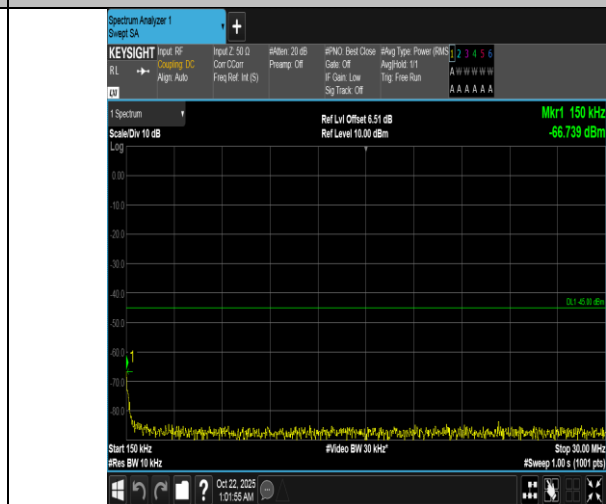
Band7-20MHz-16QAM-21350-1RB#0-0.15~30-PASS
