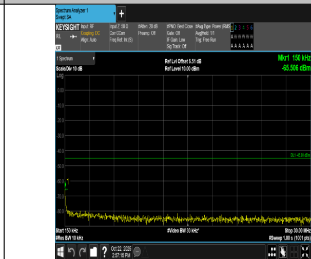
Band7-20MHz-16QAM-21350-100RB#0-0.15~30-PASS
