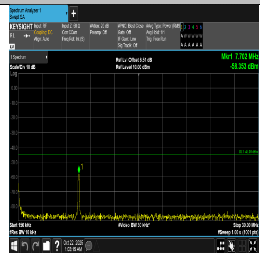
Band7-20MHz-QPSK-21350-1RB#99-0.15~30-PASS
