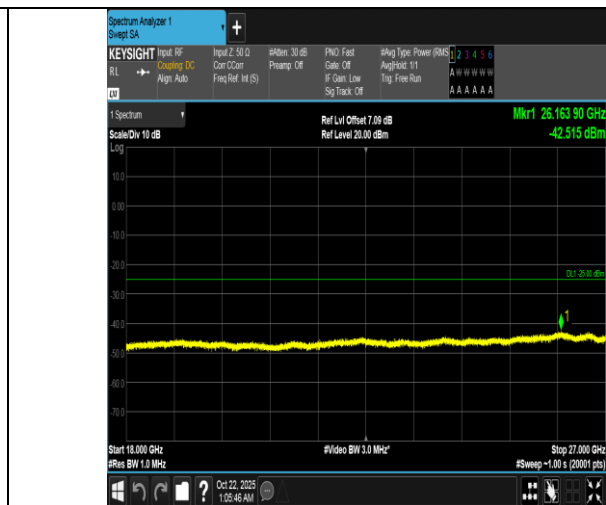
Band7-20MHz-16QAM-21350-1RB#99-18000~27000-PASS
