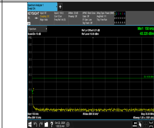
Band7-20MHz-QPSK-21350-1RB#0-0.15~30-PASS
