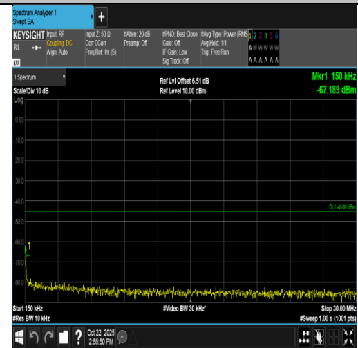
Band7-20MHz-QPSK-21350-100RB#0-0.15~30-PASS
