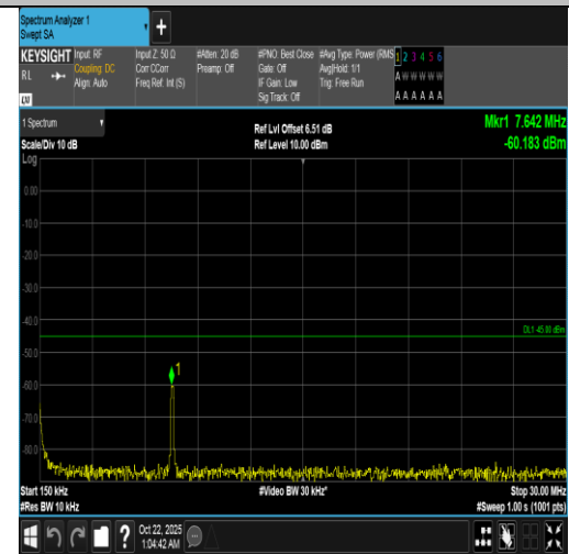
Band7-20MHz-16QAM-21350-1RB#99-0.15~30-PASS
