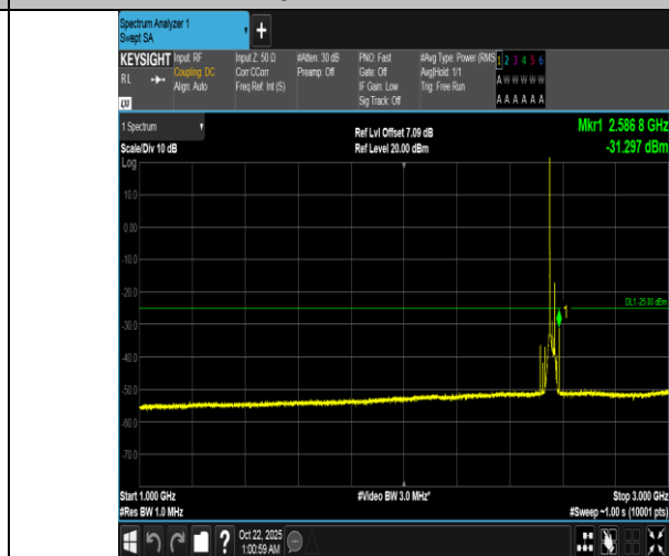
Band7-20MHz-QPSK-21350-1RB#0-1000~3000-PASS
