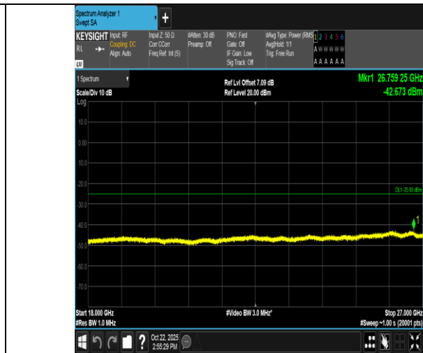
Band7-20MHz-16QAM-21100-100RB#0-18000~27000-PASS
