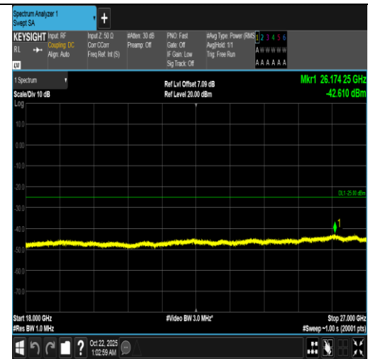
Band7-20MHz-16QAM-21350-1RB#0-18000~27000-PASS
