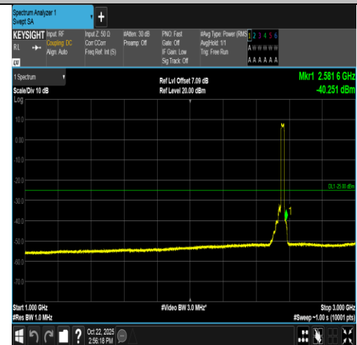
Band7-20MHz-QPSK-21350-100RB#0-1000~3000-PASS
