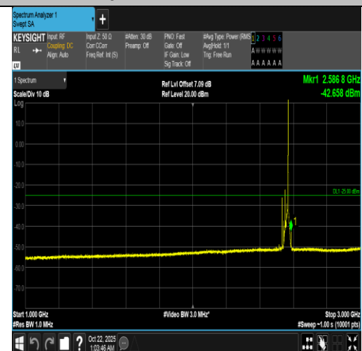
Band7-20MHz-QPSK-21350-1RB#99-1000~3000-PASS
