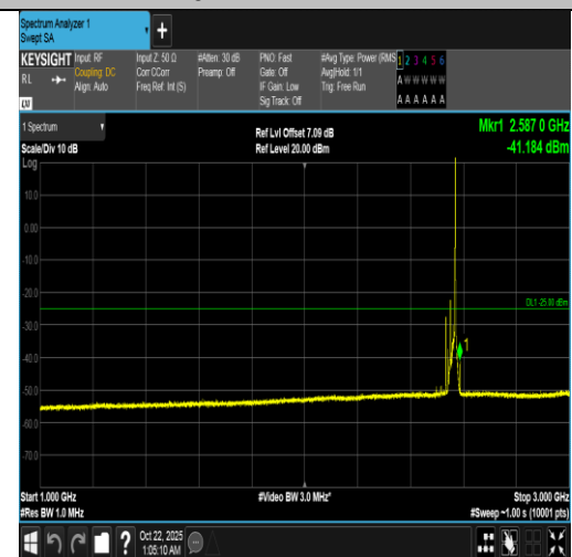
Band7-20MHz-16QAM-21350-1RB#99-1000~3000-PASS
