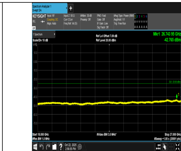
Band7-20MHz-QPSK-21350-100RB#0-18000~27000-PASS
