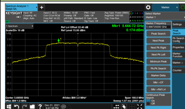
Channel 138 (5690MHz)
