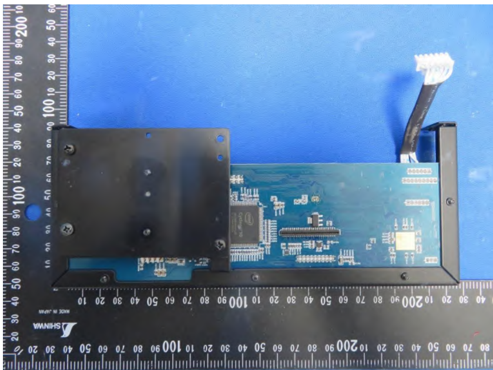
(42) EUT Photo
