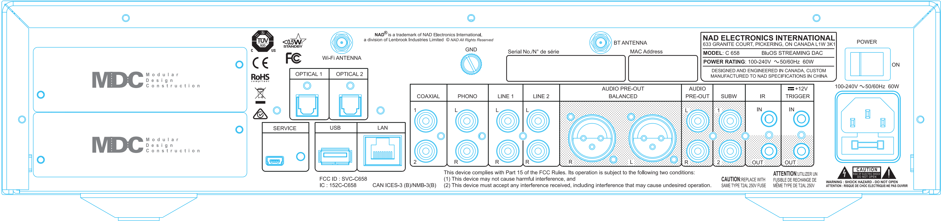
C 658 - Rear Panel
