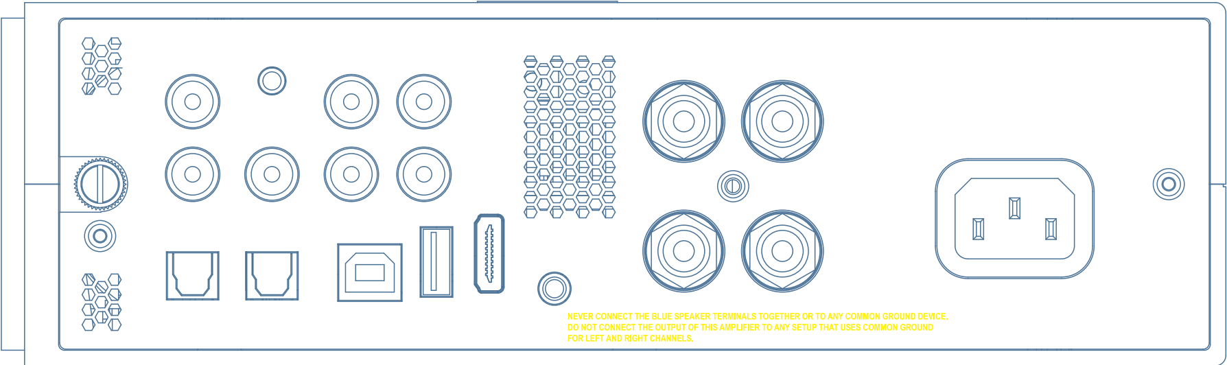
D 3045 Rear panel artwork - 2nd silkscreen printing: Pantone Process Yellow
