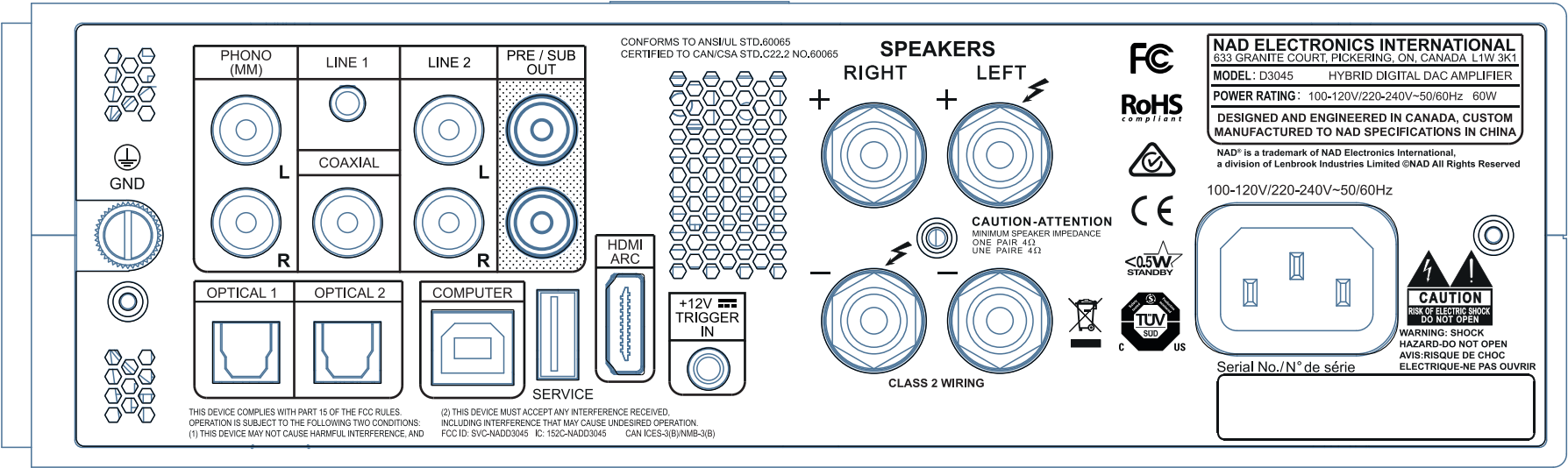
D 3045 Rear panel artwork - 1st silkscreen printing: Opaque white
