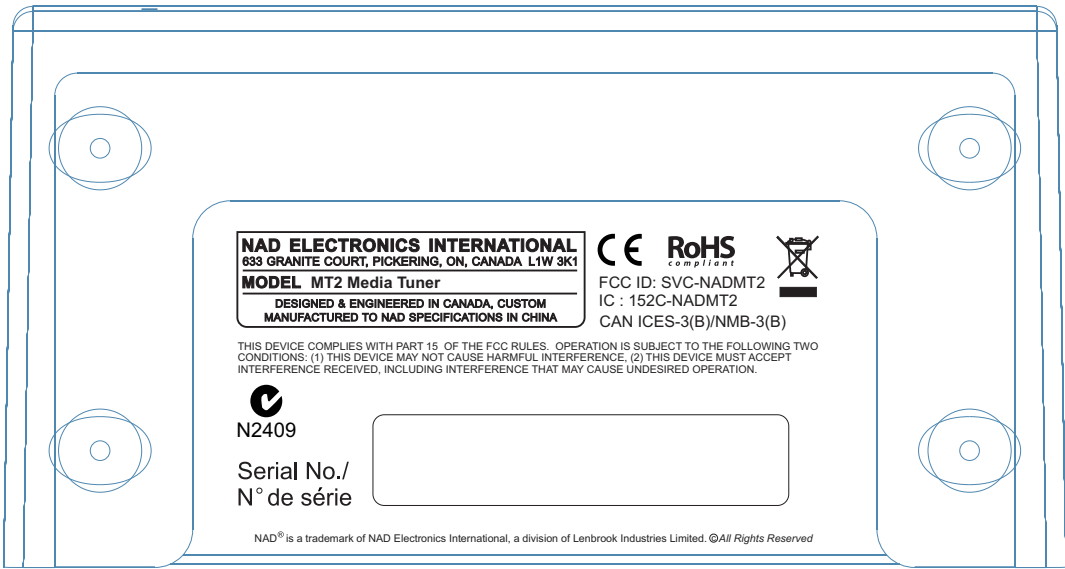
MT2 Bottom Panel
