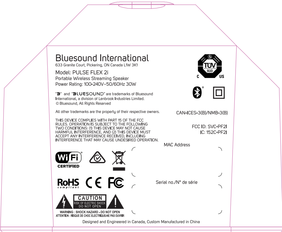
Pulse Flex 2i - Bottom panel silkscreen
