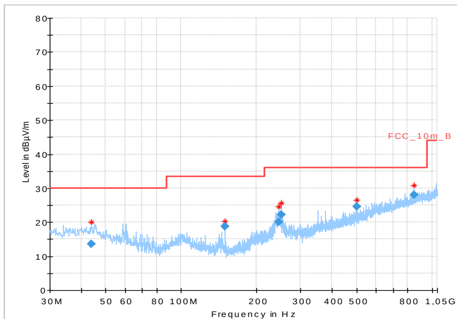
Plot 2: Low channel, 30 MHz to 1 GHz
