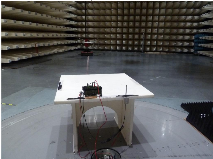
Photo 2 - Spurious Emissions 30MHz to 1 GHz EUT Set-up with external antenna:
