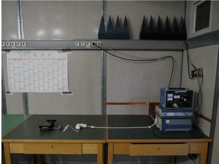
Photo 5 - AC Conducted Emissions EUT Set-up with internal antenna:
