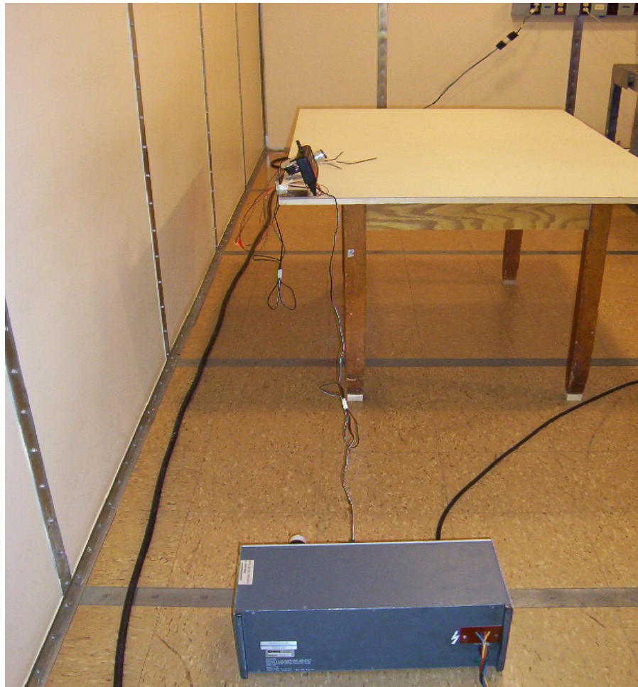
Conducted Emission Test Setup – Side View
