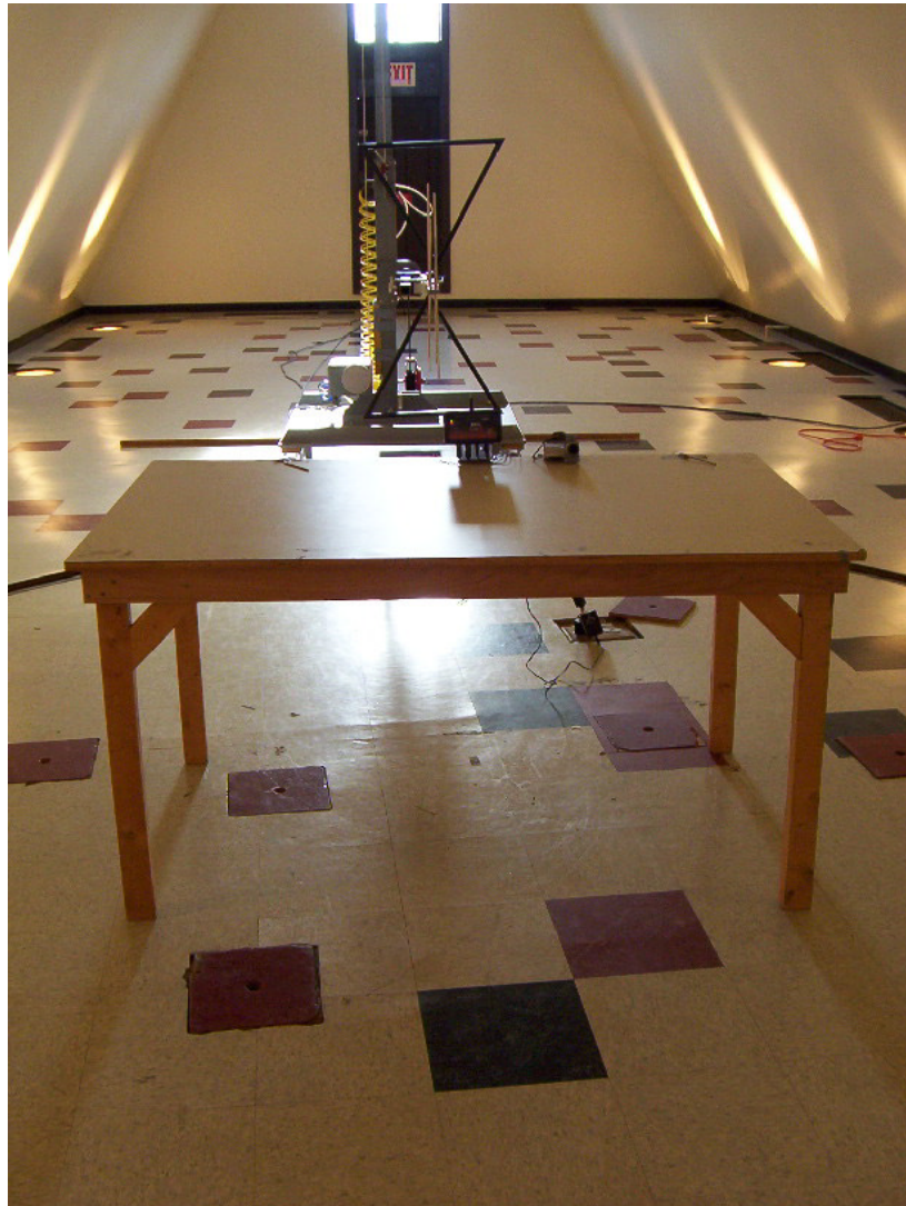
Radiated Emission Test Setup – Front View
