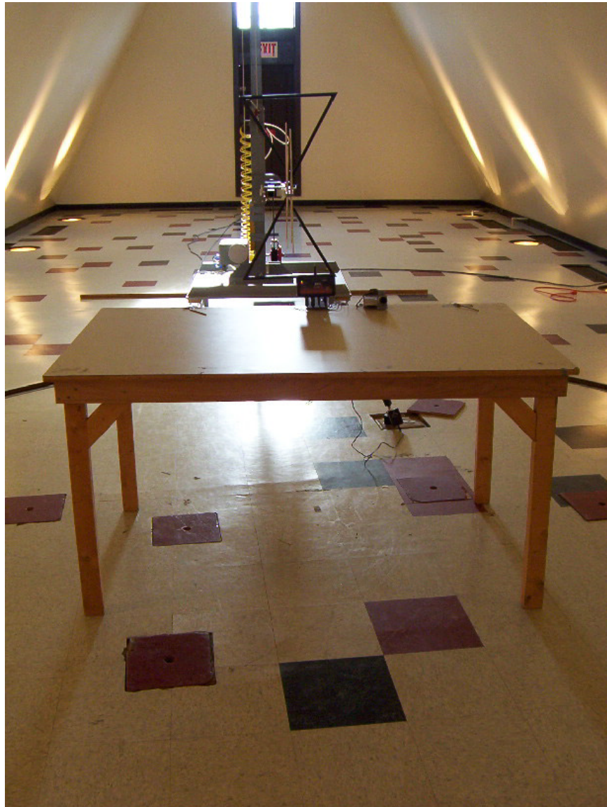
Radiated Emission Test Setup – Front View
