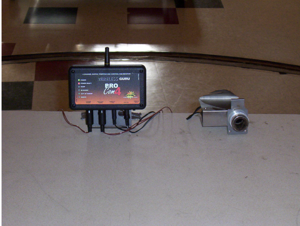
Radiated Emission Test Setup – Front Close up
