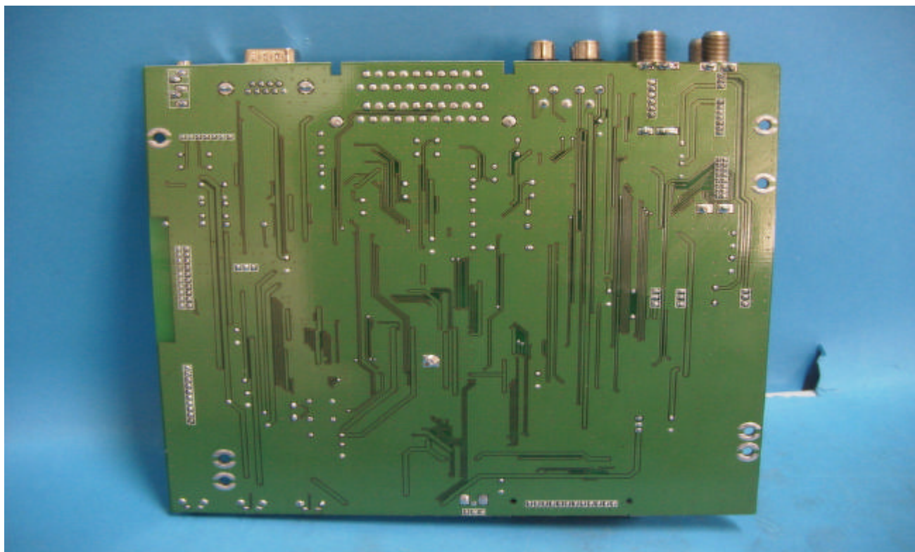
Main Board PCB Copper View
