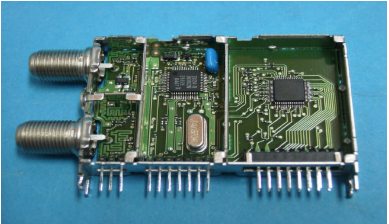
Inner Front View
