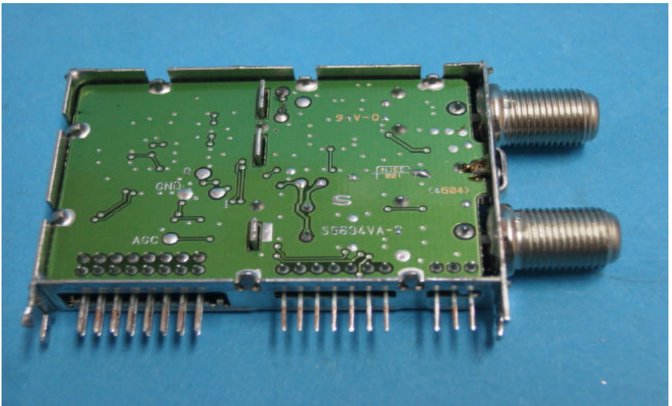
Inner Rear View
