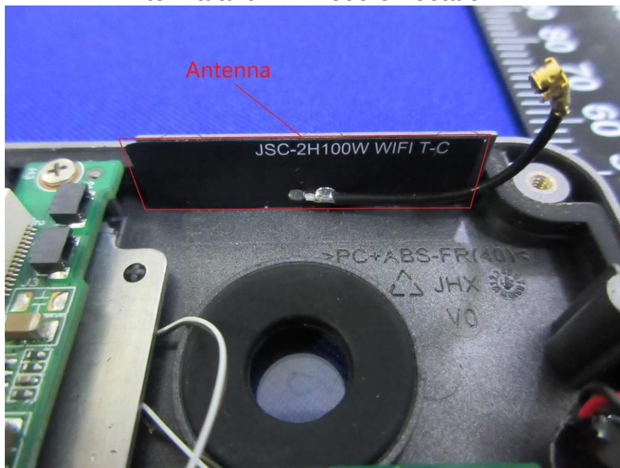
Antenna and RF Module Location-2
