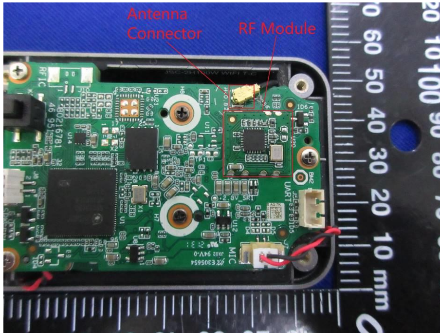
Antenna and RF Module Location-1
