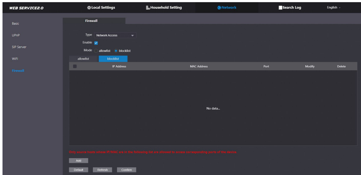
Figure 6-9 Firewall
