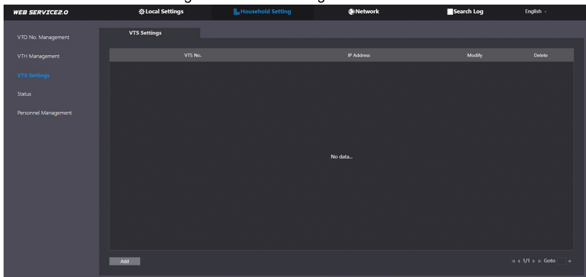
Figure 5-10 VTS management
