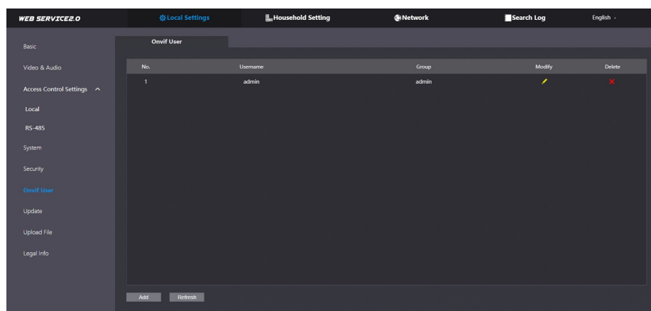
Figure 4-12 Onvif user
