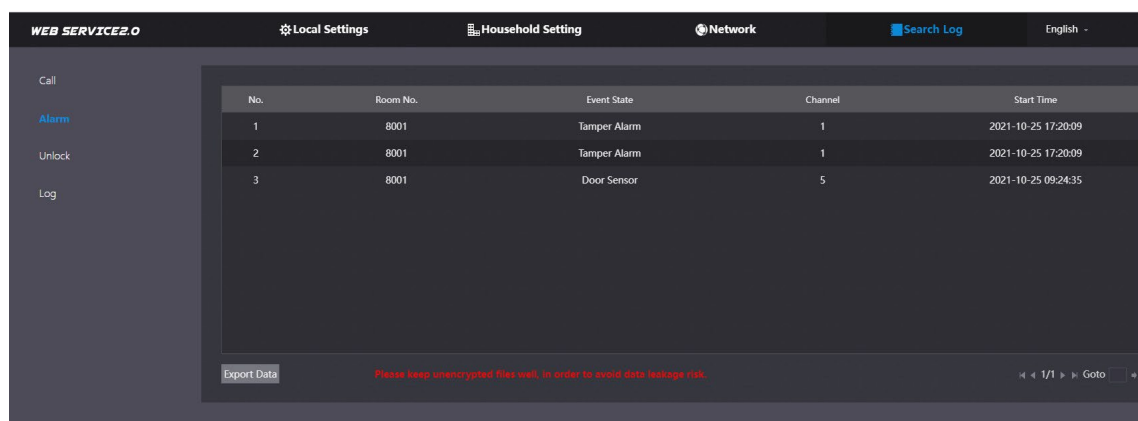
Figure 7-2 Alarm
