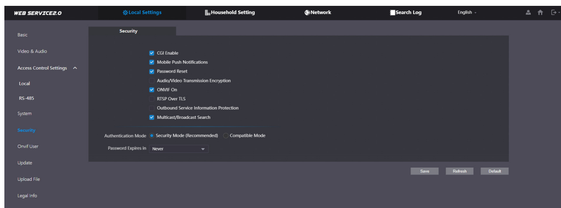
Figure 4-11 Security
