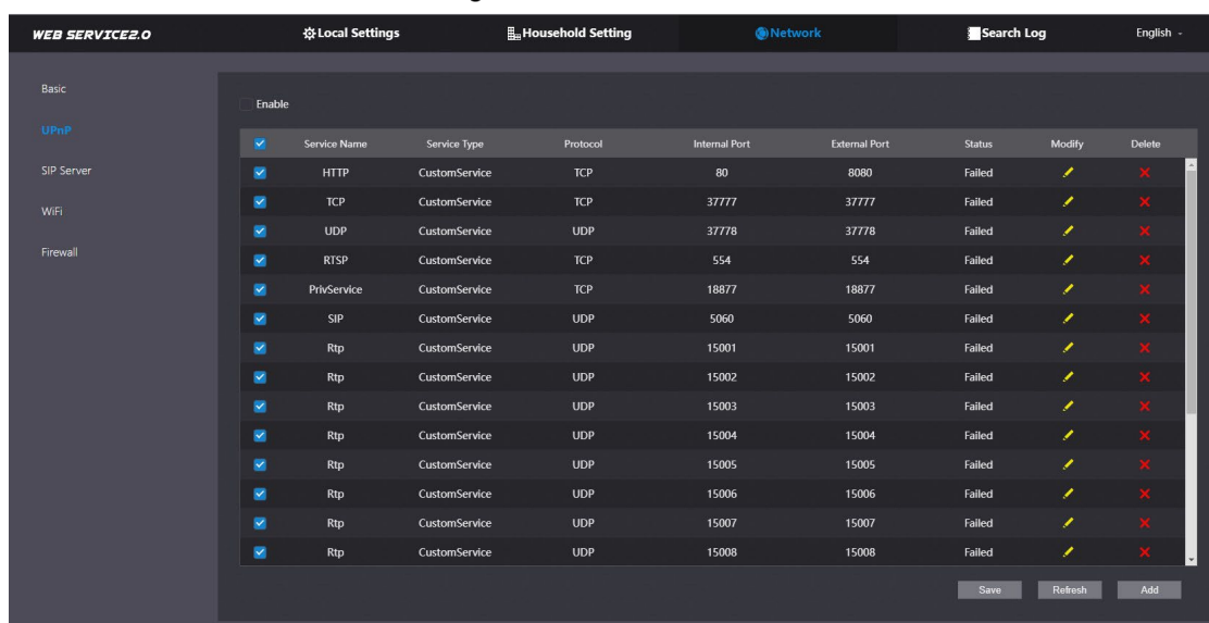
Figure 6-4 UPnP
