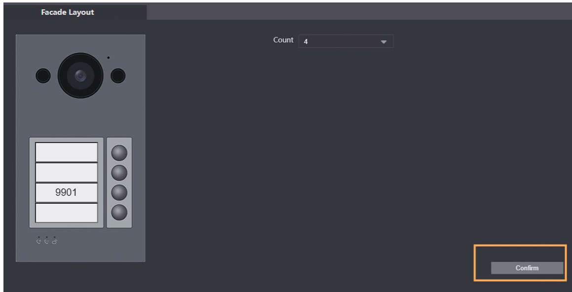
Figure 4-5 Confirm
