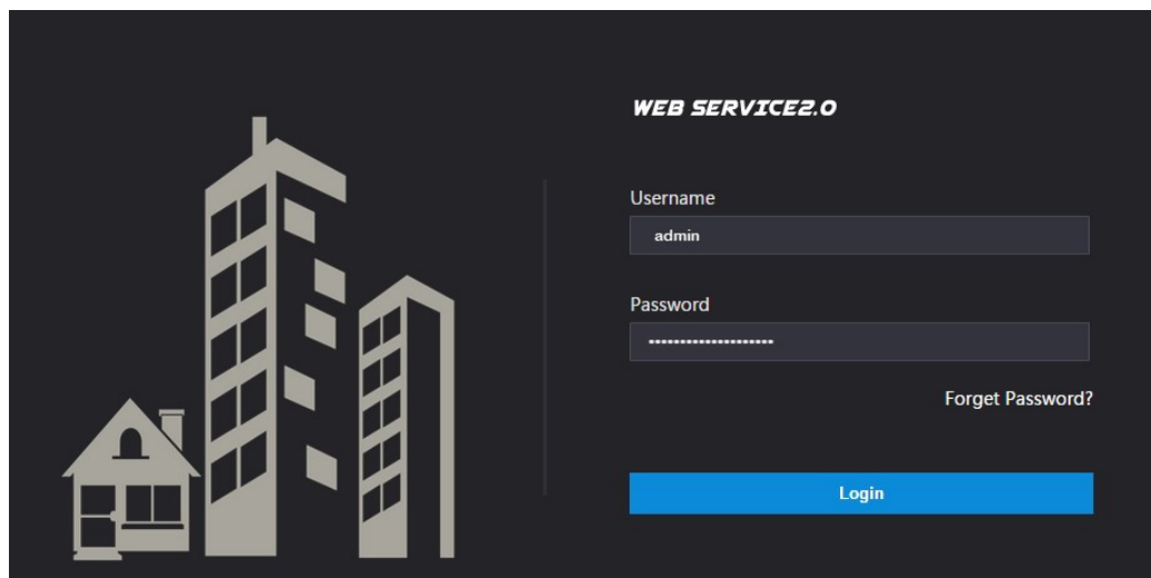
Figure 1-4 Login page
