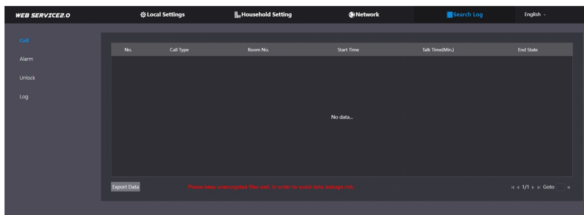
Figure 7-1 Call
