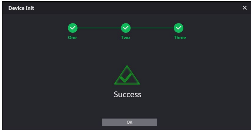
Figure 3-3 Initialization successful
