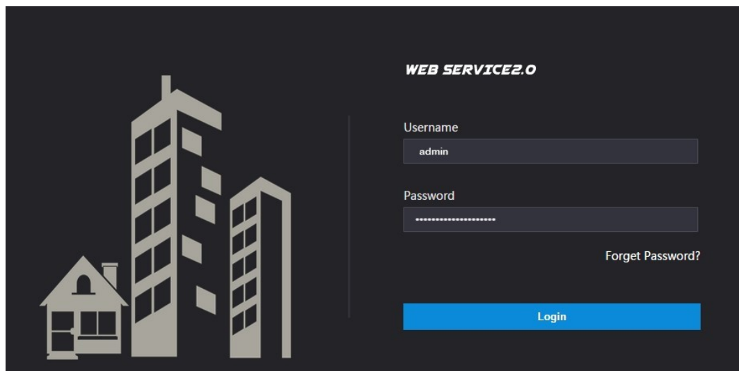
Figure 3-4 Login page
