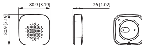
Figure 3-2 Dimensions (inch[mm])
