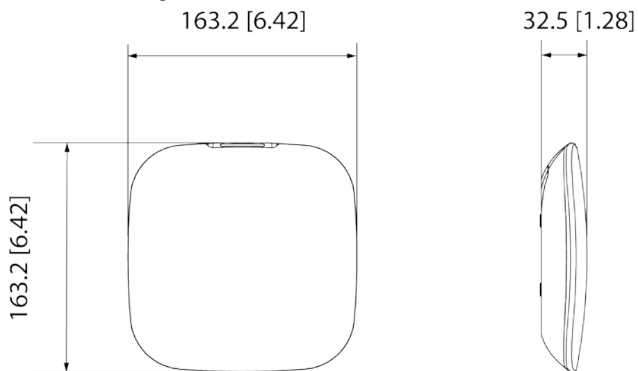
Figure 3-2 Dimensions (mm[inch])
