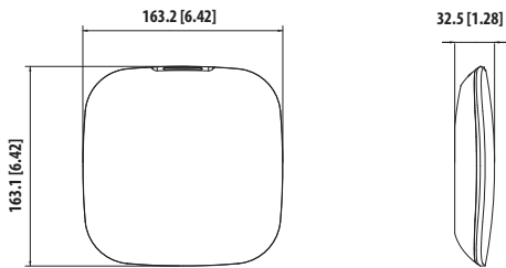
Figure 3-2 Dimensions (inch[mm])
