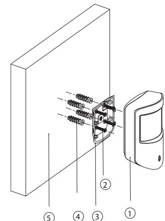
Figure 5-1 Installation items
