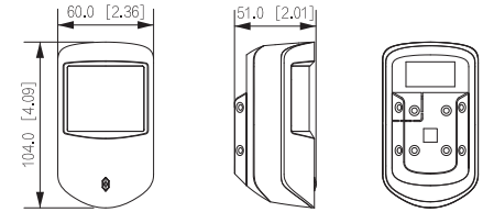
Figure 3-2 Dimensions (mm[inch])
