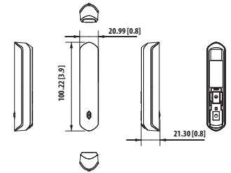
Figure 3-2 Dimensions (mm[inch])
