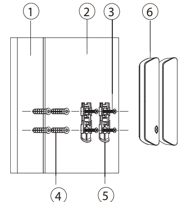
Figure 5-1 Installation
