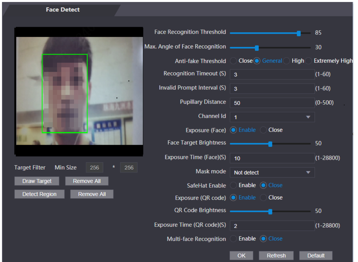
Figure 3-8 Face detect
