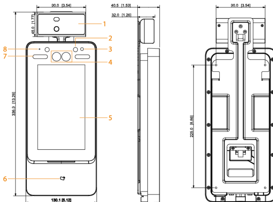
Figure 1-3 Dimensions and components of model Y (mm [inch])
