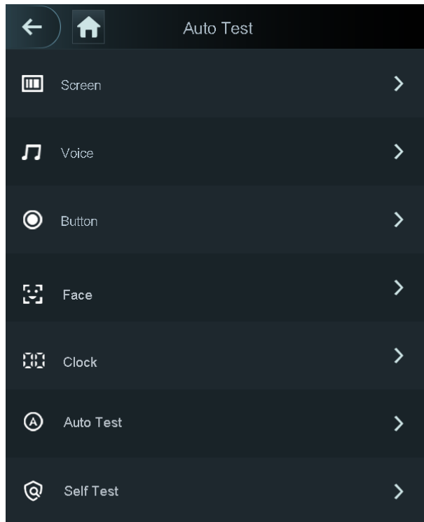
Figure 3-25 Auto test
