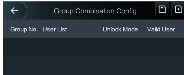
Figure 3-9 Group combination
