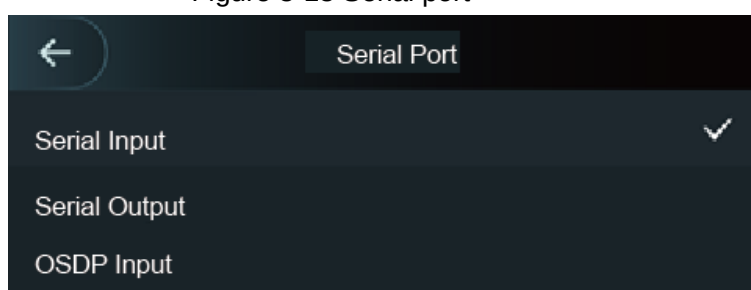
Figure 3-13 Serial port
