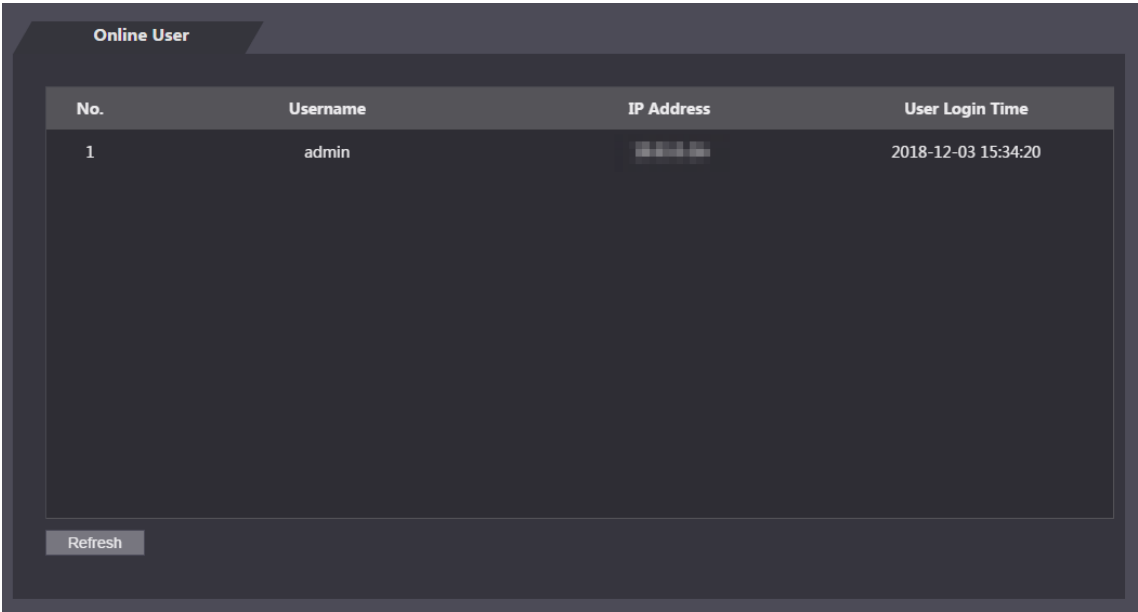
Figure 4-42 Online user
