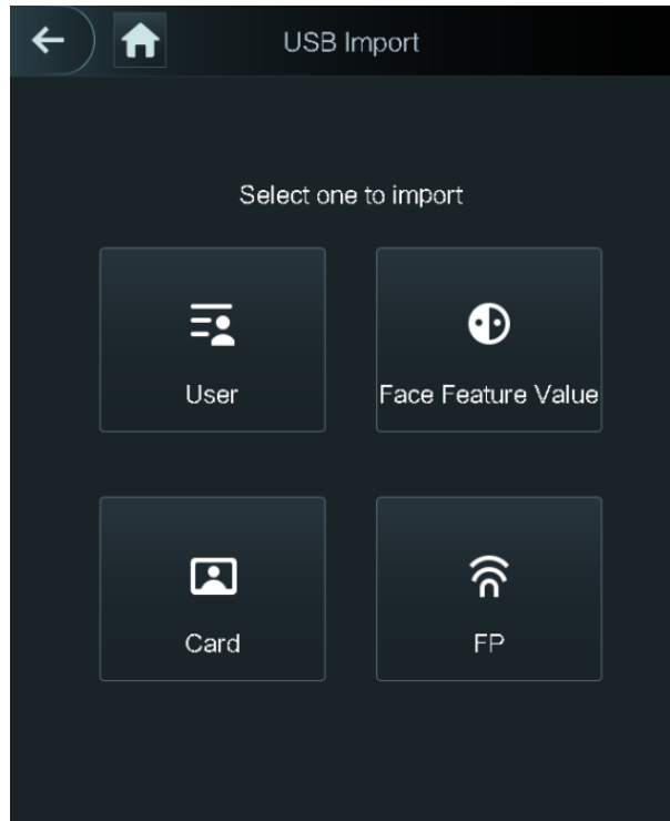
Figure 3-17 USB Import
