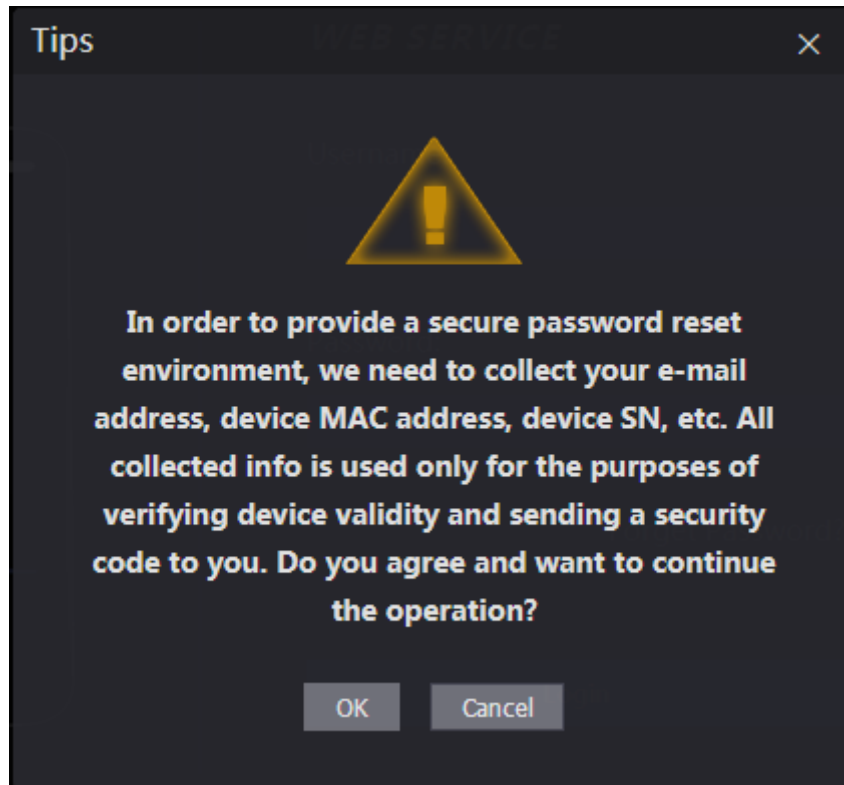
Figure 4-5 Tips
