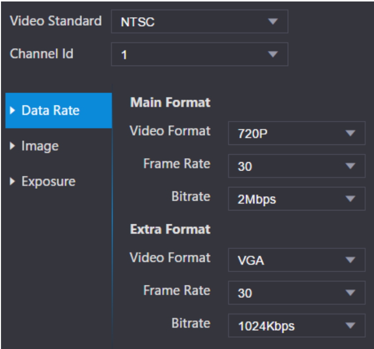
Figure 4-25 Data rate
