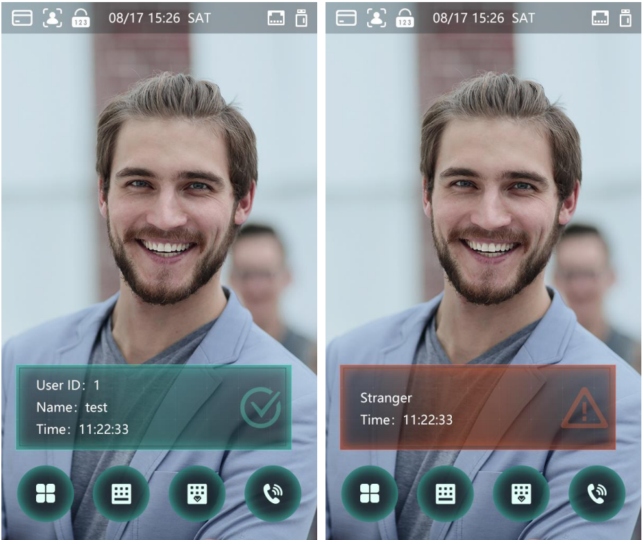
Figure 3-22 Only name
