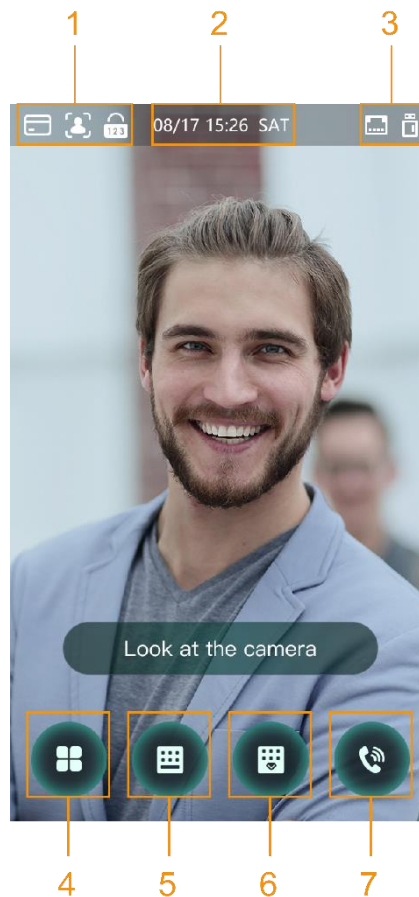
Figure 3-3 Homepage
