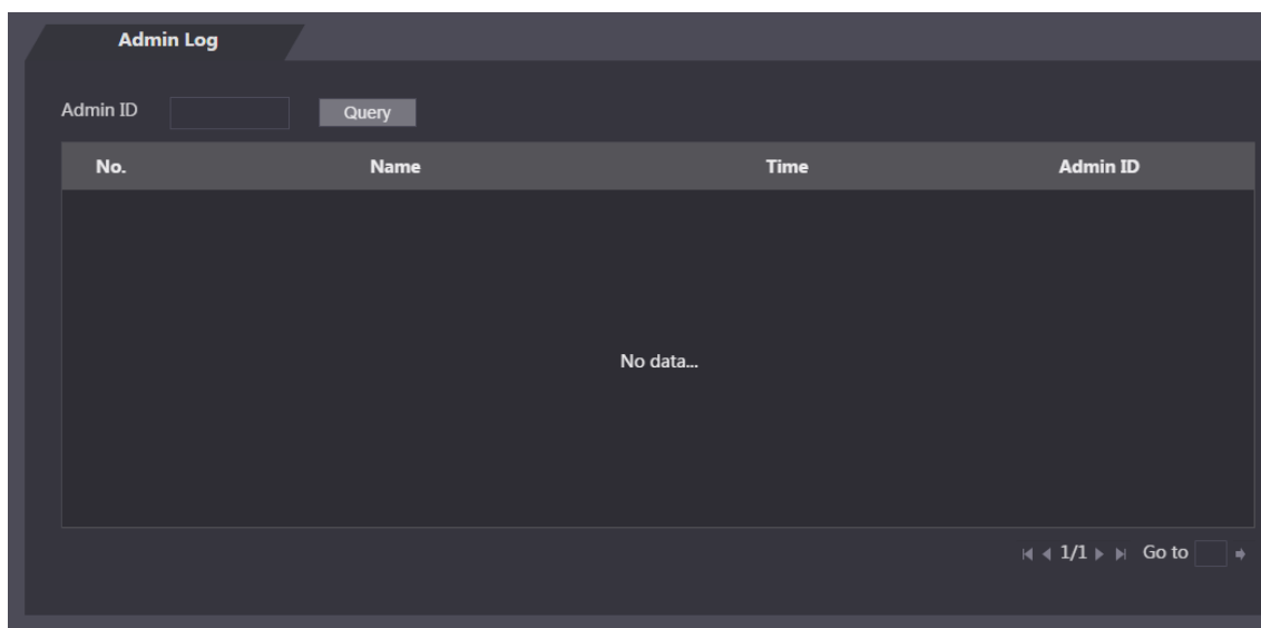
Figure 4-44 Admin log
