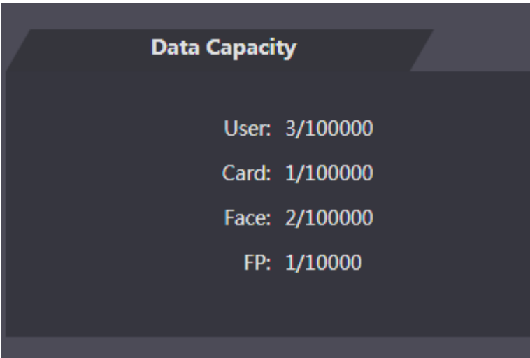
Figure 4-24 Data capacity
