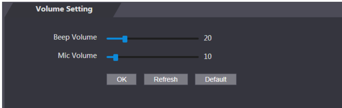
Figure 4-29 Volume setting
