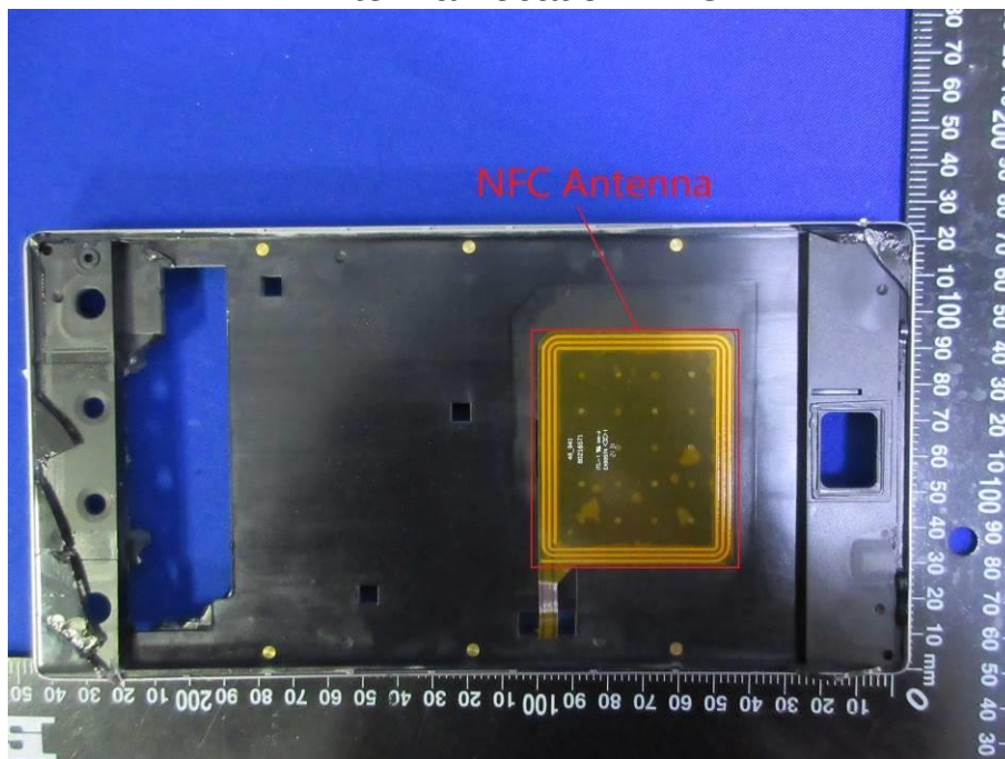
Antenna Location-NFC
