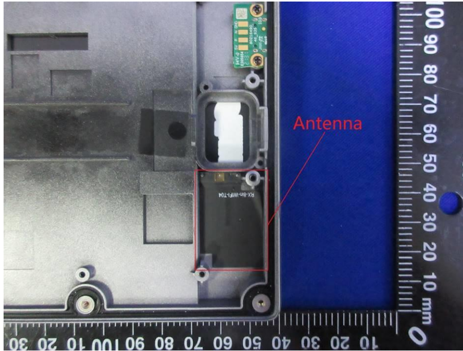
Antenna Location-WLAN
