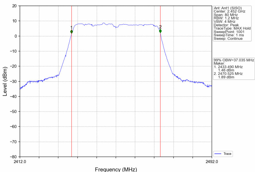
802.11n(HT40)_HCH_2452MHz_Ant1 (SISO)_NTN
