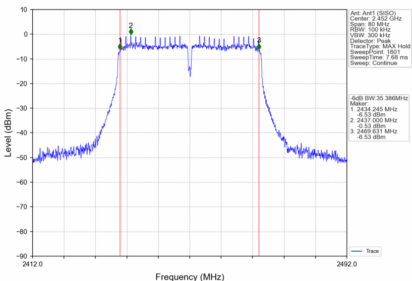
802.11n(HT40)_HCH_2452MHz_Ant1 (SISO)_NTN
