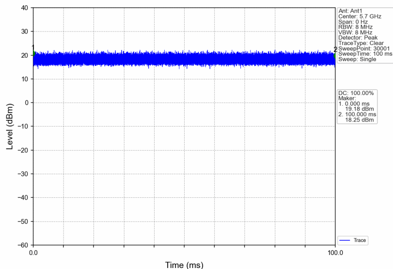
802.11ac(VHT20)_LCH_5745MHz_Ant1_NTNV
