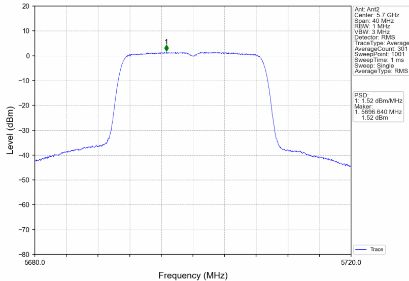
802.11n(HT20)_HCH_5700MHz_MIMO_NTNV
