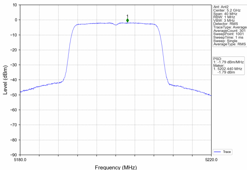
802.11ac(VHT20)_MCH_5200MHz_MIMO_NTNV
