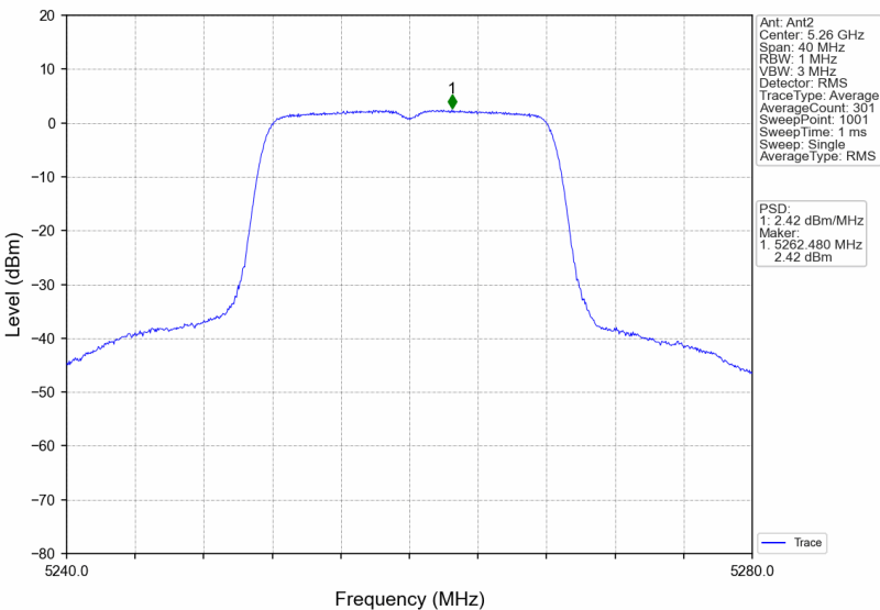
802.11n(HT20)_LCH_5260MHz_MIMO_NTNV
