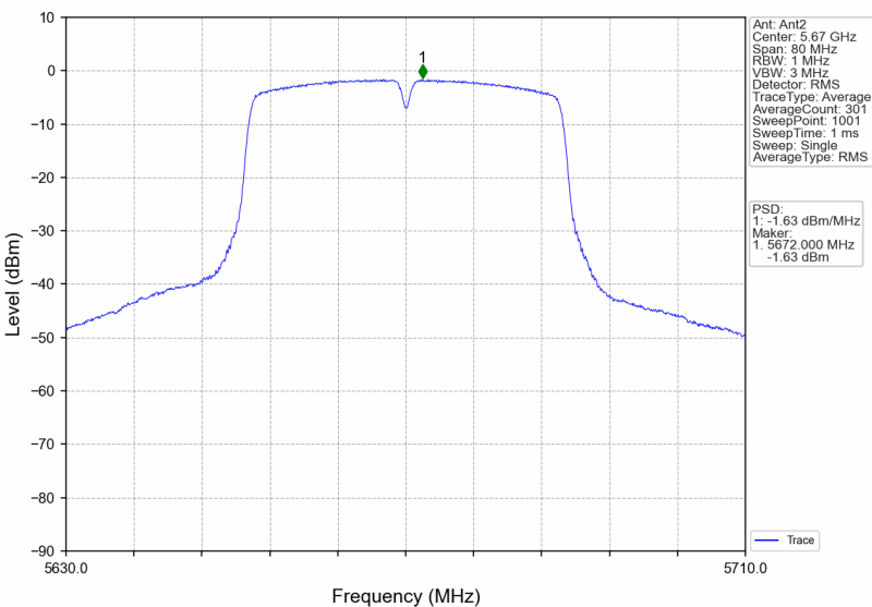
802.11n(HT40)_HCH_5670MHz_MIMO_NTNV
