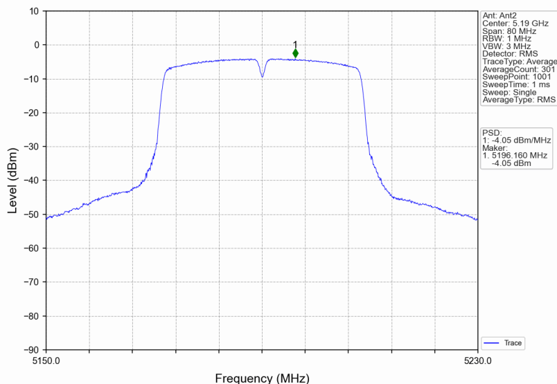
802.11n(HT40)_LCH_5190MHz_MIMO_NTNV
