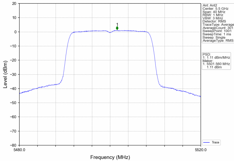
802.11ac(VHT20)_LCH_5500MHz_MIMO_NTNV
