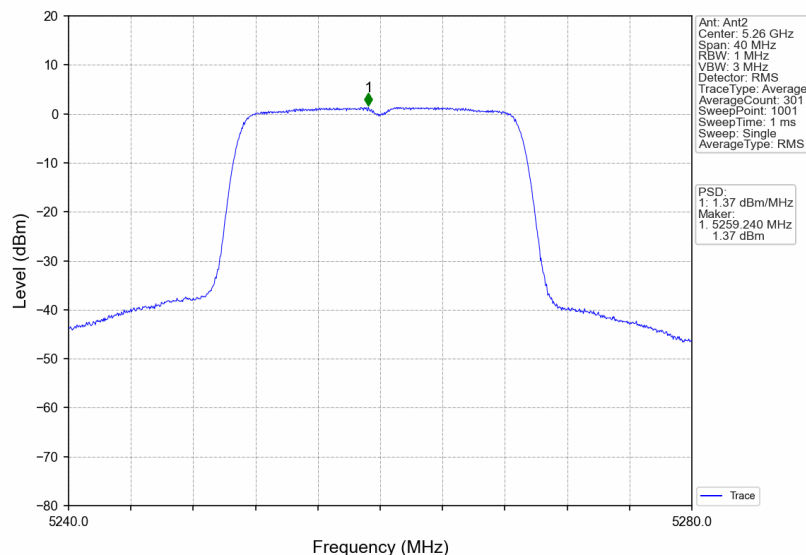
802.11ac(VHT20)_LCH_5260MHz_MIMO_NTNV
