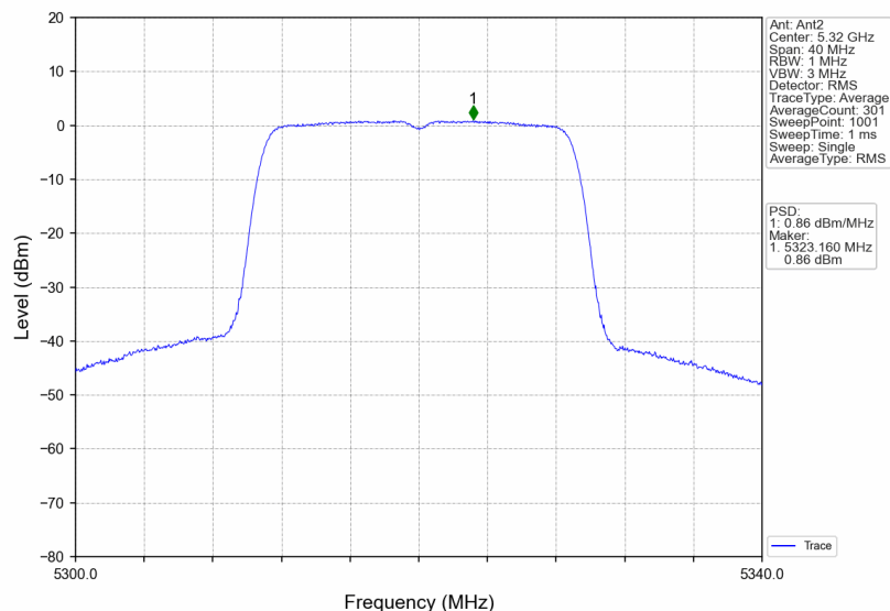
802.11ac(VHT20)_HCH_5320MHz_MIMO_NTNV
