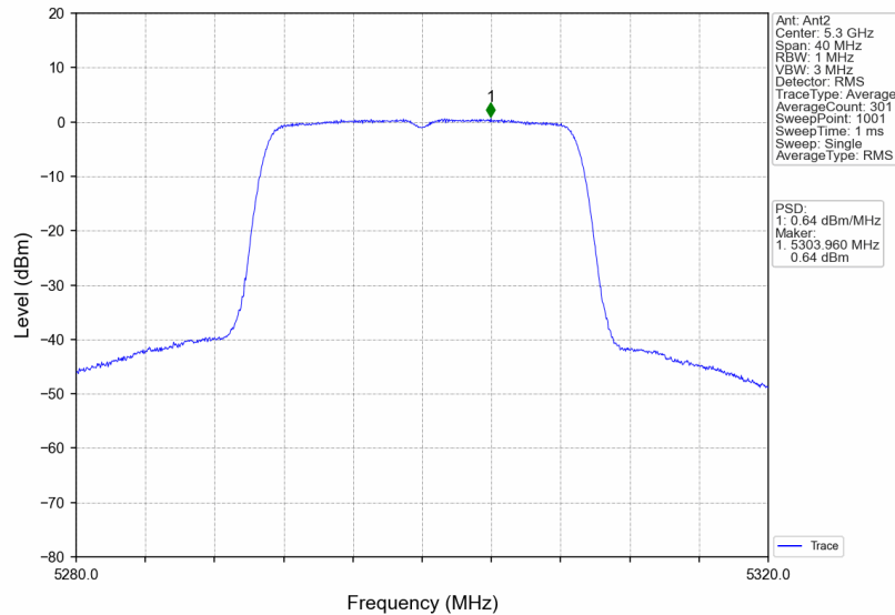
802.11ac(VHT20)_MCH_5300MHz_MIMO_NTNV
