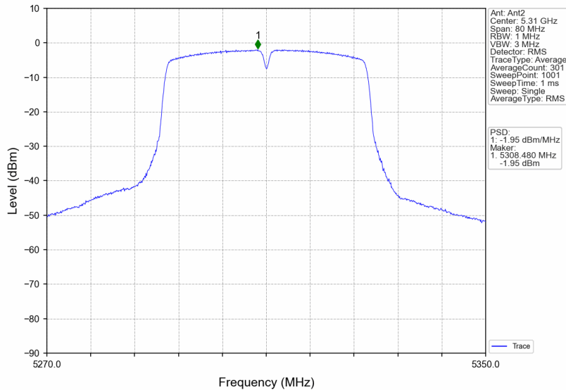
802.11n(HT40)_HCH_5310MHz_MIMO_NTNV
