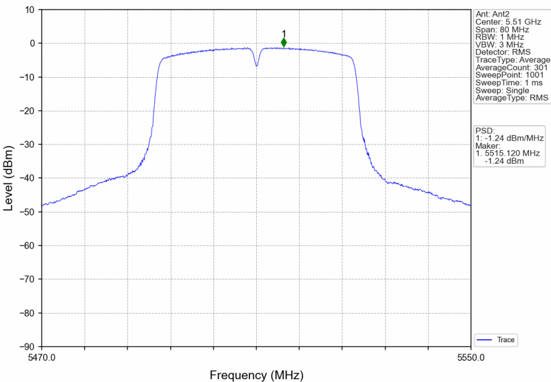
802.11n(HT40)_LCH_5510MHz_MIMO_NTNV
