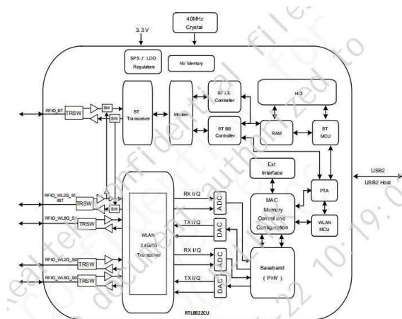
Figure 3 BL-M8822CU1
