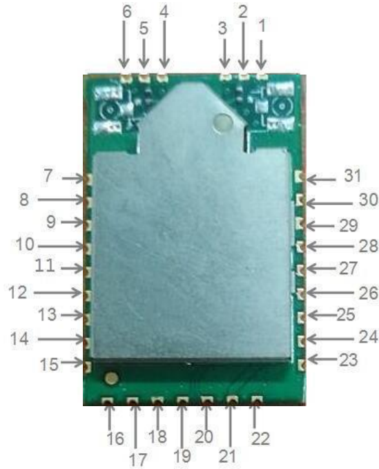
Figure 4 Top view
