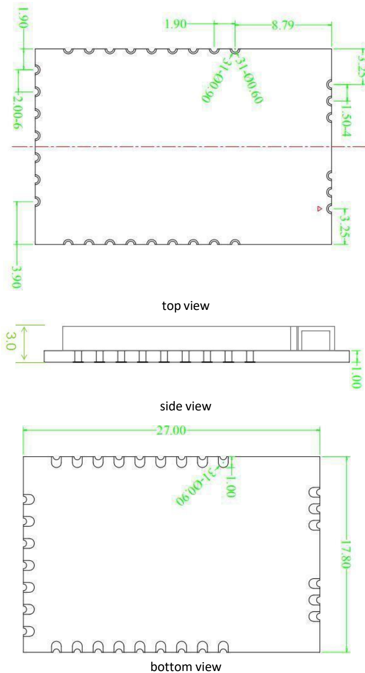
Figure 6 Module dimension (top , side and bottom view)
