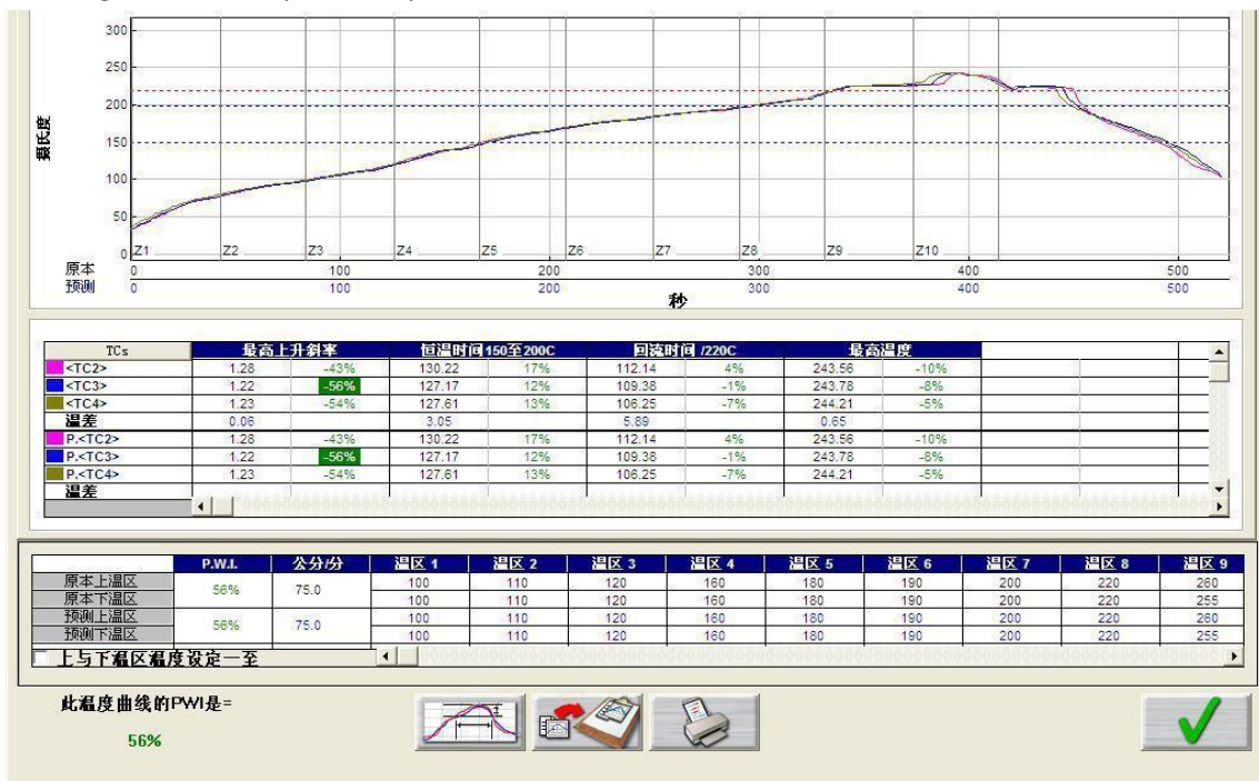
Figure 7 Typical Solder Reflow Profile
