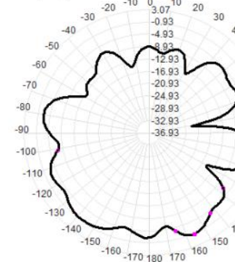
Total(H-XY), Max= -1.03dBi, CirD=22.05
