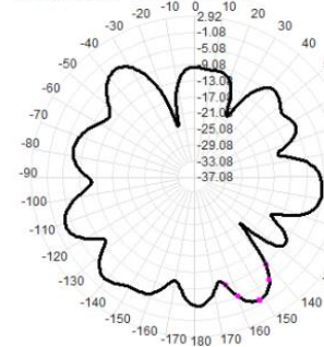
Total(H-XY), Max= -2.52dBi, CirD=21.40
