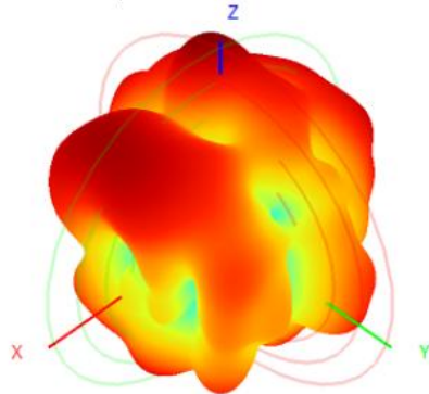
2450.0MHz H+V, Eff: 48.7%
