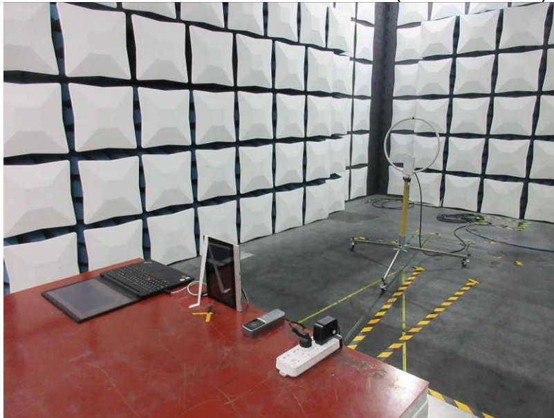
RADIATED RF MEASUREMENT SETUP (9kHz ~ 30 MHz)
