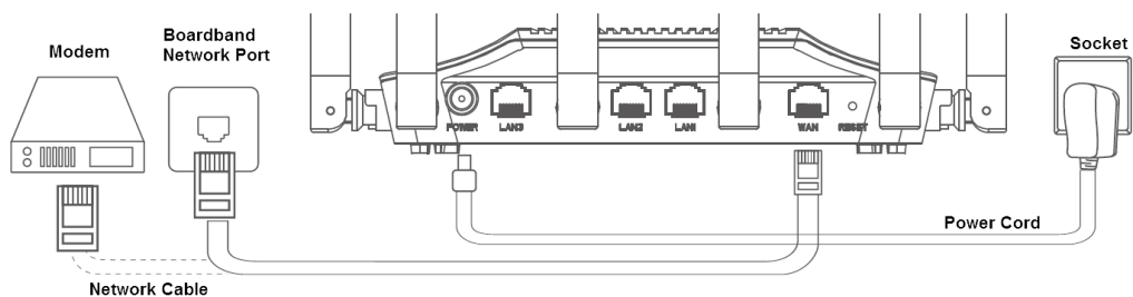
Figure 1-1 Connection diagram
