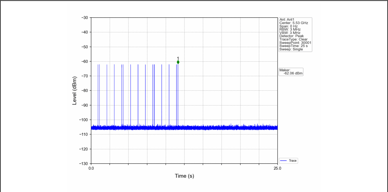
Signal Calibration_802.11ac(VHT80)_2C_5530MHz_RadarType6_Trial0
