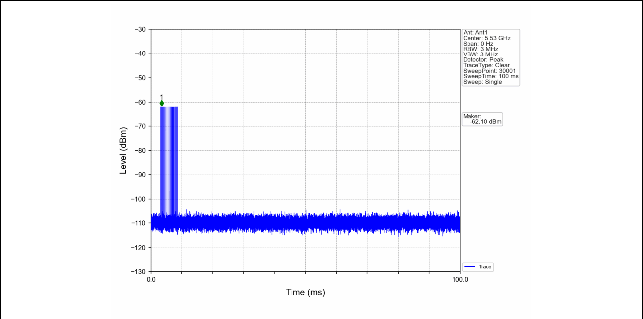
Signal Calibration_802.11ac(VHT80)_2C_5530MHz_RadarType4_Trial0
