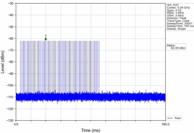
Signal Calibration_802.11ac(VHT80)_2A_5290MHz_RadarType2_Trial0
