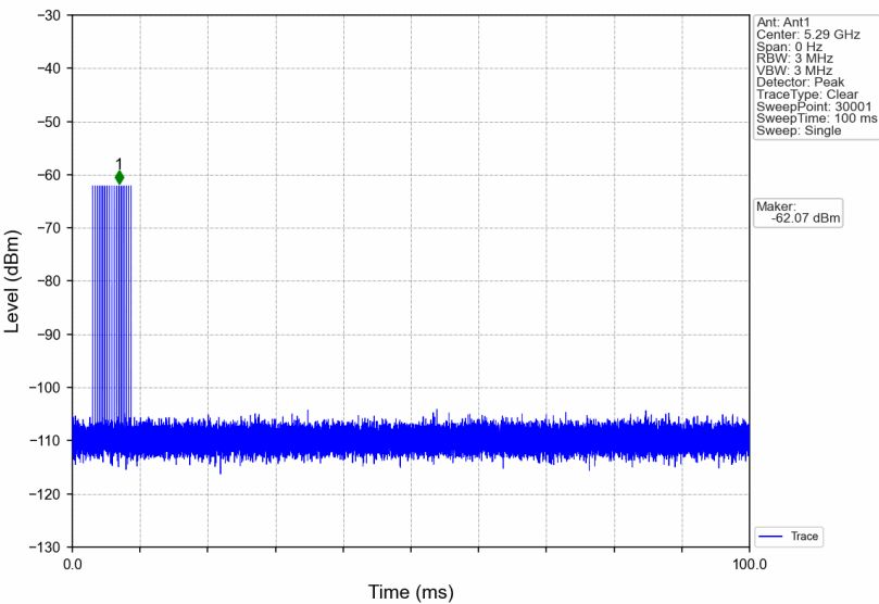
Signal Calibration_802.11ac(VHT80)_2A_5290MHz_RadarType4_Trial0
