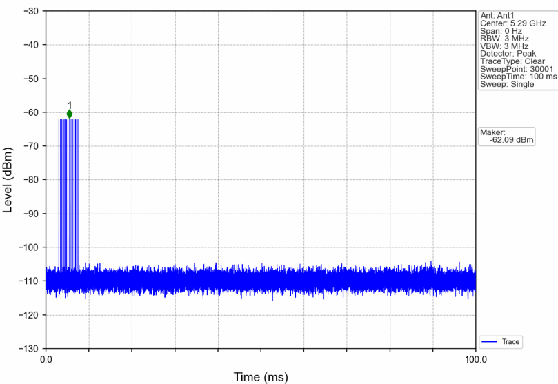
Signal Calibration_802.11ac(VHT80)_2A_5290MHz_RadarType5_Trial0
