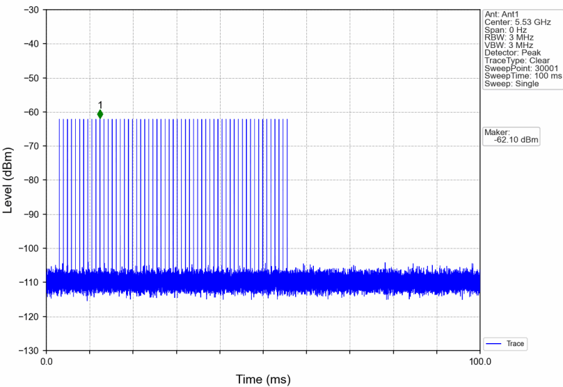
Signal Calibration 802.11ac(VHT80)_2C_5530MHz_RadarType2_Trial0
