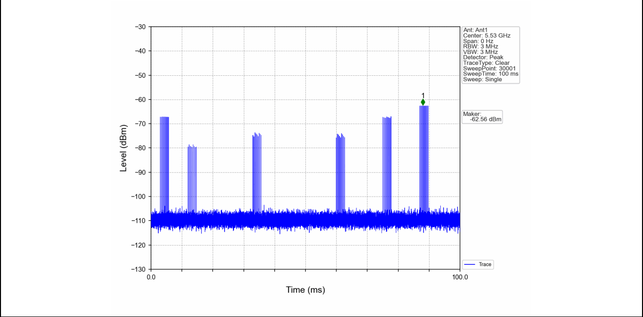
Signal Calibration_802.11ac(VHT80)_2C_5530MHz_RadarType6_Trial0
