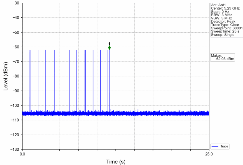
Signal Calibration_802.11ac(VHT80)_2A_5290MHz_RadarType6_Trial0
