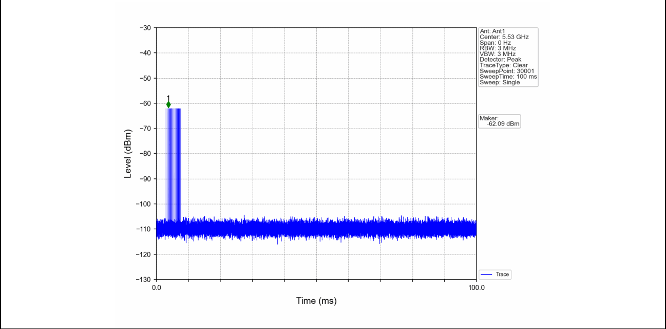
Signal Calibration_802.11ac(VHT80)_2C_5530MHz_RadarType5_Trial0
