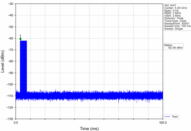
Signal Calibration_802.11ac(VHT80)_2A_5290MHz_RadarType3_Trial0
