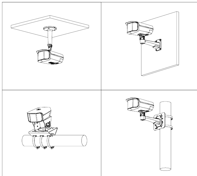
Figure 3-3 Installation method
