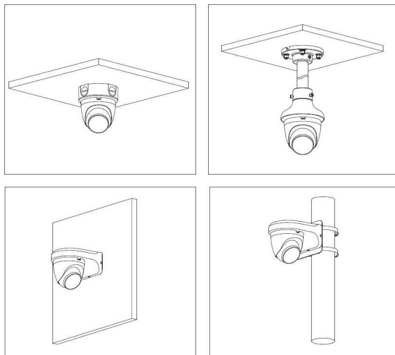
Figure 4-3 Installation method
