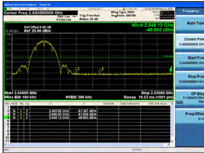
11B_Ant2_High_2462
