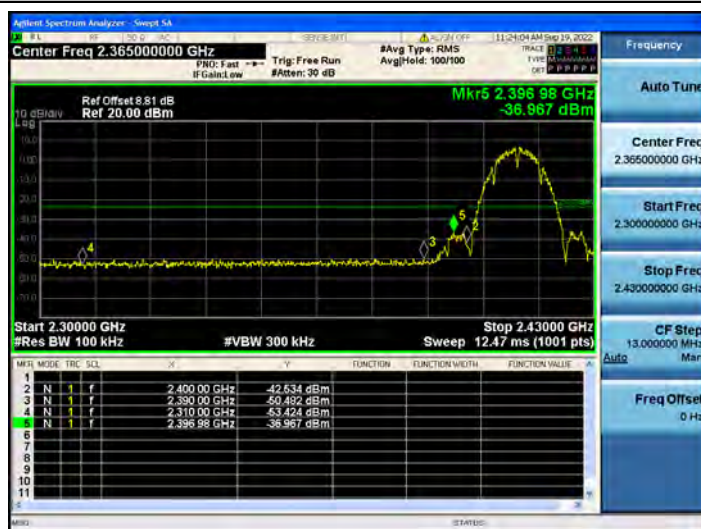
11B_Ant2_Low_2412
