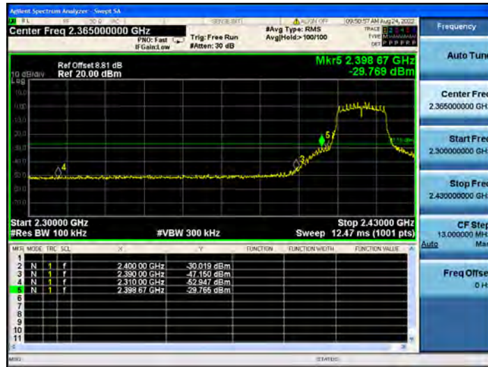
11G_Ant2_Low_2412
