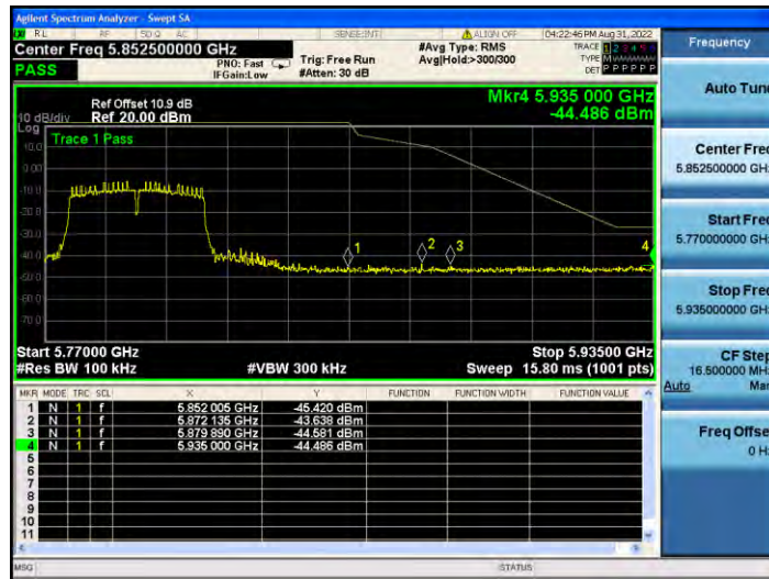
11N40MIMO_Ant2_High_5795
