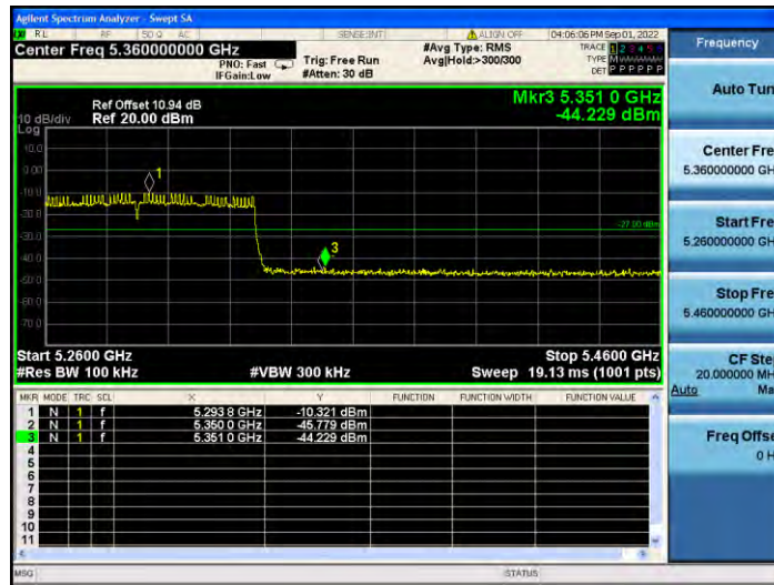
11AC80MIMO_Ant2_High_5290
