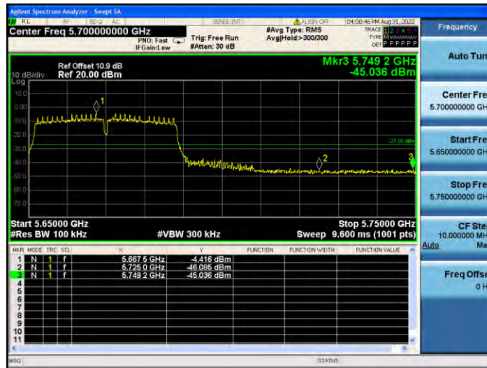
11N40MIMO_Ant2_High_5670
