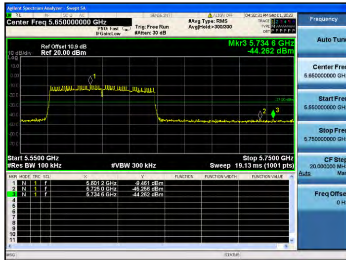
11AC80MIMO_Ant2_High_5610
