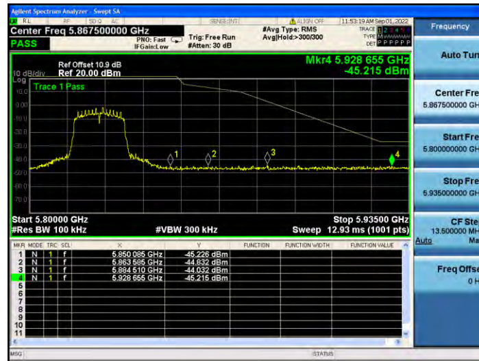
11AC20MIMO_Ant2_High_5825
