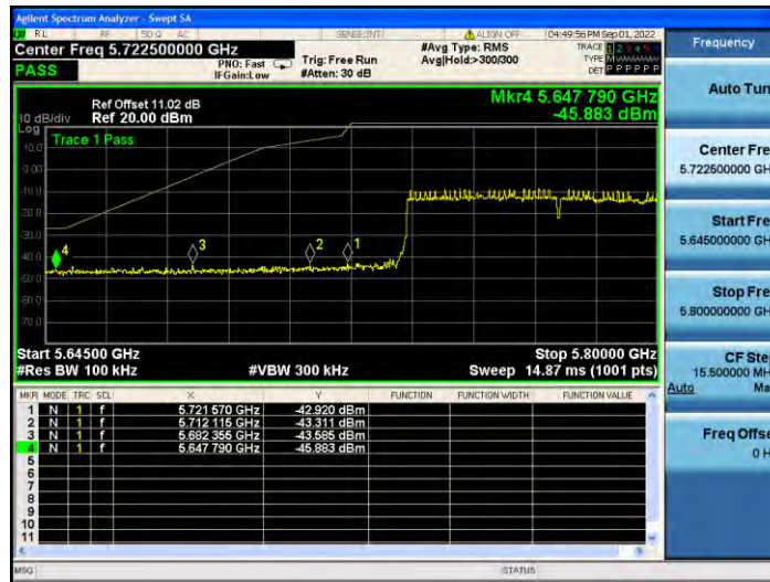
11AC80MIMO_Ant2_High_5775
