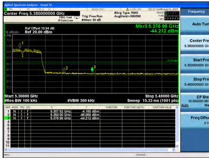
11N40MIMO_Ant2_High_5310
