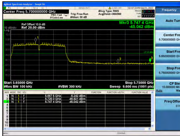
11AC40MIMO_Ant2_High_5670
