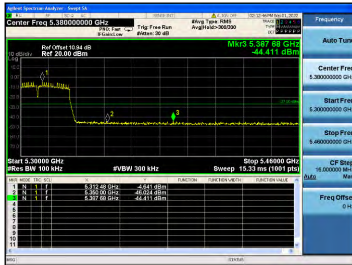
11AC40MIMO_Ant2_High_5310
