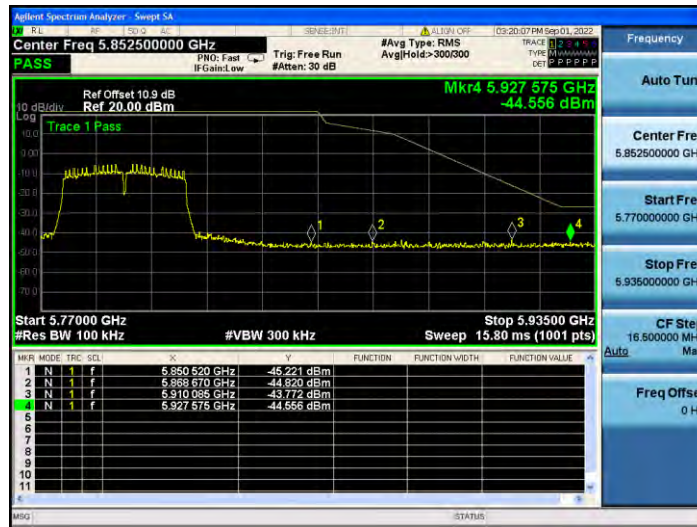
11AC40MIMO_Ant2_High_5795
