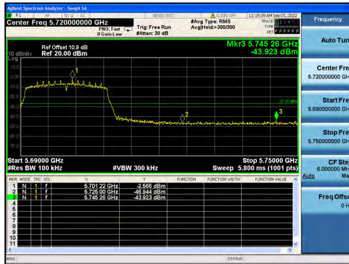
11AC20MIMO_Ant2_High_5700
