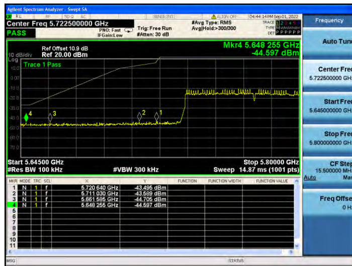
11AC80MIMO_Ant1_High_5775
