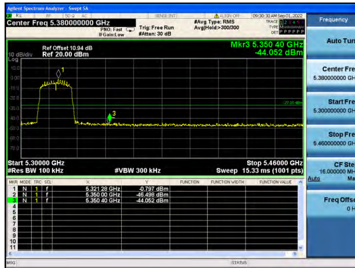
11AC20MIMO_Ant2_High_5320
