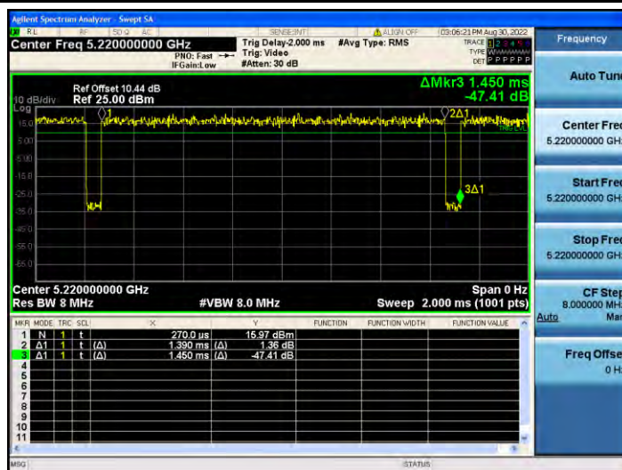
11A Ant2 5220
