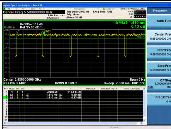
11AC20MIMO Ant2 5580
