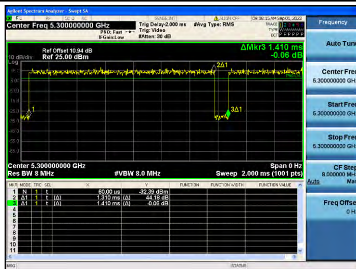
11AC20MIMO Ant2 5300
