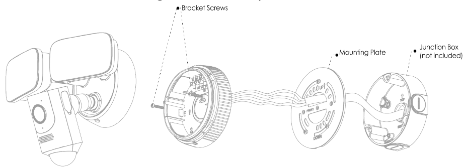
Figure 2-1 Assembly
