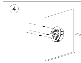
Lock the Mounting Plate
