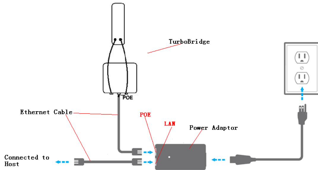
Figure 6 Connections at Bridge mode
