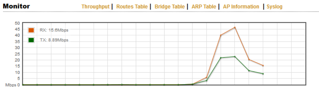
Figure 16 Throughput monitor
