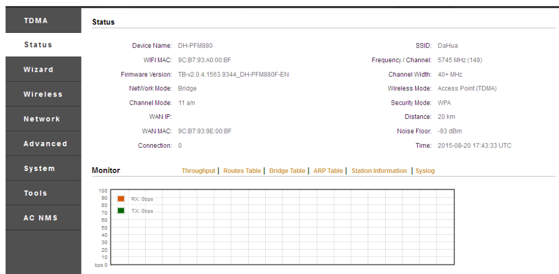
Figure 10 Status Page
