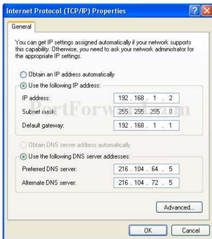
Figure 8 IP settings
