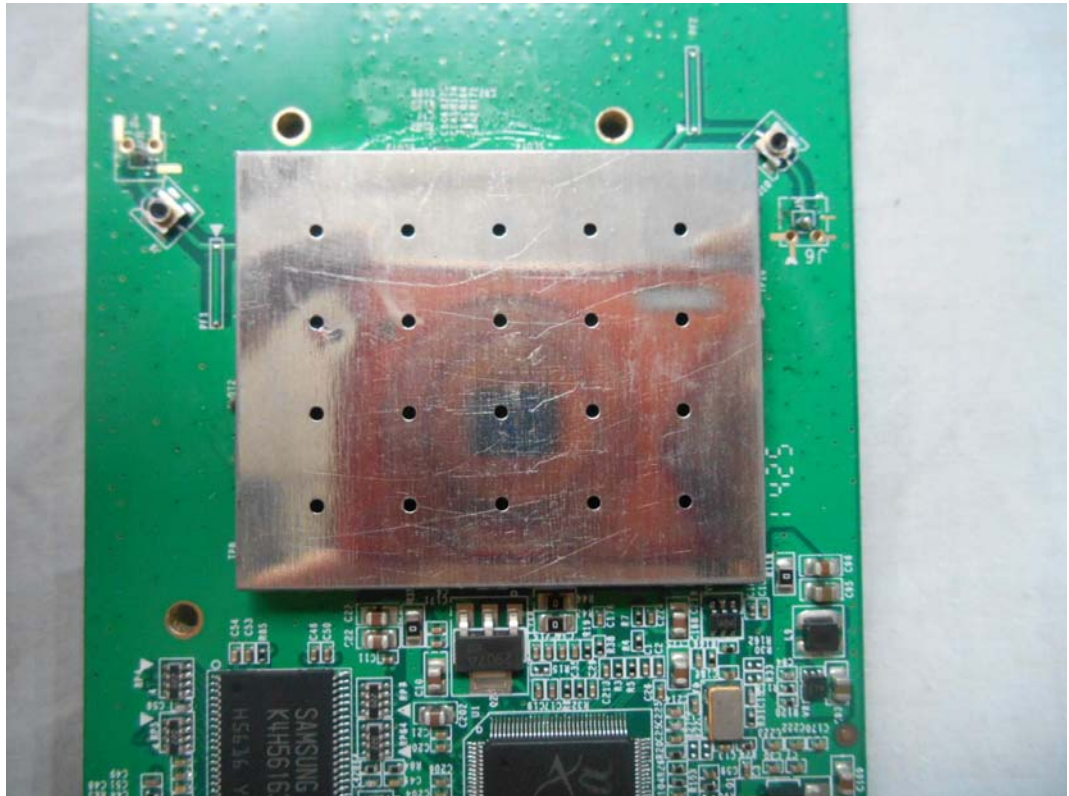
FIGURE 11 CPE (M/N: DH-PFM881) MAIN BOARD (RF PART)
