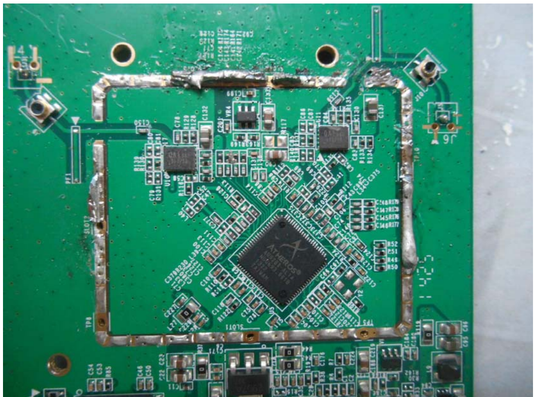
FIGURE 12 CPE (M/N: DH-PFM881) MAIN BOARD (RF PART SHIELDED COVER REMOVED)
