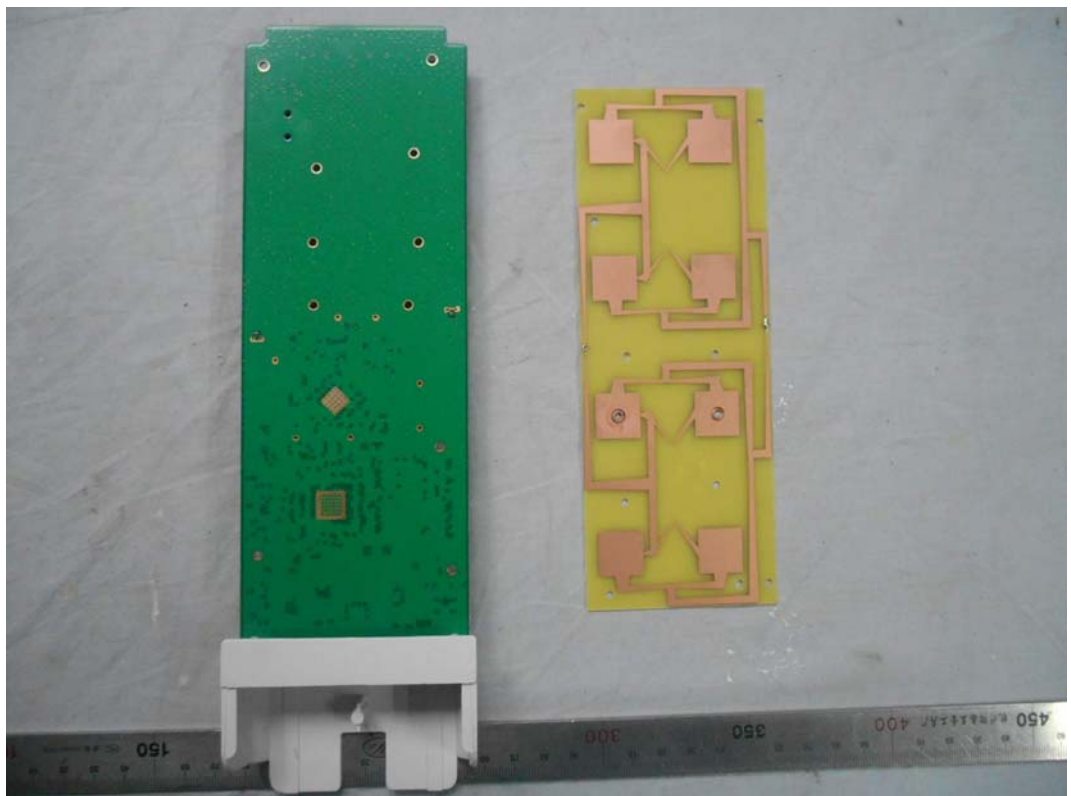
FIGURE 8 CPE (M/N: DH-PFM881) MAIN BOARD (ANTENNA REMOVED)
