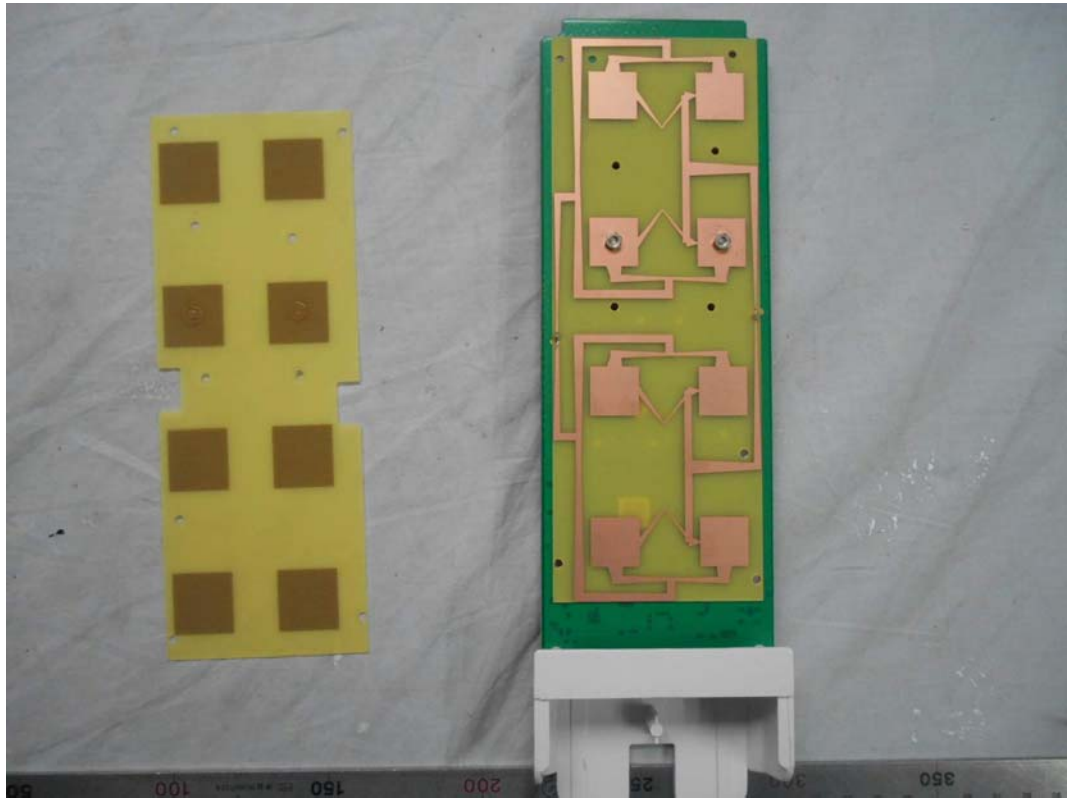
FIGURE 7 CPE (M/N: DH-PFM881) MAIN BOARD (BACK BOARD REMOVED)
