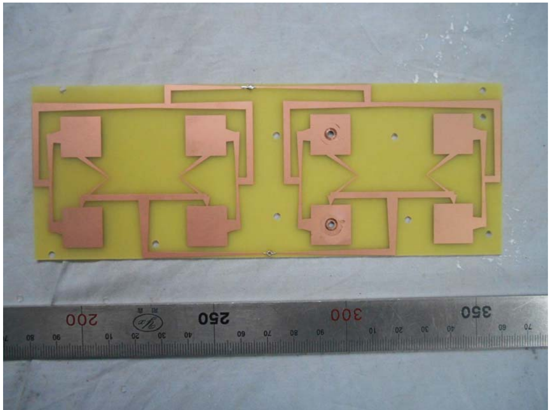
FIGURE 9 CPE (M/N: DH-PFM881) ANTENNA
