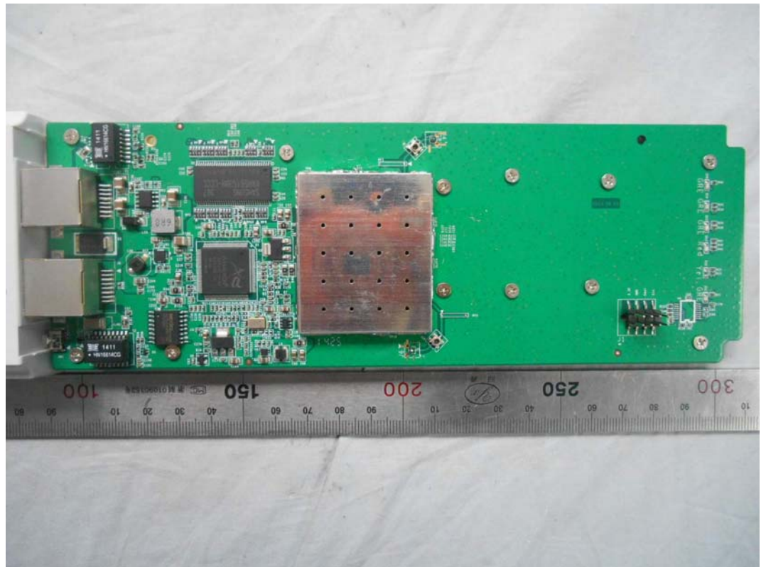
FIGURE 5 CPE (M/N: DH-PFM881) MAIN BOARD (FRONT VIEW)
