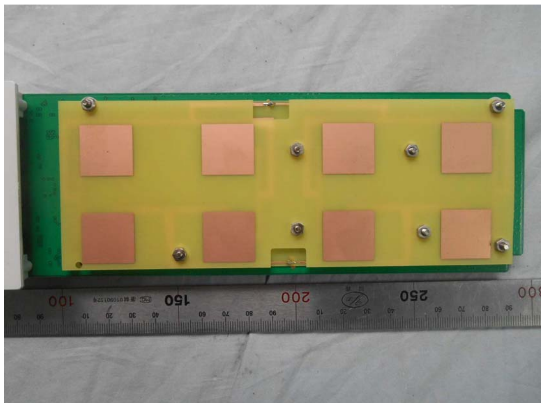
FIGURE 6 CPE (M/N: DH-PFM881) MAIN BOARD (BACK VIEW)
