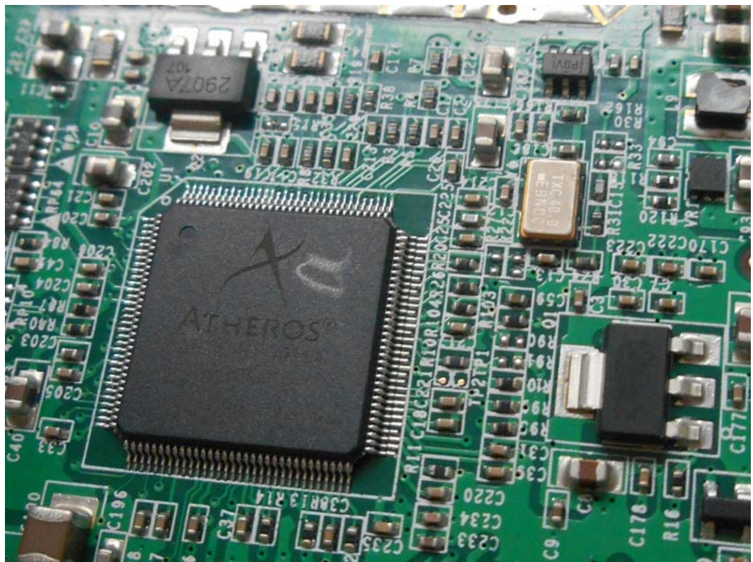
FIGURE 8 AP (M/N: DH-PFM880) CHIP & CRYSTAL ON MAIN BOARD
