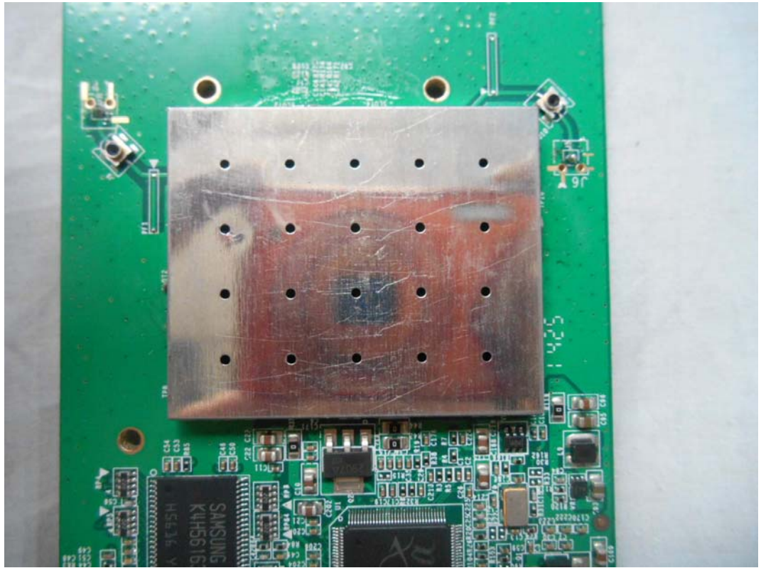
FIGURE 10 AP (M/N: DH-PFM880) MAIN BOARD (RF PART SHIELDED COVER REMOVED)
