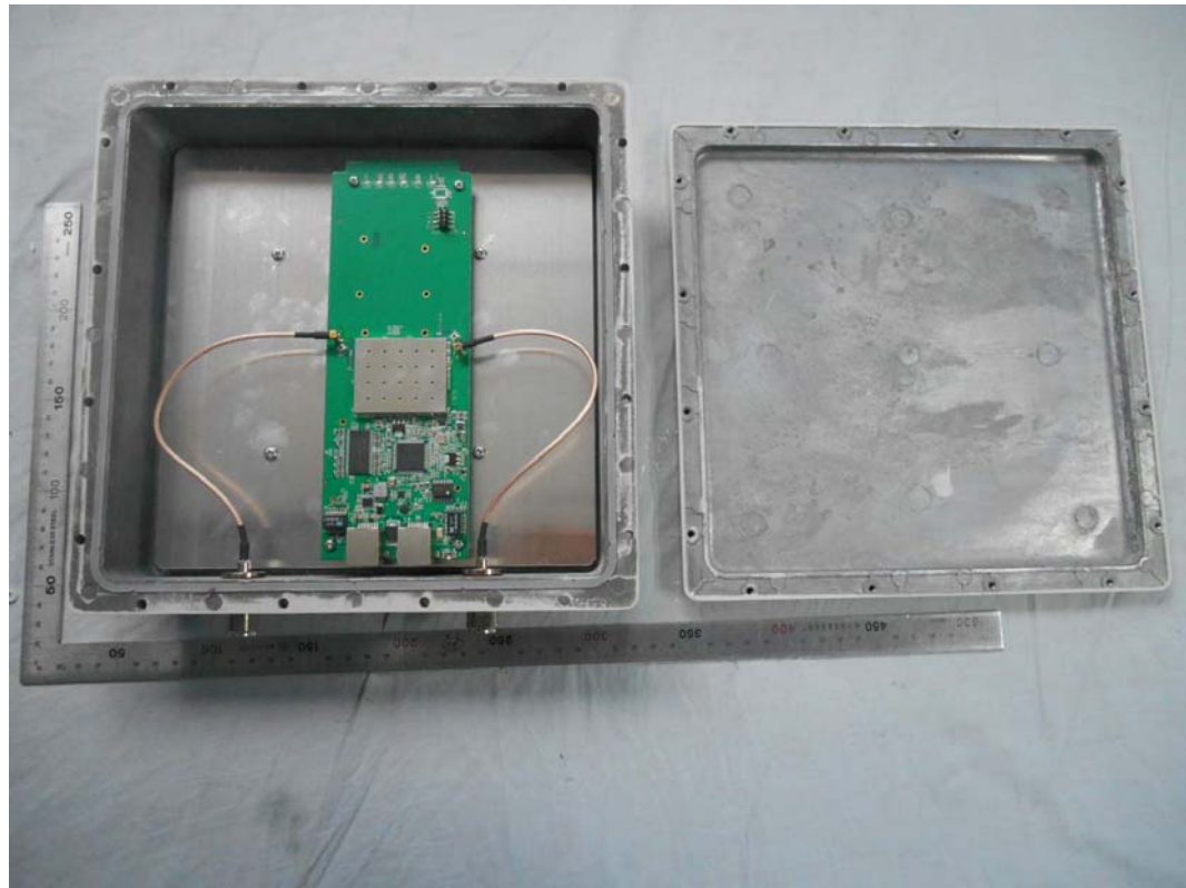
FIGURE 4 AP (M/N: DH-PFM880) COVER REMOVED
