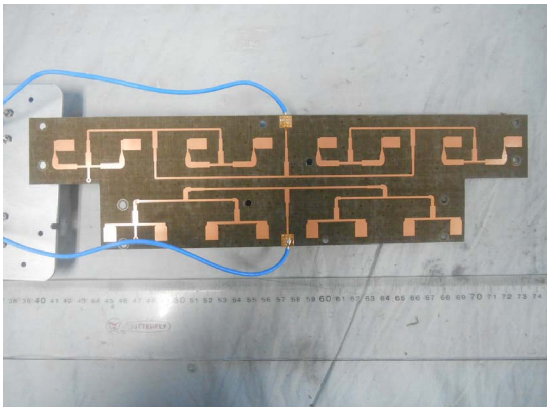
FIGURE 16 AP (M/N: DH-PFM880) ANTENNA (BACK SIDE)
