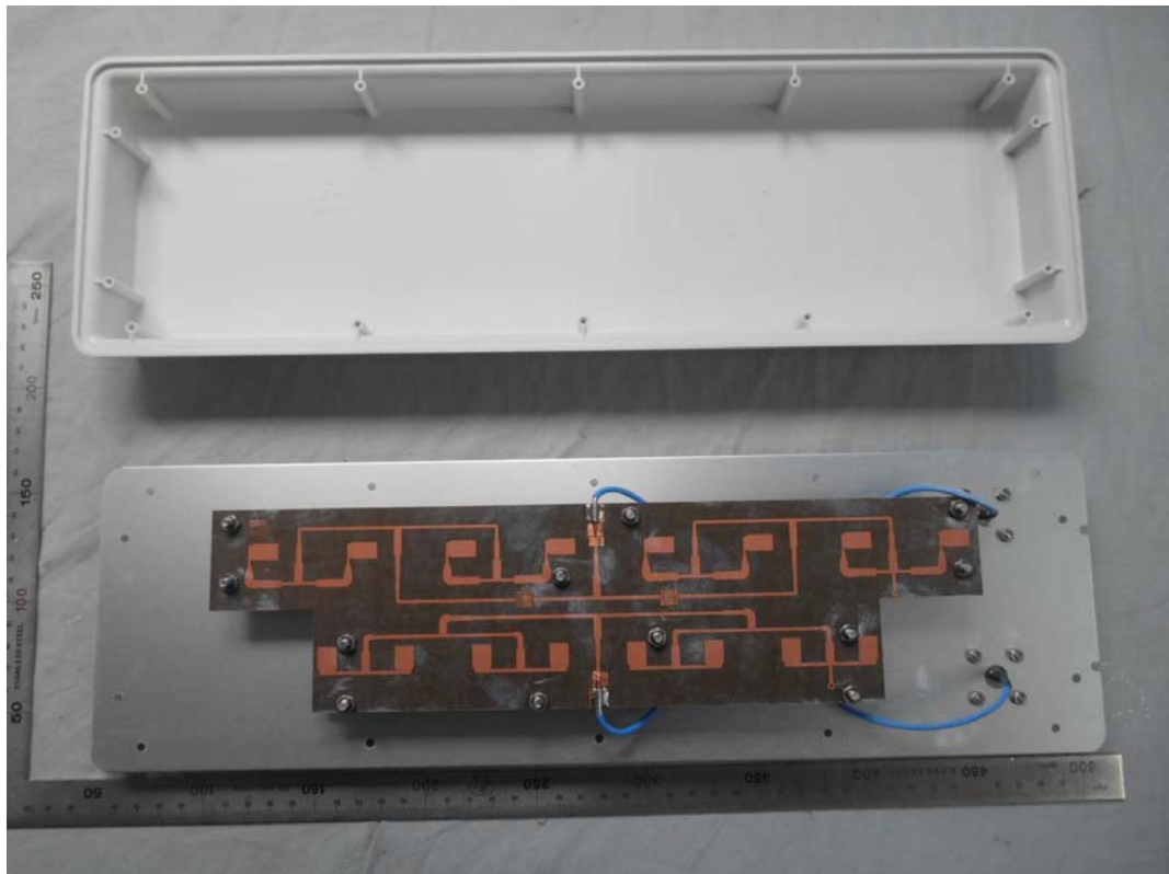
FIGURE 15 AP (M/N: DH-PFM880) ANTENNA (FRONT SIDE)
