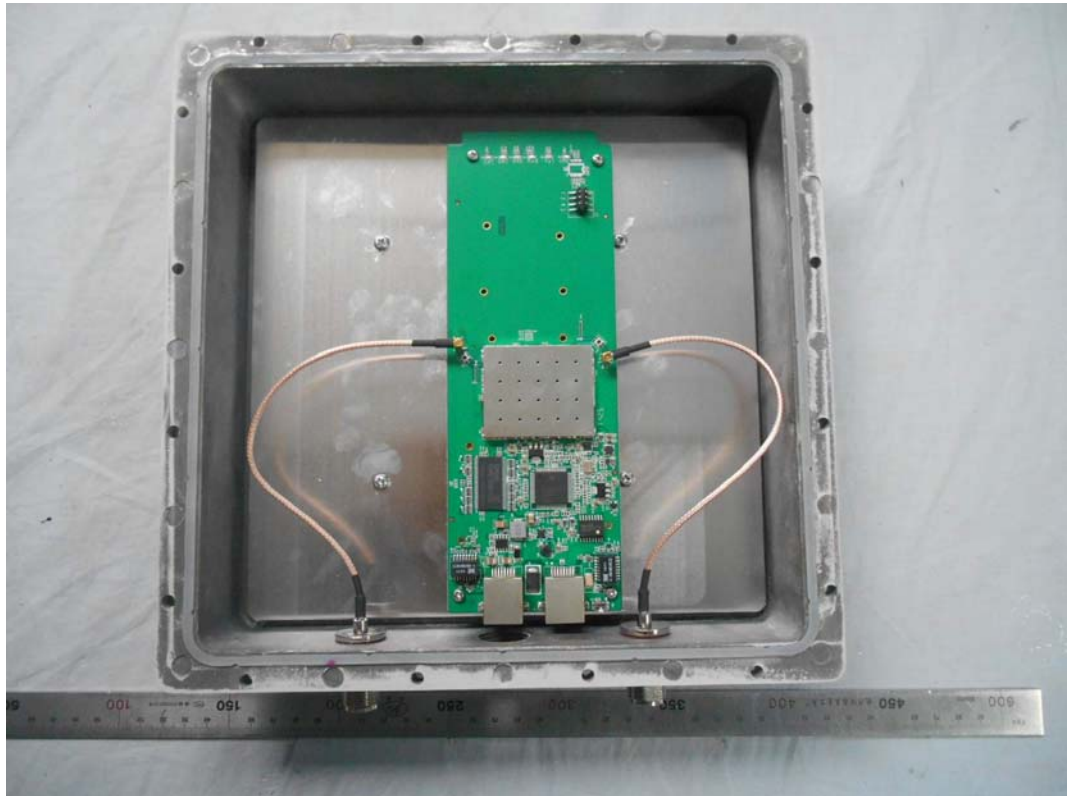
FIGURE 5 AP (M/N: DH-PFM880) INSIDE VIEW
