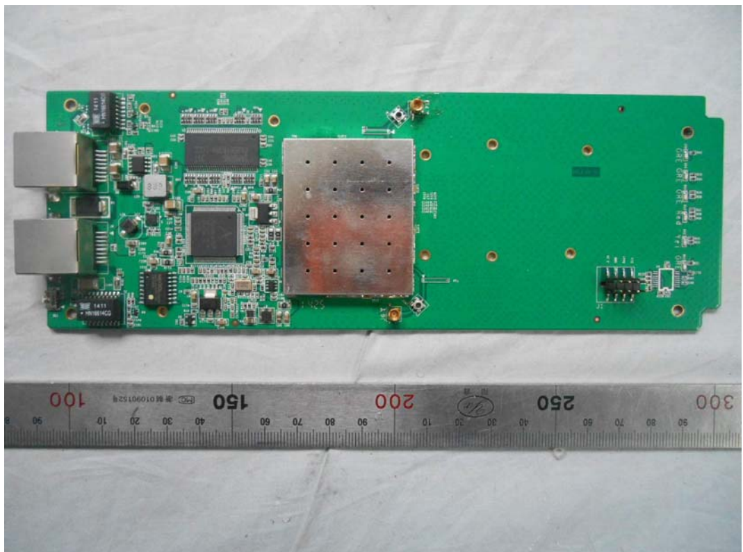
FIGURE 6 AP (M/N: DH-PFM880) MAIN BOARD (FRONT SIDE)
