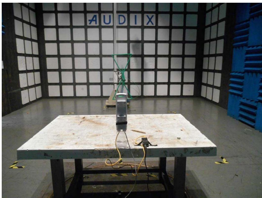
BACK VIEW OF RADIATED EMISSION TEST (DH-PFM881)
