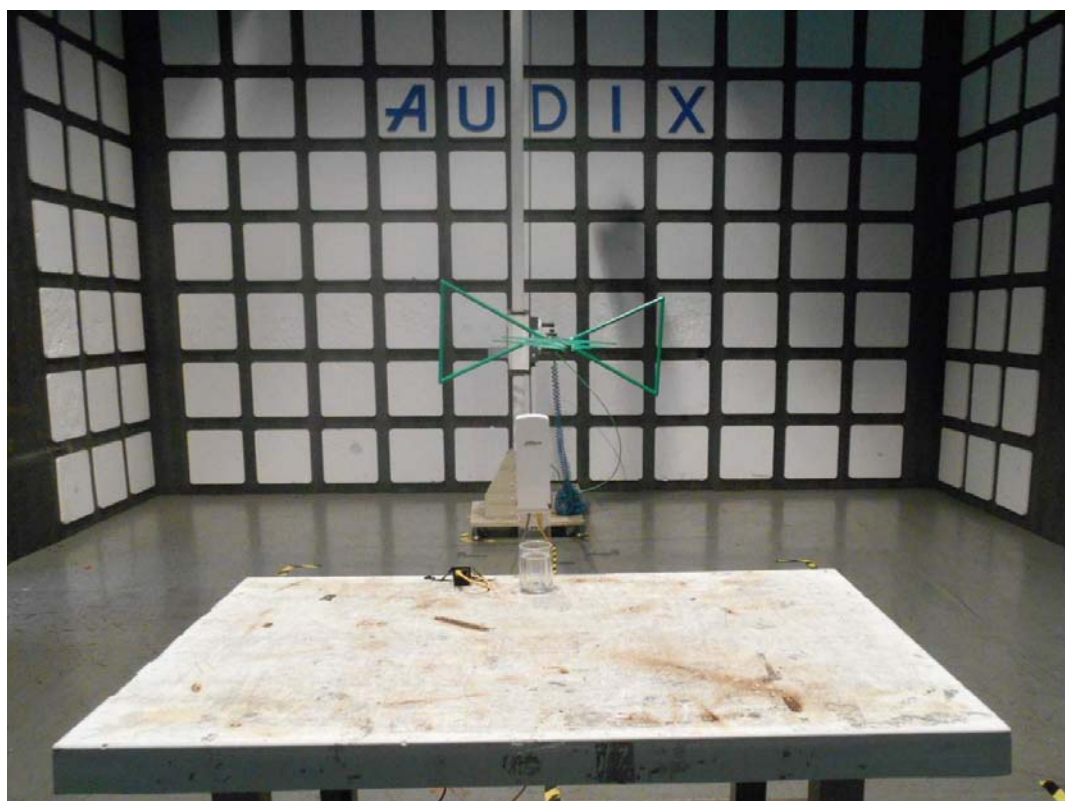
FRONT VIEW OF RADIATED EMISSION TEST (DH-PFM881)
