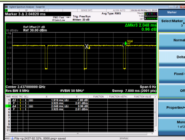
802.11n-HT20 (T = 1.919ms)
