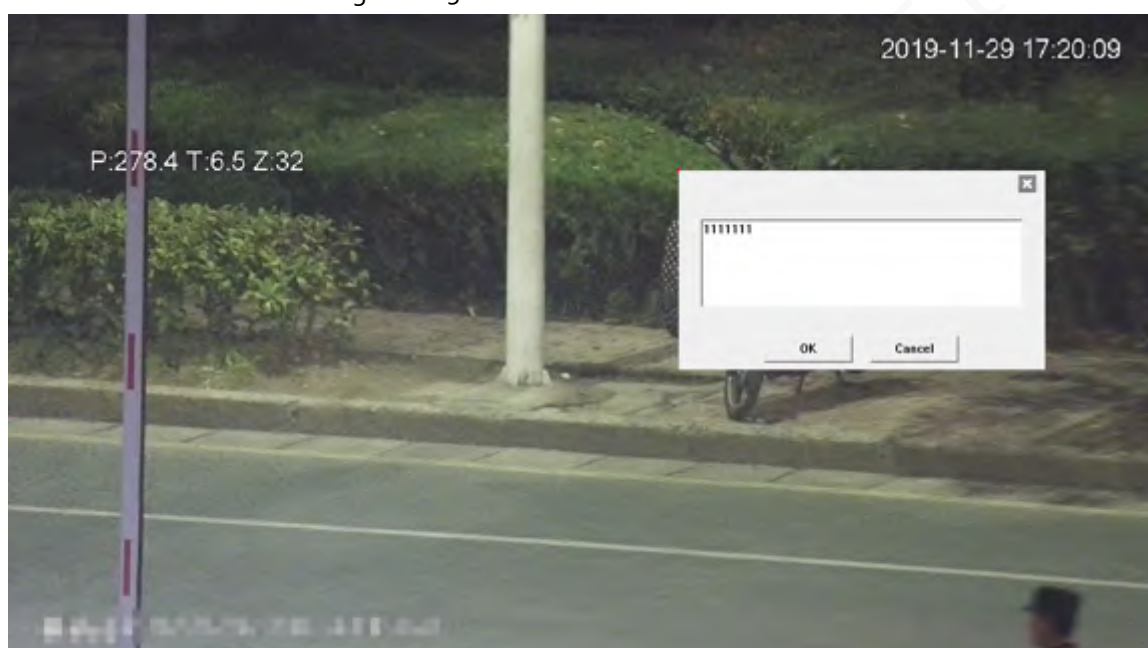
Figure 2-16 Mark—manage comments
