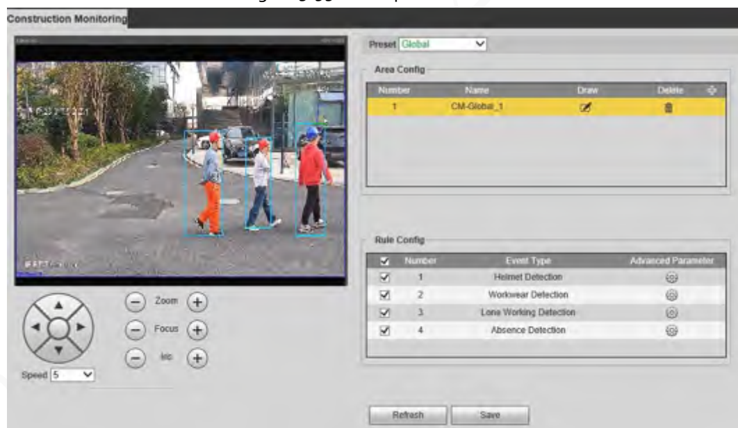
Figure 5-95 Global plan
