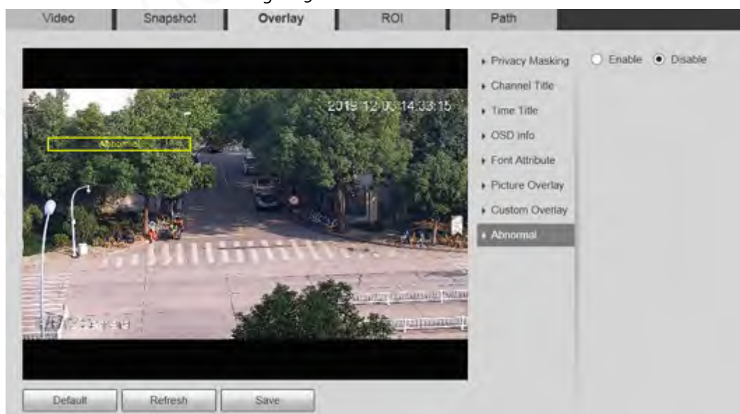
Figure 5-28 Abnormal
