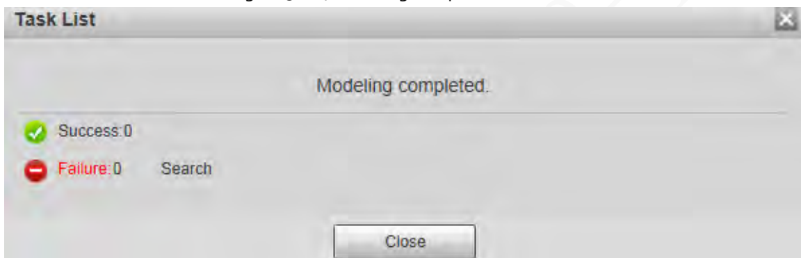
Figure 5-114 Modeling completed
