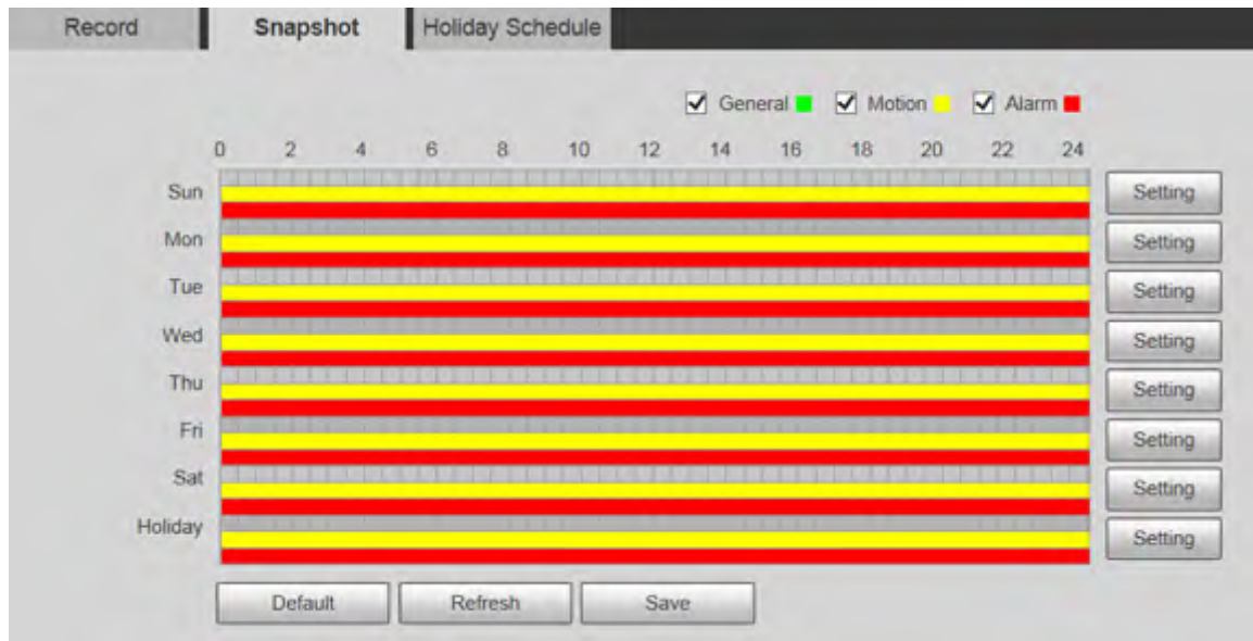
Figure 5-137 Snapshot
