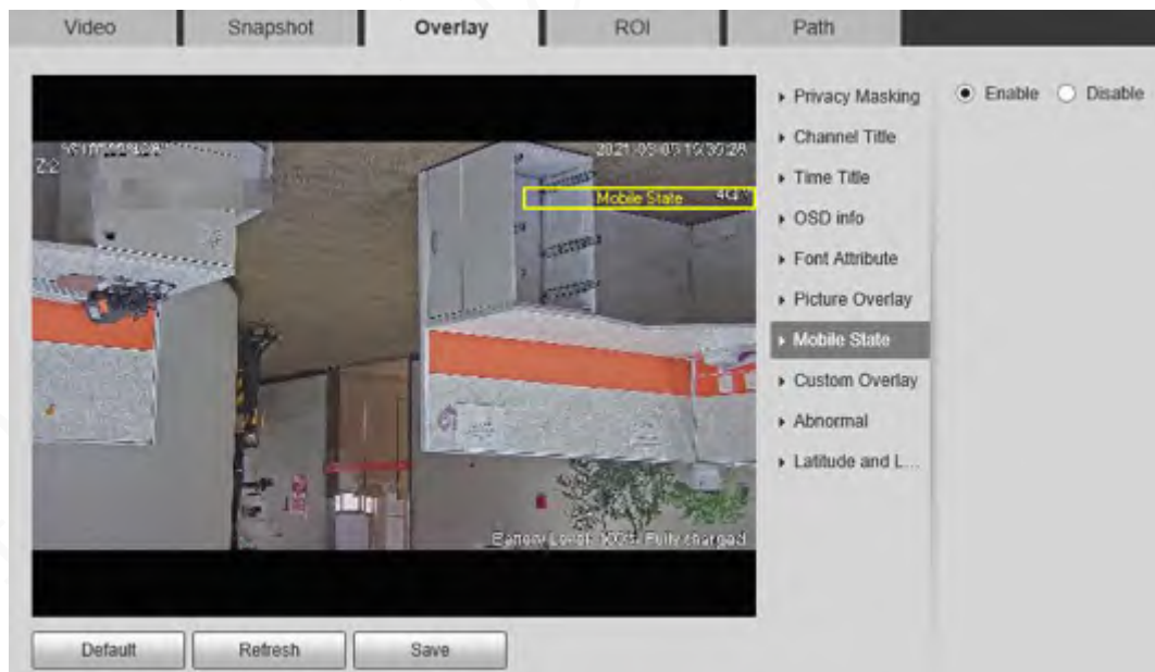
Figure 5-26 Mobile state
