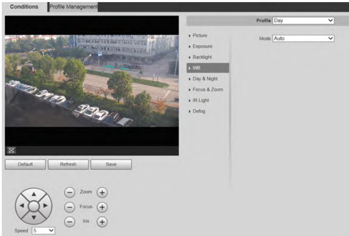
Figure 5-8 WB settings
