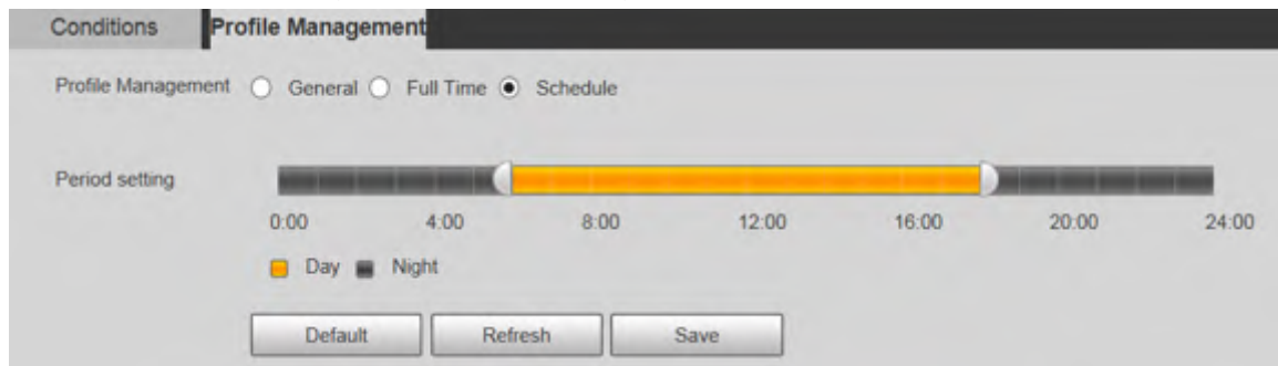
Figure 5-17 Profile management—schedule
