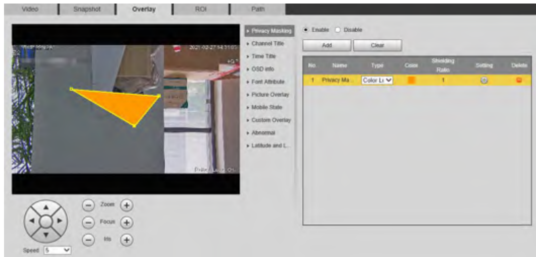
Figure 5-20 Privacy masking
