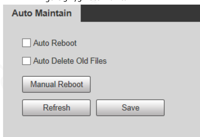
Figure 5-173 Auto maintain
