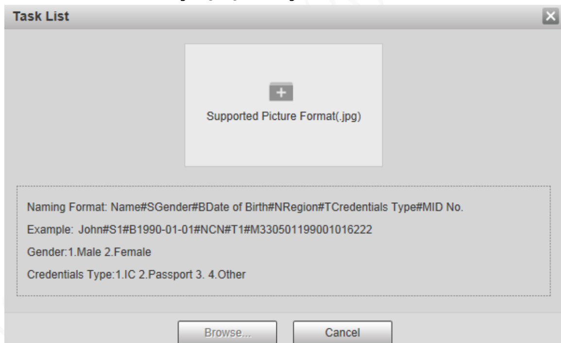
Figure 5-109 Batch registration
