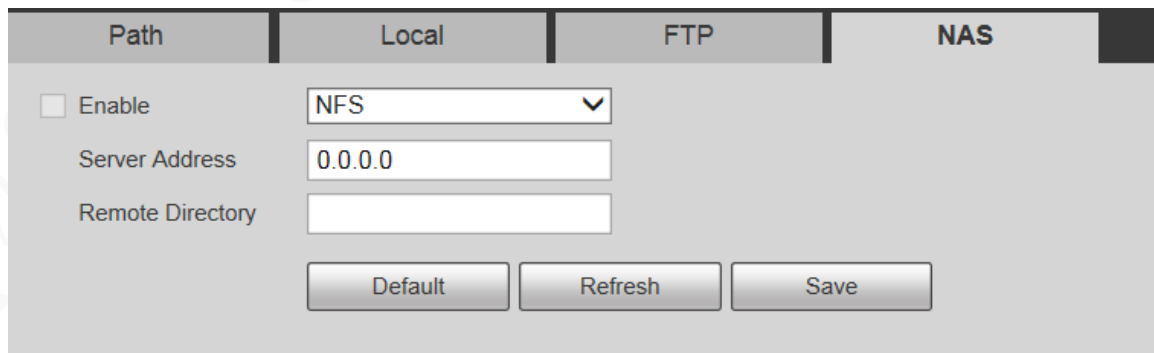
Figure 5-143 NAS settings
