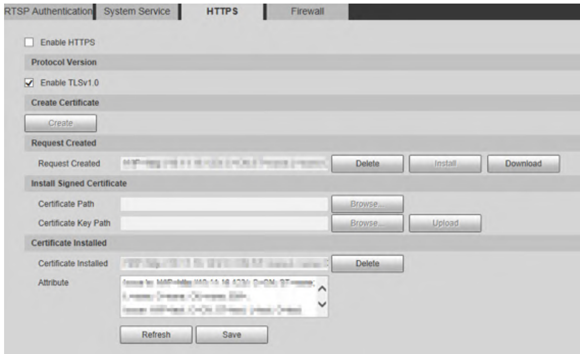
Figure 5-159 Certificate installation
