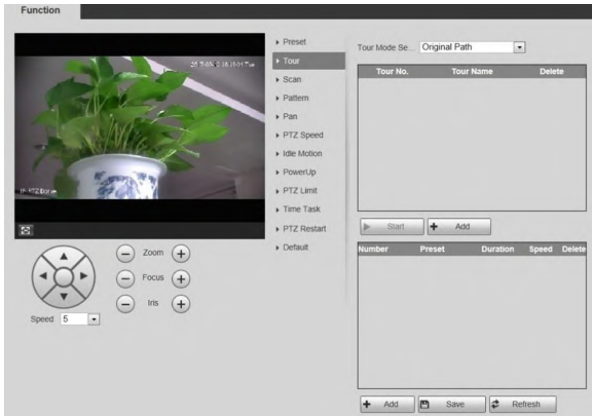
Figure 5-70 Tour settings
