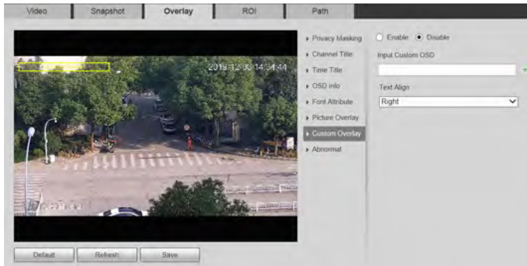
Figure 5-27 Custom overlay
