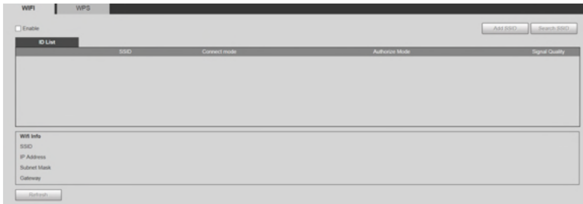
Figure 5-48 Wi-Fi settings (1)
