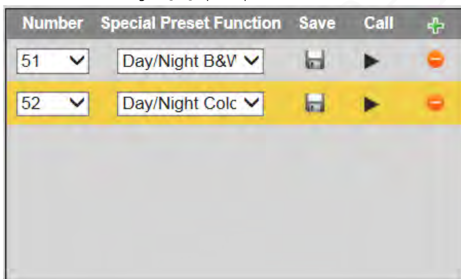
Figure 5-69 Special presets
