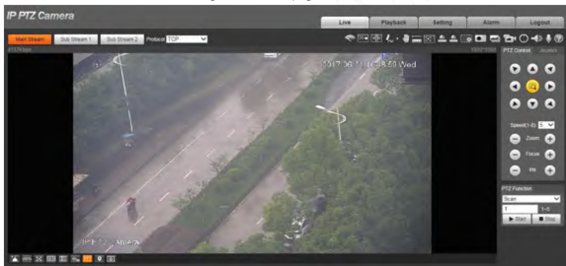
Figure 1-12 Live page
