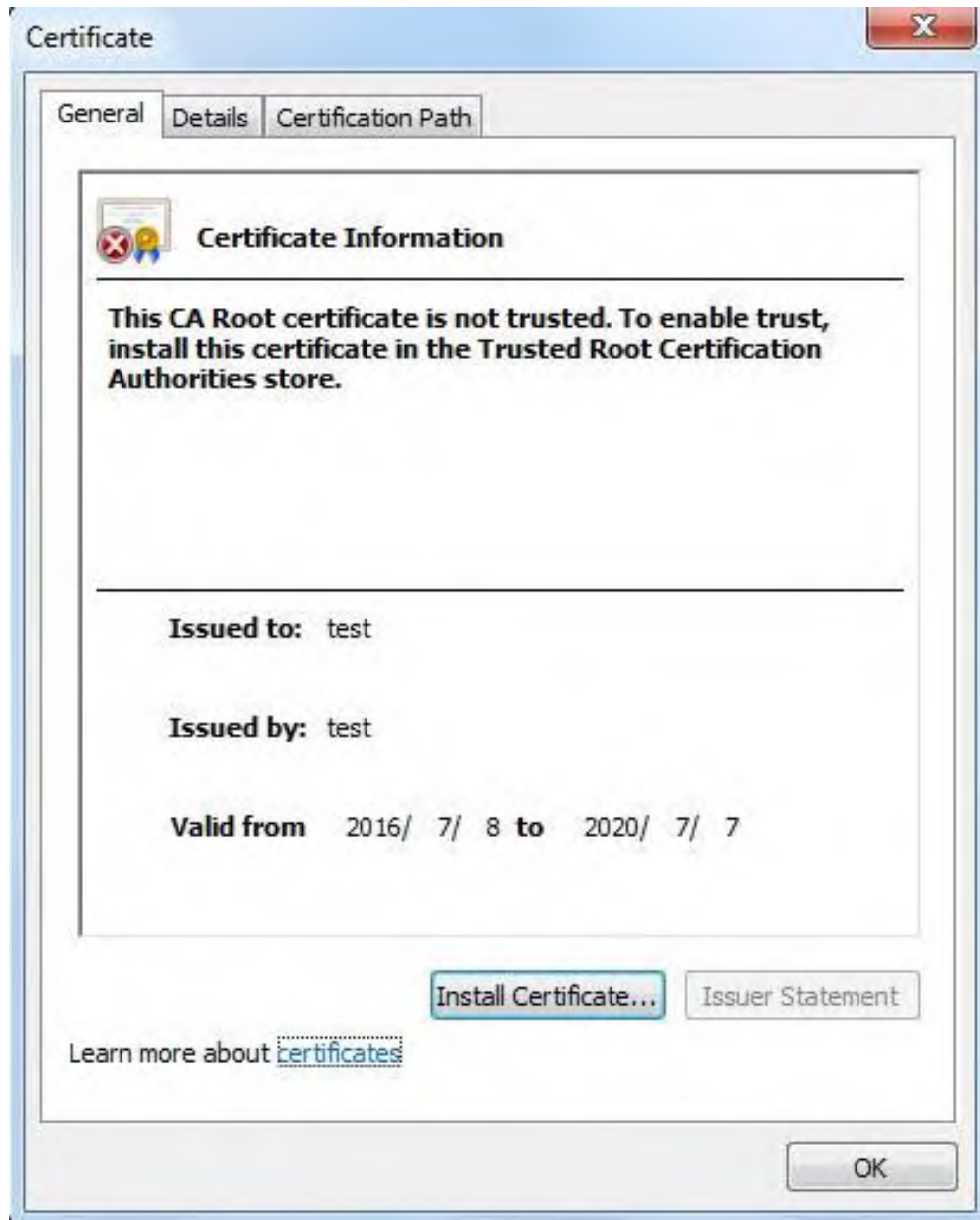
Figure 5-161 Certificate information
