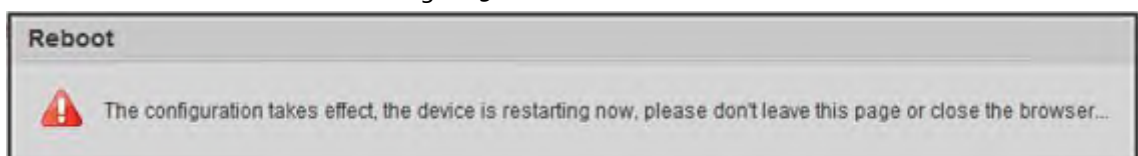
Figure 5-168 Reboot
