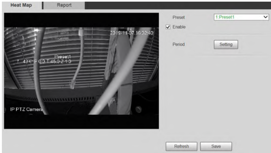
Figure 5-118 Heat map
