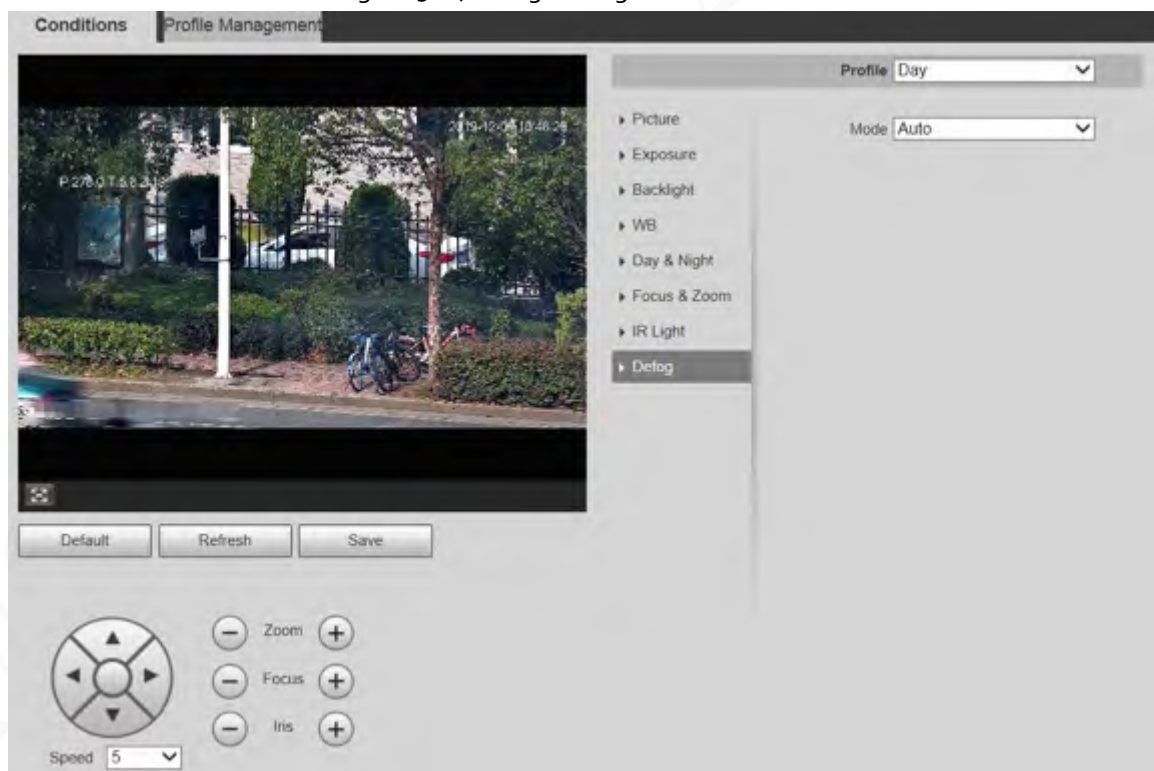
Figure 5-14 Defog settings—auto
