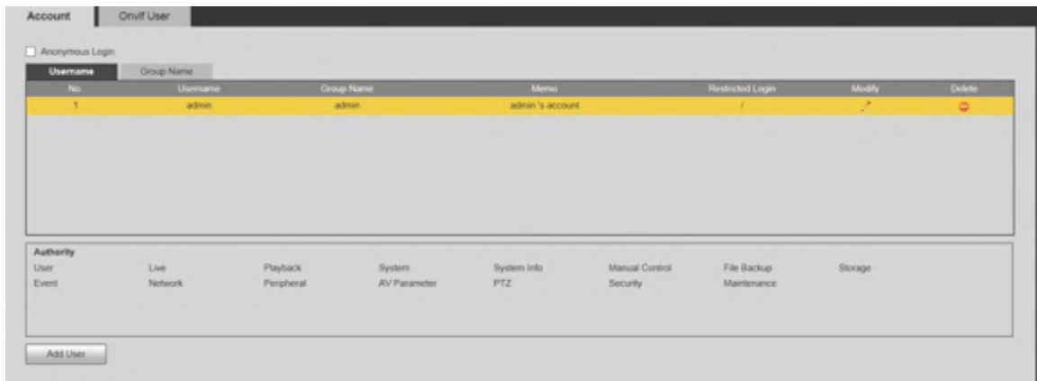
Figure 5-148 Account interface
