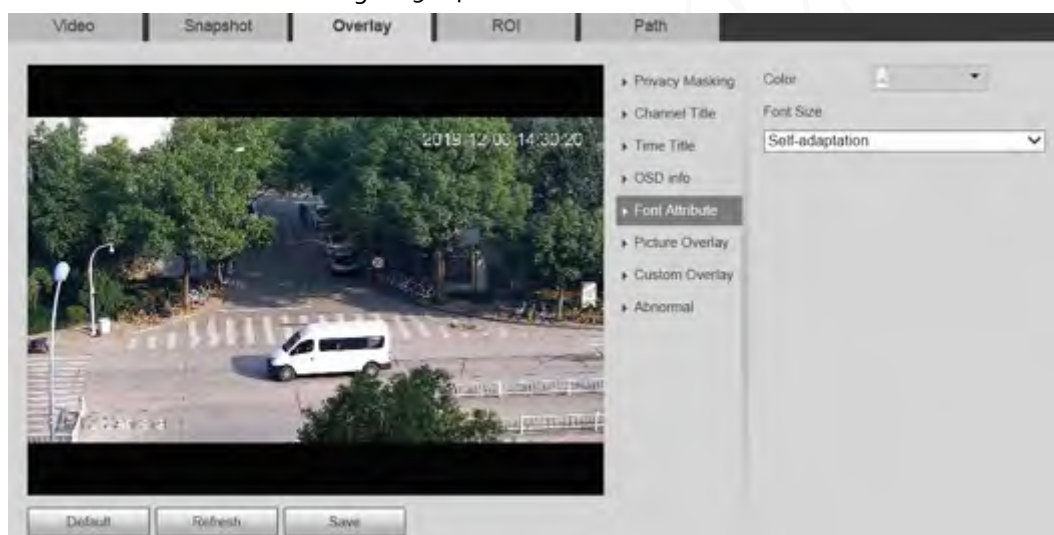
Figure 5-24 Font attribute
