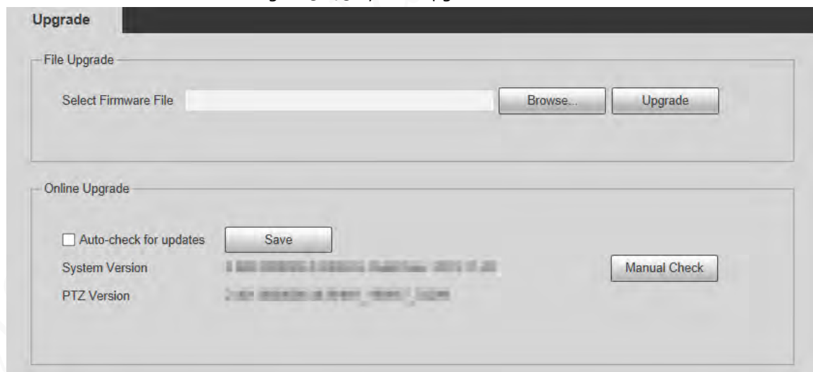
Figure 5-175 System upgrade
