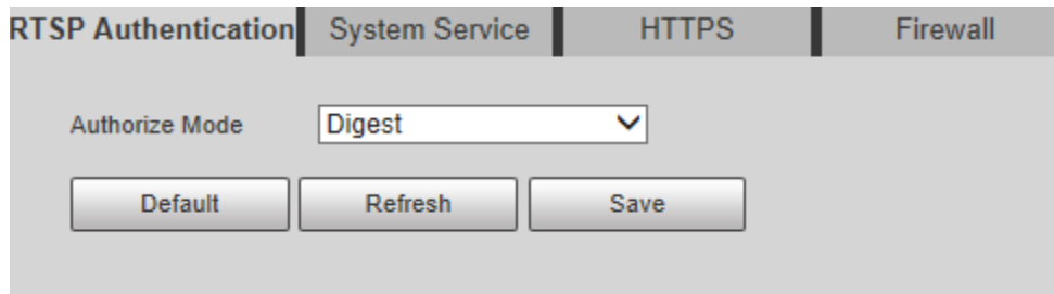
Figure 5-155 RTSP authentication
