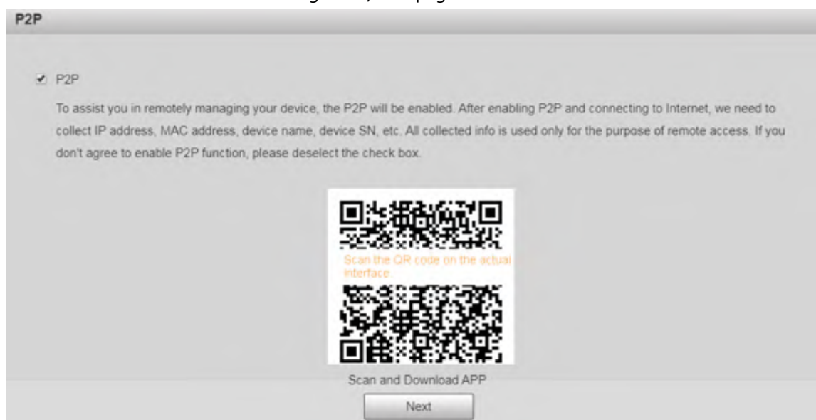
Figure 1-7 P2P page
