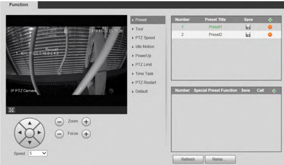
Figure 5-67 Preset
