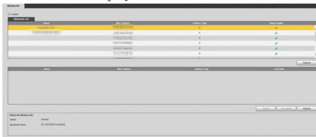
Figure 5-62 Bluetooth list
