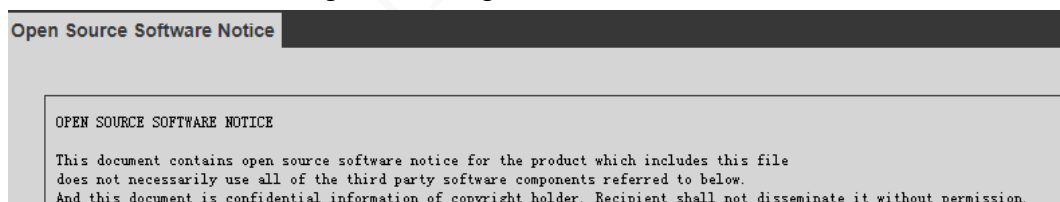
Figure 5-182 Legal information
