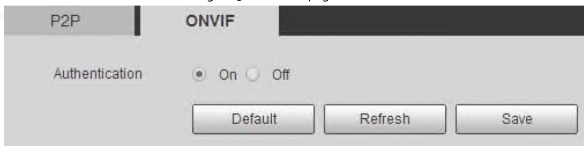
Figure 5-60 ONVIF page
