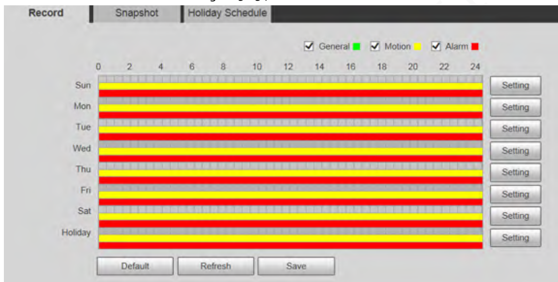
Figure 5-134 Record
