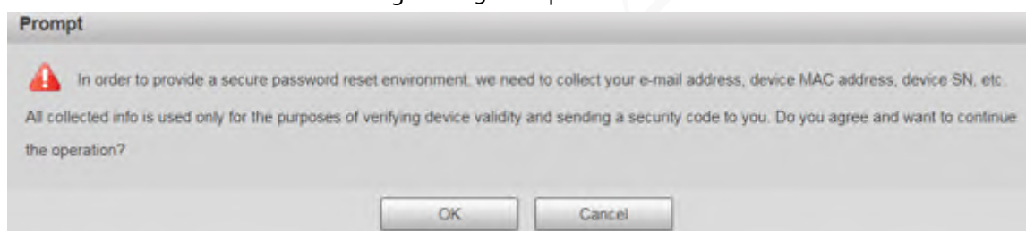
Figure 1-15 Prompt
