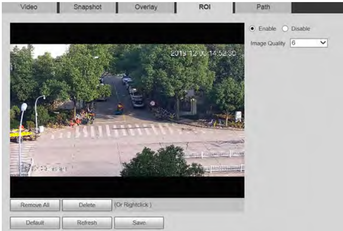
Figure 5-30 ROI settings
