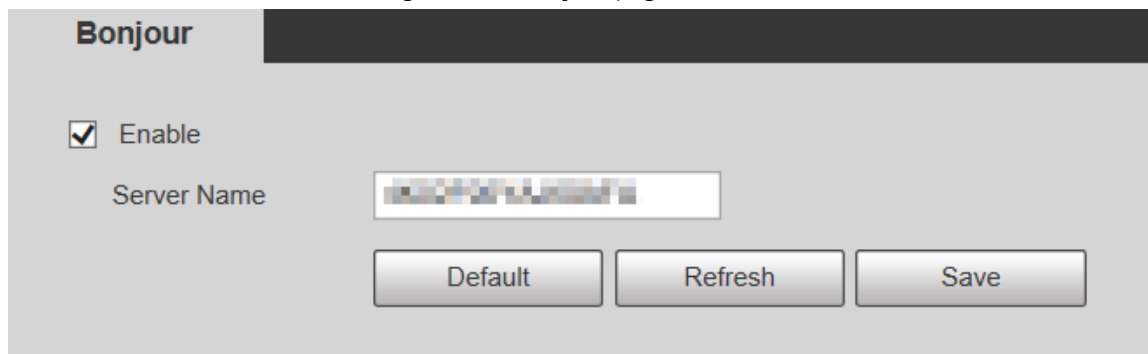
Figure 5-42 Bonjour page
