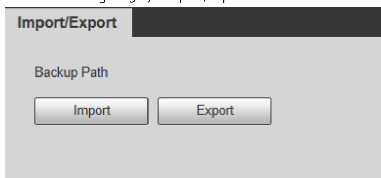
Figure 5-172 Import/Export
