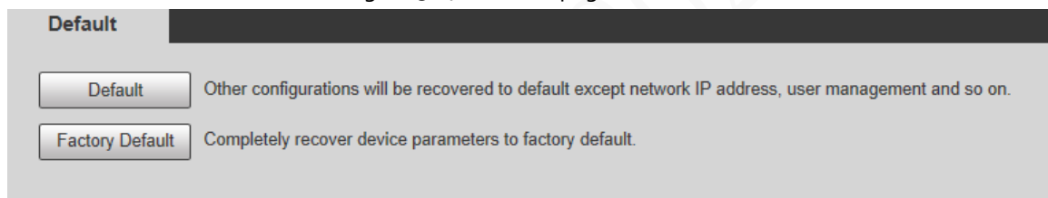
Figure 5-171 Default page
