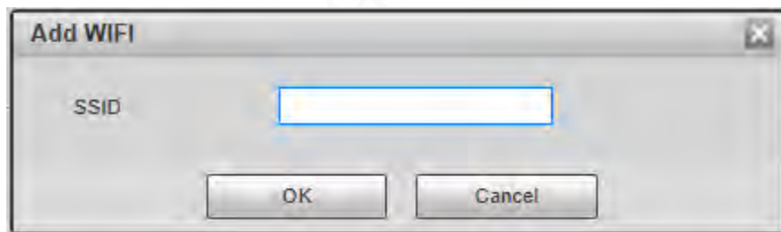
Figure 5-50 Add Wi-Fi
