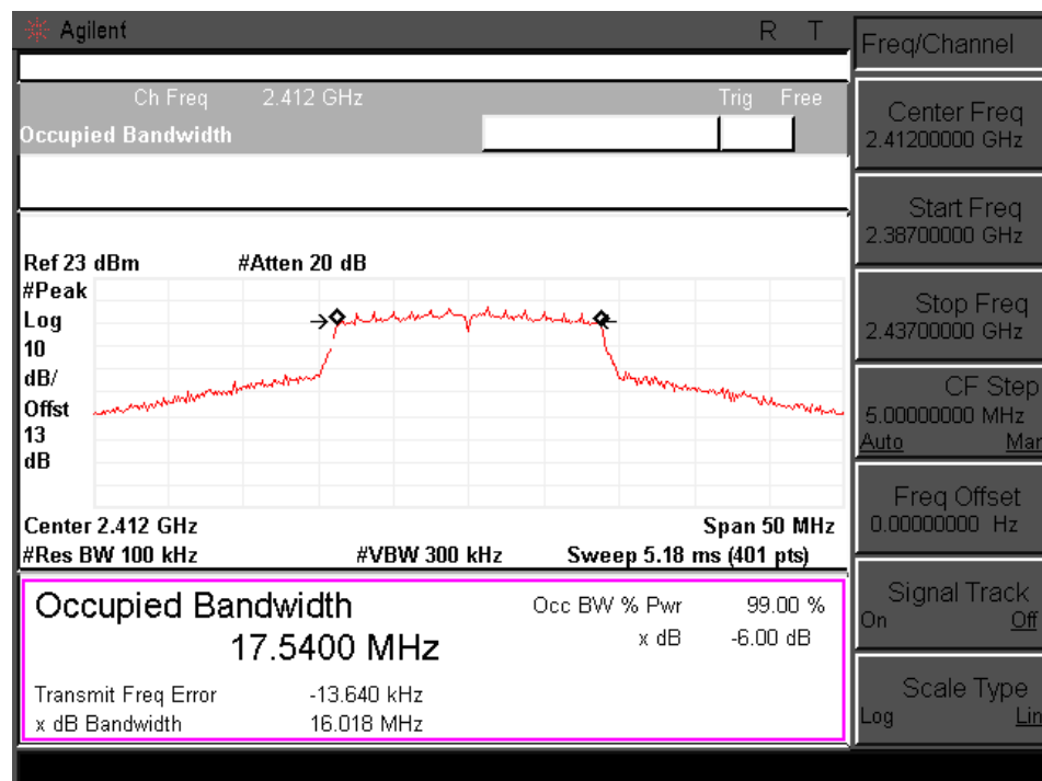
Channel 01 (2412MHz)
