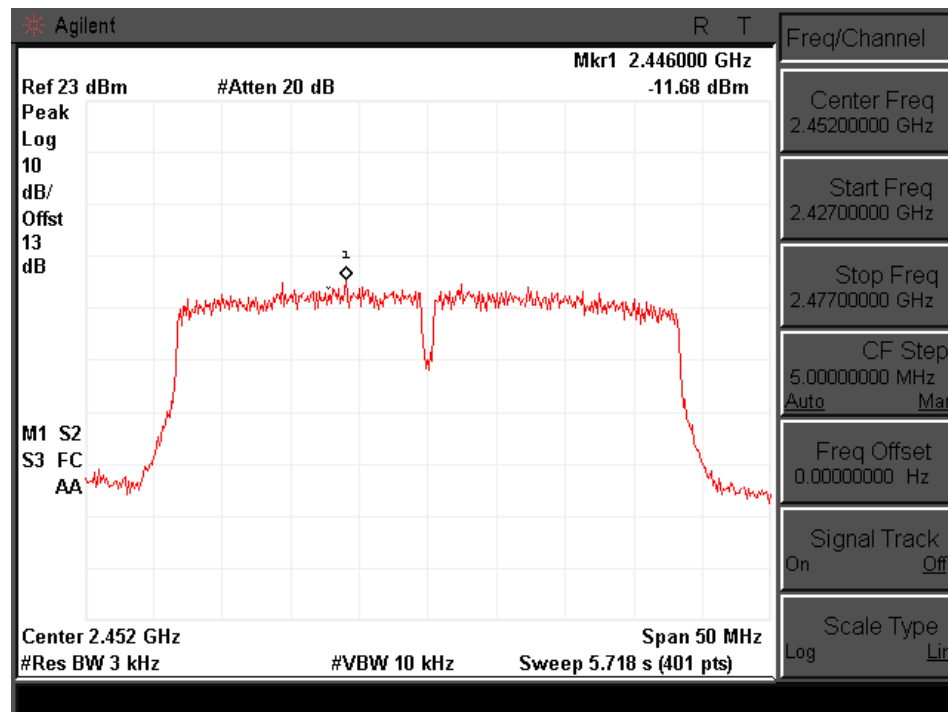
Channel 09 (2452MHz)
