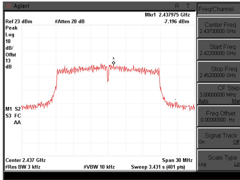
Channel 06 (2437MHz)
