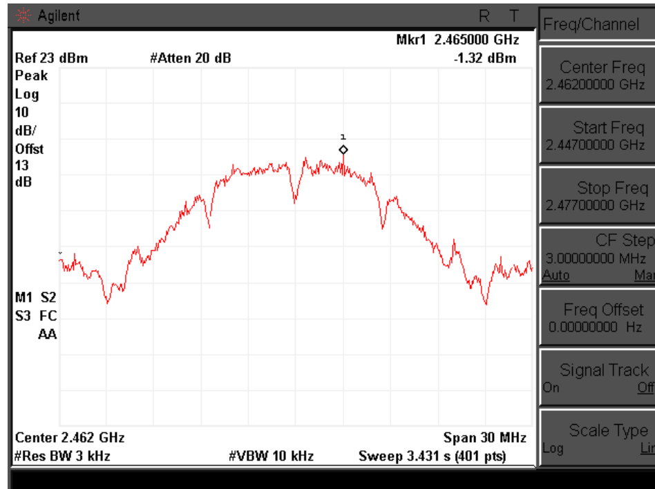
Channel 11 (2462MHz)
