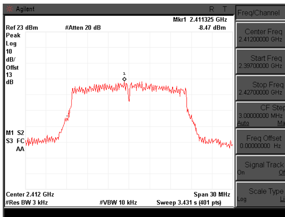
Channel 01 (2412MHz)
