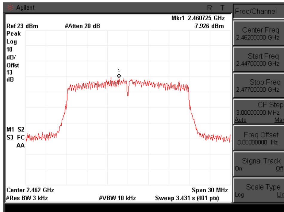
Channel 11 (2462MHz)
