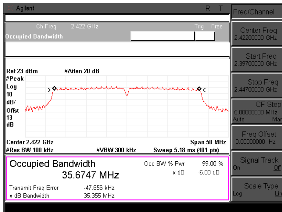
Channel 03 (2422MHz)
