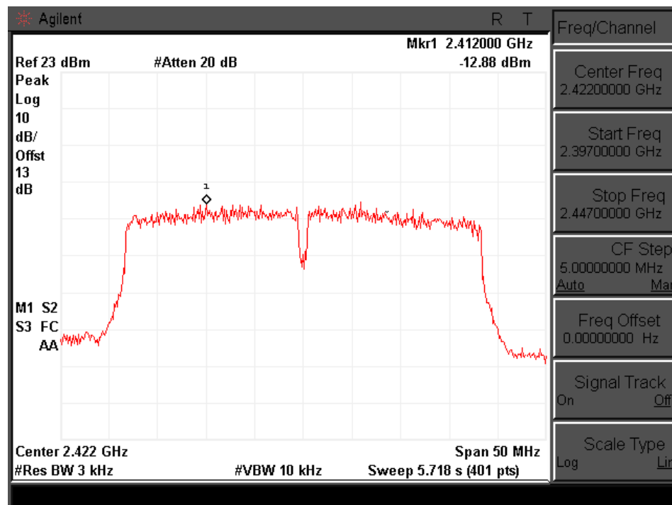
Channel 03 (2422MHz)
