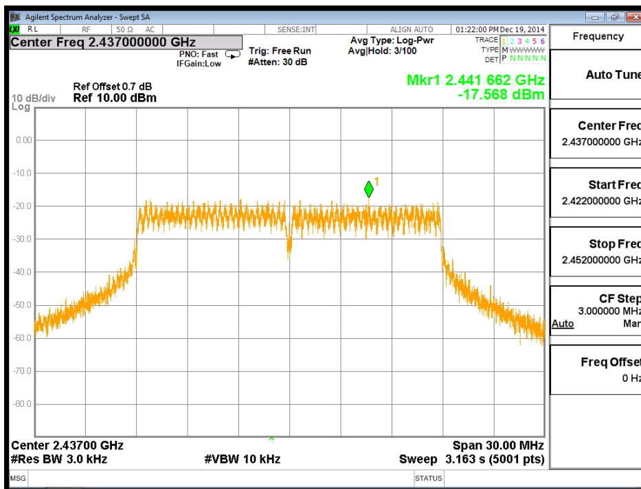
Channel 06 (2437MHz)
