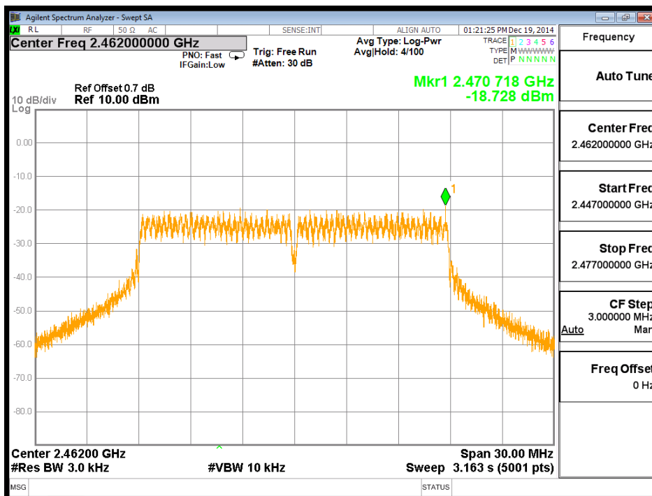
Channel 11 (2462MHz)
