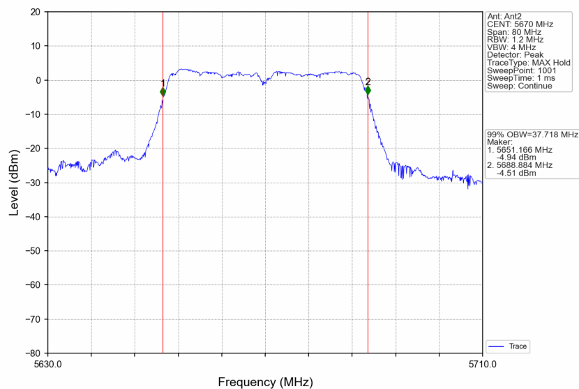
802.11n(HT40)_HCH_5670MHz_Ant2_NTNV
