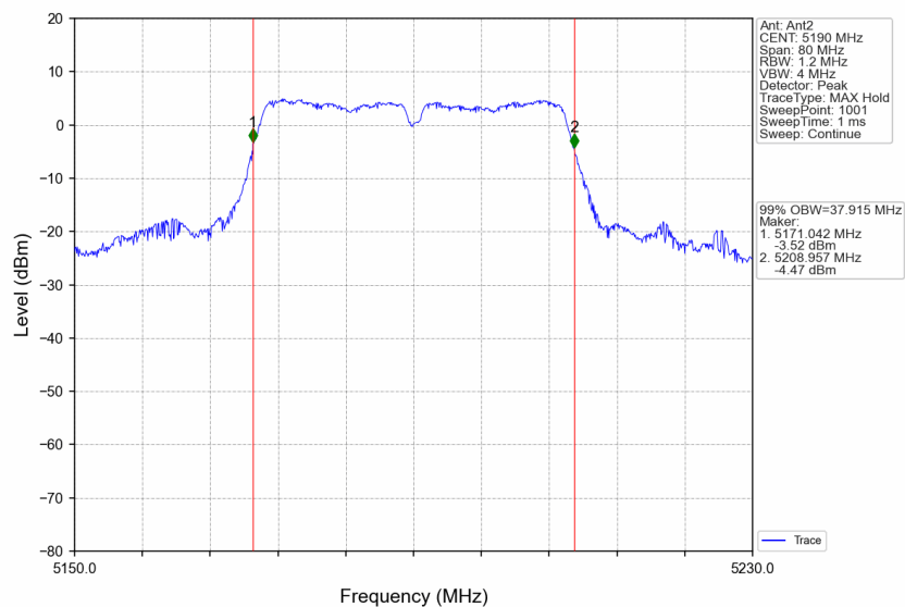
802.11ac(VHT40)_LCH_5190MHz_Ant2_NTNV
