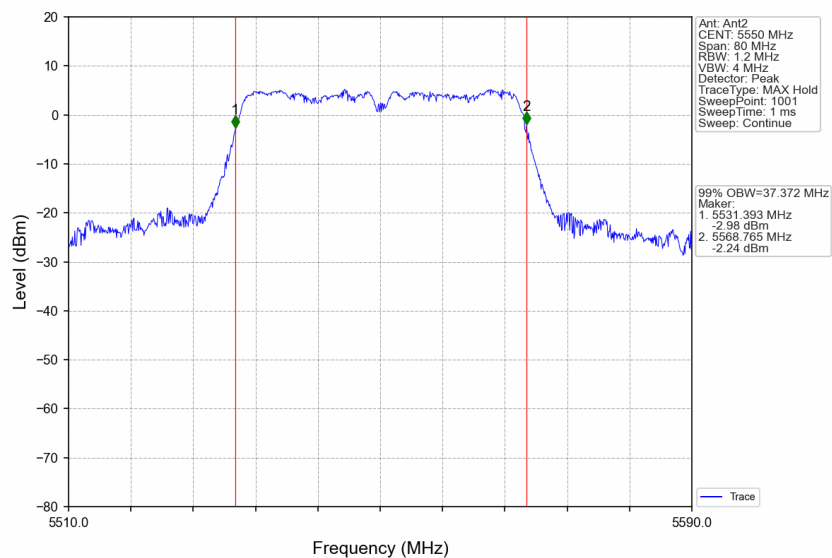
802.11n(HT40)_MCH_5550MHz_Ant2_NTNV
