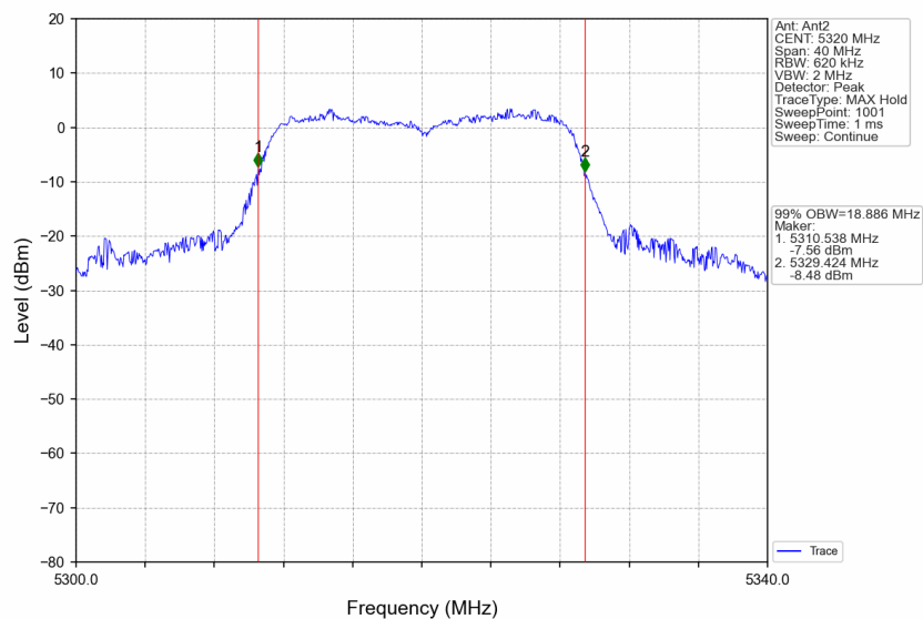
802.11ac(VHT20)_HCH_5320MHz_Ant2_NTNV
