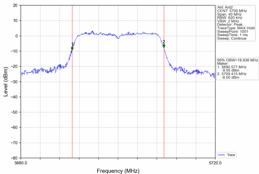
802.11ac(VHT20)_HCH_5700MHz_Ant2_NTNV
