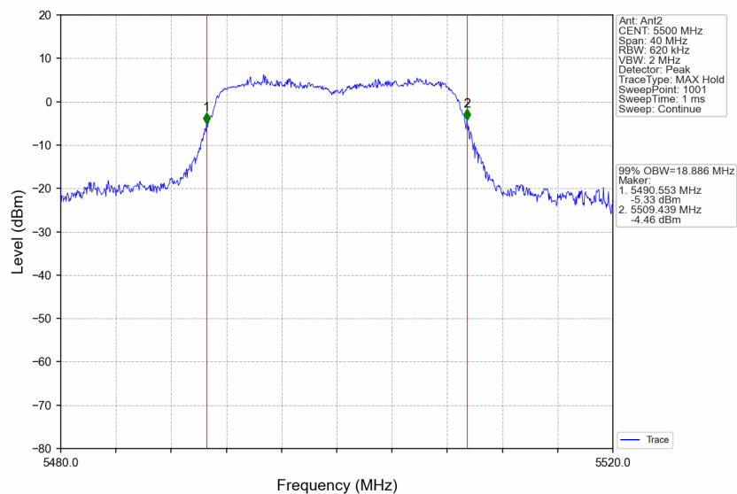
802.11ac(VHT20)_LCH_5500MHz_Ant2_NTNV
