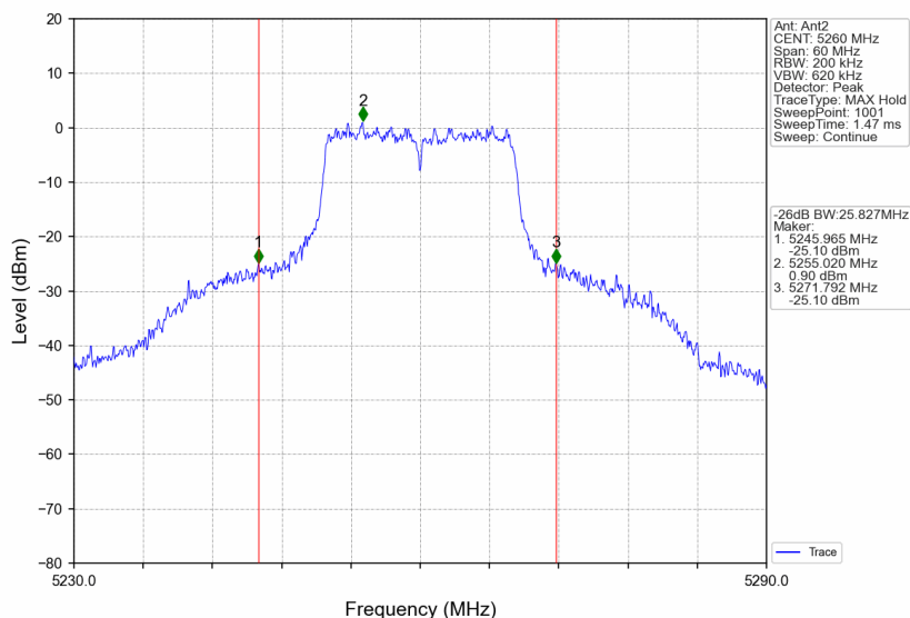
802.11a_LCH_5260MHz_Ant2_NTNV
